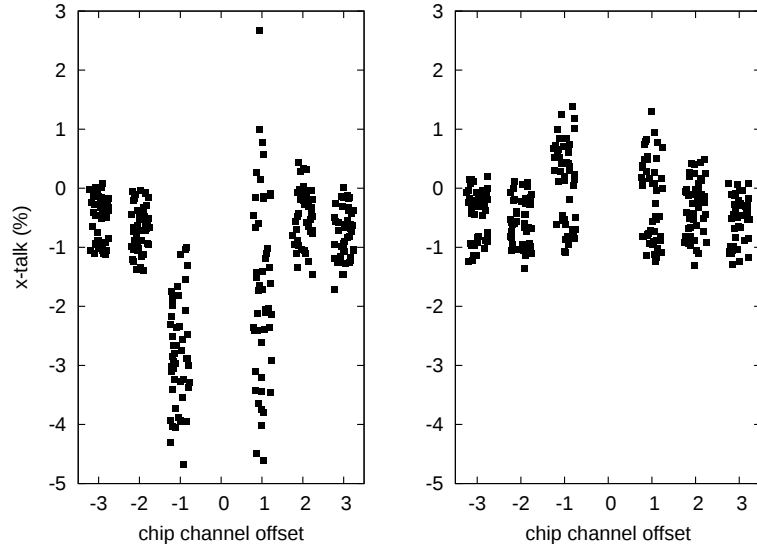
Figure 3.18: Readout cross-talk computed before (left) and after (right) the FIR correction, using ACDC2 data (1 r and 2\phi sensors).
