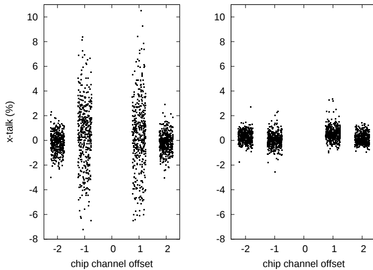
Figure 3.20: Remaining readout cross-talk after a FIR correction per TELL1 board (left) and a per analog cable (right).
