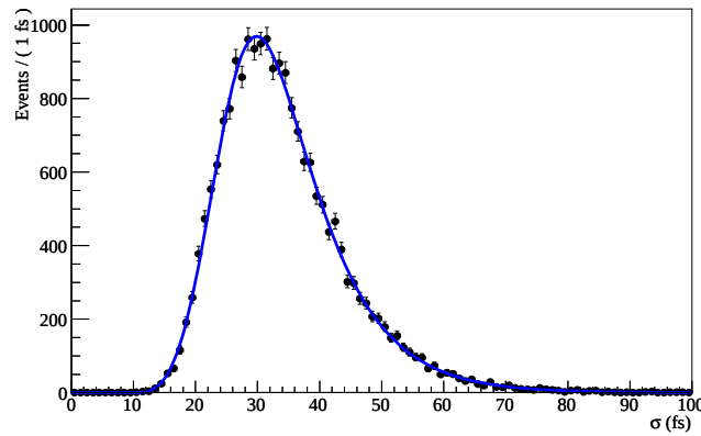
Figure 6.2: Distribution of the error estimates of selected B_s \rightarrow D_s^- \pi^+ events. We show the outcome of the fit performed with the function E .
