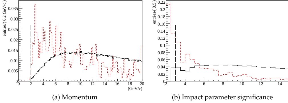
Figure 5.2: Distributions of the different variables for all the particles from the decay (pions and kaons). The red dashed histograms are background events, the black, continuous histograms are signal events. The cut values are shown.
