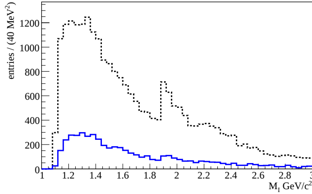
Figure 7.4: Invariant mass distribution for selected secondary interactions. The blue continuous line represents the true secondary interactions. The dashed black line is the full selected statistics.
