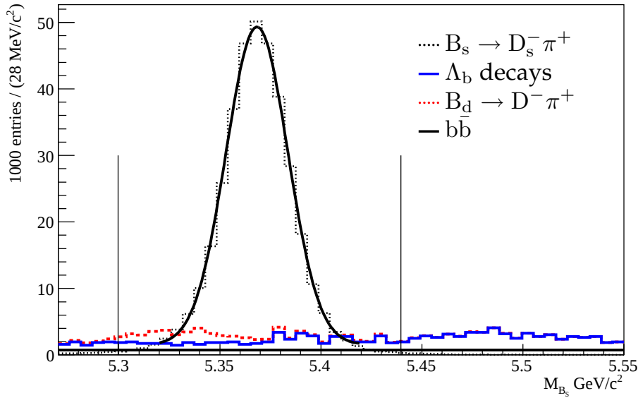
Figure 5.8: Reconstructed B_s with the B_s \rightarrow D_s^- \pi^+ selection. No trigger is applied. The upper limit of the estimated combinatorial b\bar{b} background is represented as a flat distribution (continuous black line). The blue histogram is the reconstructed \Lambda_b \rightarrow D_s^- p and \Lambda_b \rightarrow \Lambda_c^+ \pi^- decays. The dashed red histogram represents the B_d \rightarrow D^- \pi^+ events. All the backgrounds are stacked together. The histograms are normalized to 2 \text{ fb}^{-1} of data.
