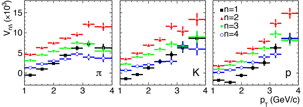
Figure D.1.: V_{n\Delta}(p_T) with n = 1...4 for pions, kaons, and protons. These values are determined using a DCT (see Eq. (C.5)) on the identified yield associated with a high- p_T trigger particle, with the near-side peak removed (see Sect. 6.3).
