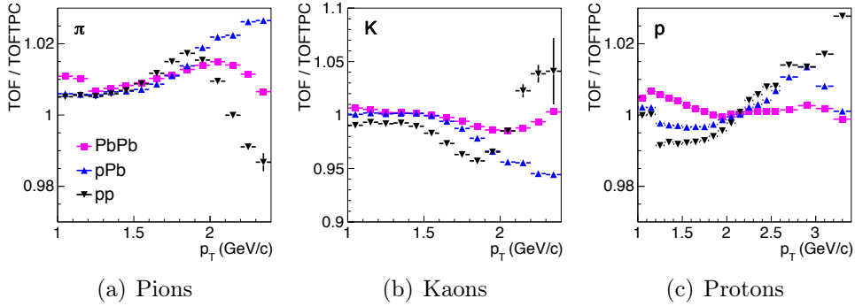
Figure 4.6.: Comparison between the identified yield using a TOF stand-alone fit method and the (TOF, TPC) fit method for pp, p-Pb, and Pb-Pb.
