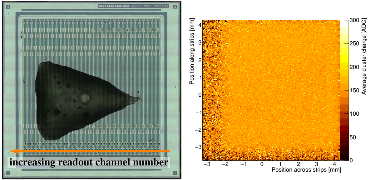
(a) ATLAS07 miniature sensor with Epolite FH-5313 (b) Cluster charge map of miniature sensor with glue
