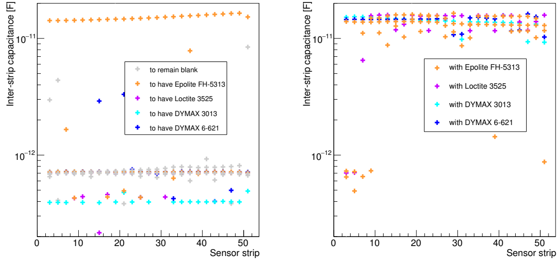
(a) Inter-strip capacitances of FZ1 sensors before gluing (b) Inter-strip-capacitances of FZ1 sensors after gluing
