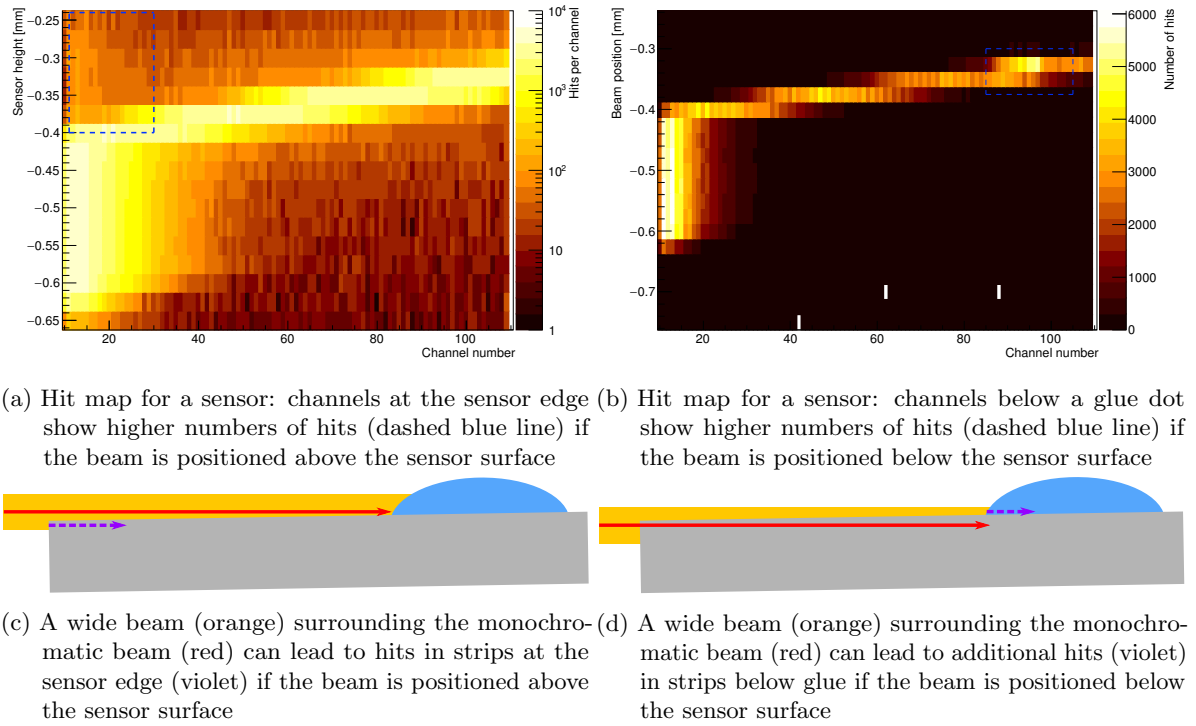
Figure 8.15: Illustration how a wide beam background affects the hit map of a sensor: independent of the beam position, the beam halo leads to additional hits in strips at the sensor edge as well as strips below a glue dot.
