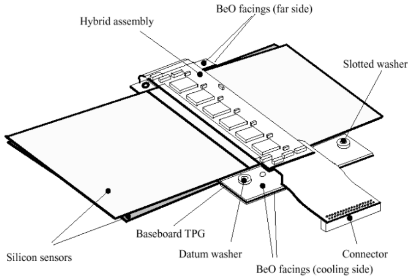
Figure 2.3: Layout of a silicon strip detector module in the Inner Detector (from [34]): silicon sensors are glued on to both sides of a baseboard with an attached heat spreader for cooling. Hybrids with readout chips form bridges over the sensor surfaces.
