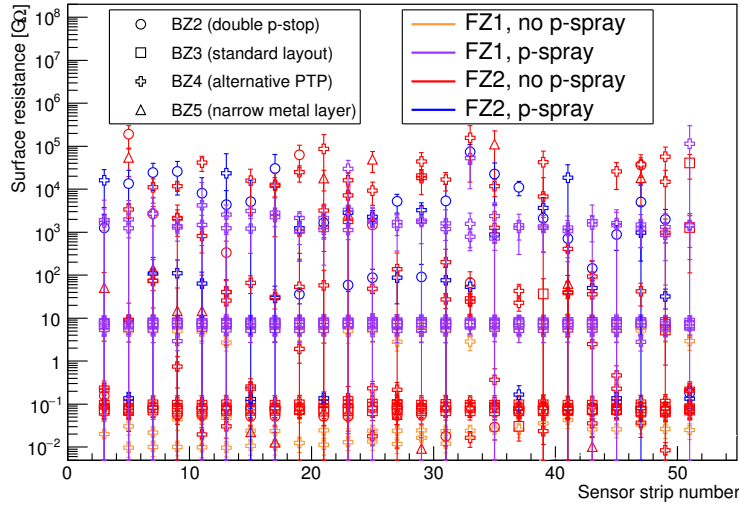
Figure 5.27: Surface resistances measured on 25 strips of ATLAS07 sensors with wafer type (colour) and sensor architecture (marker type) indicated. Surface resistances show a spread over several orders of magnitude. Uncertainties are uncertainties of the linear fit.
