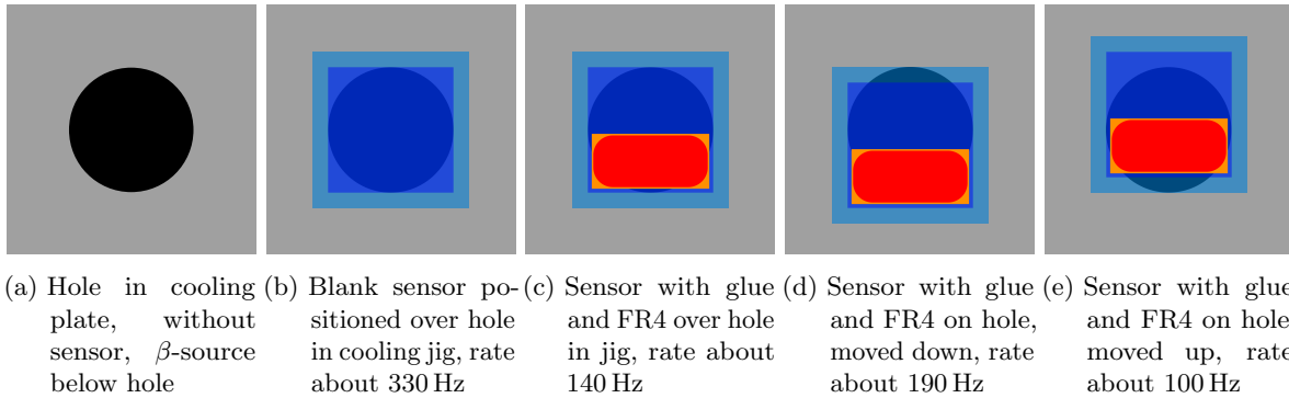
Figure 6.40: Schematic of the possible impact of sensor positions on the data taking rate in a \beta -source setup: when a blank sensor (blue, active area indicated in dark blue) is positioned centred over the \beta -source, a much higher rate can be achieved than for sensors with additional material (glue (red) and FR4 (orange)). This indicates that the additional material blocks a significant fraction of the particles, so that a large fraction of events were collected for sensor areas without glue and FR4.
