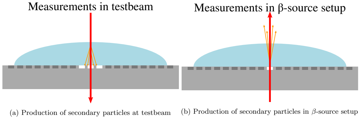
Figure 8.1: Paths of electrons (red) through glue (blue) and sensor (grey) in a testbeam and a \beta -source setup (not to scale). While secondary particles (orange) produced in testbeam tests (left) could theoretically lead to larger clusters, the sensor orientation in the \beta -source setup (right) would not lead to larger cluster sizes caused by secondary particle tracks.
