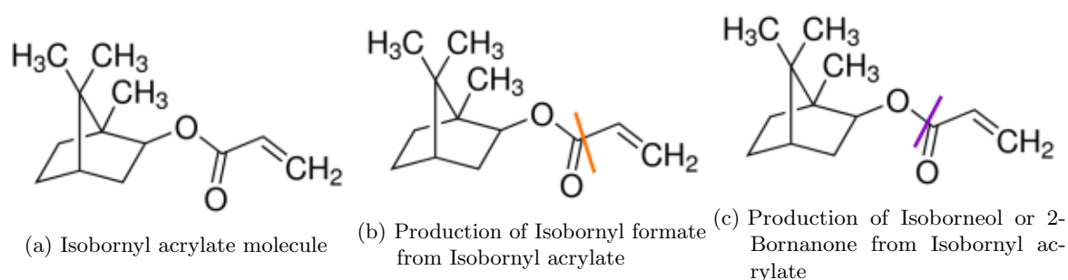
Figure 4.6: Major constituent of DYMAX 6-621 Isobornyl acrylate and possible decay products.
