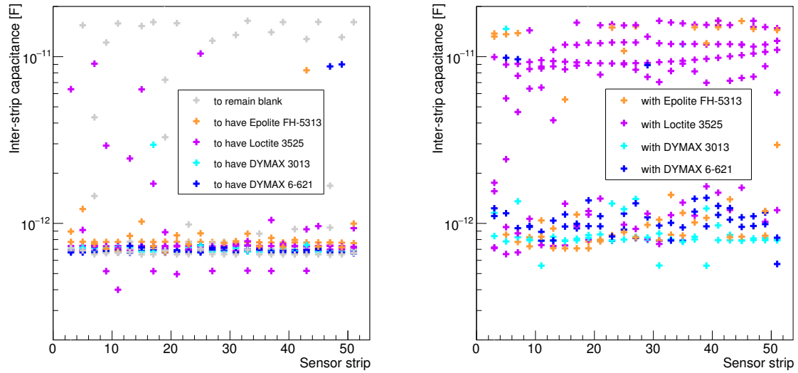
(c) Inter-strip capacitances of FZ2 sensors before gluing (d) Inter-strip capacitances of FZ2 sensors after gluing
