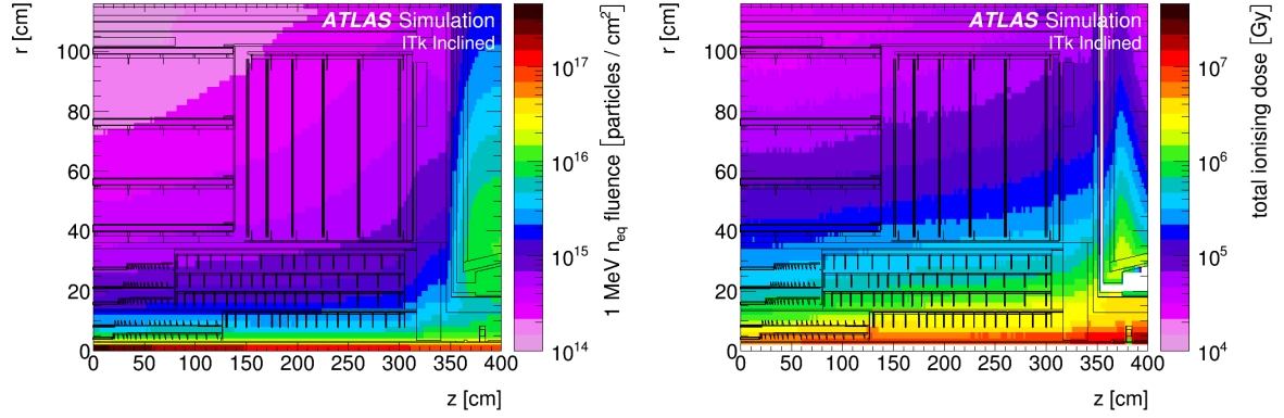
(a) Expected total fluence in the ITk strip tracker, (b) Expected total dose in the ITk strip tracker, from [12]
