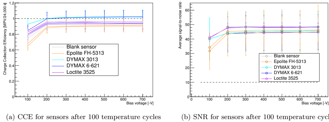
Figure 6.36: CCE and SNR for ATLAS07 sensors (FZ2, narrow strip pitch) with and without glue. CCE for sensors with and without glue are comparable within uncertainties and at or above 90 %. SNR for all sensors agree within uncertainties and are well above the required minimum SNR of 10.
