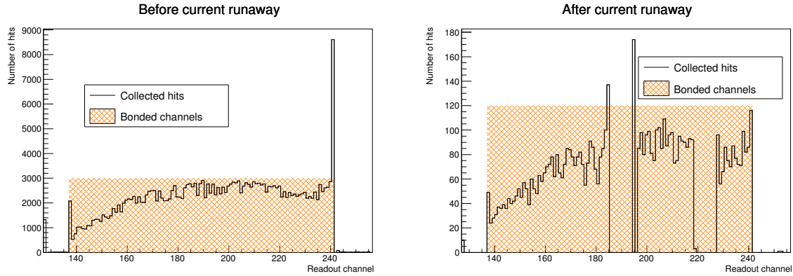
(a) Hit map of a neutron irradiated sensor, operated at -800 V, before current runaway (b) Hit map of a neutron irradiated sensor, operated at -900 V, after current runaway
