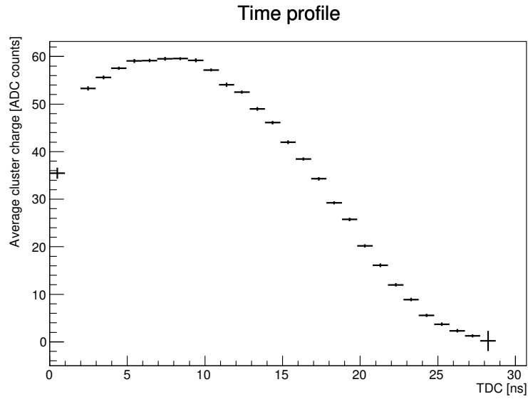
Figure 6.19: Time profile of 500,000 ALiBaVa events produced by averaging the input charge of all events with the same time discrepancy. The charge distribution shows a plateau over five time bins with lower reconstructed charges for both smaller and larger time discrepancies.
