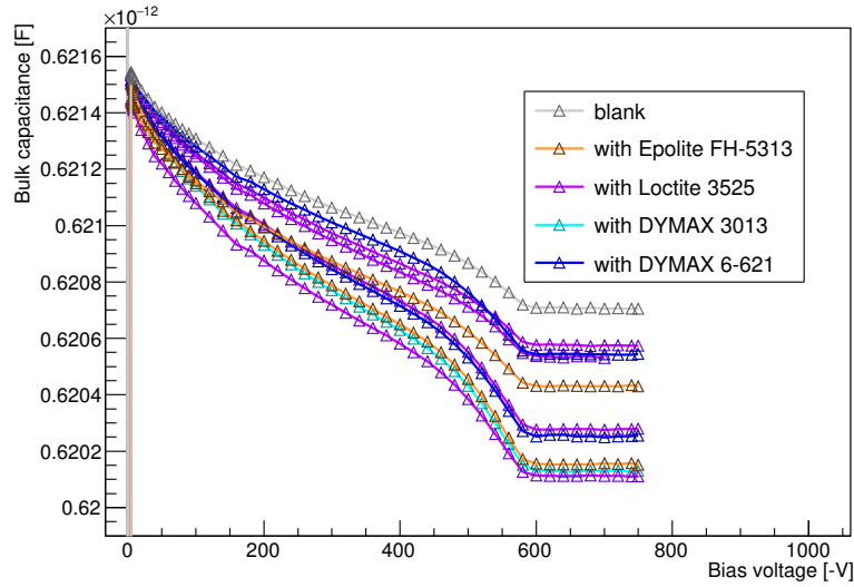
(b) Bulk capacitance measurements of ATLAS07 FZ2 sensors after irradiation with 23 MeV protons
