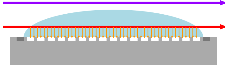
Figure 8.3: conceptual design to investigate signal production by fluorescence: by directing a beam into a glue layer parallel to the sensor surface (red line), fluorescence would produce light along the beam path, of which light reaching the sensor surface could cause sensor strips to register signals (white). This effect would occur only if the beam traverses the glue, not if it is positioned above the glue (violet line).
