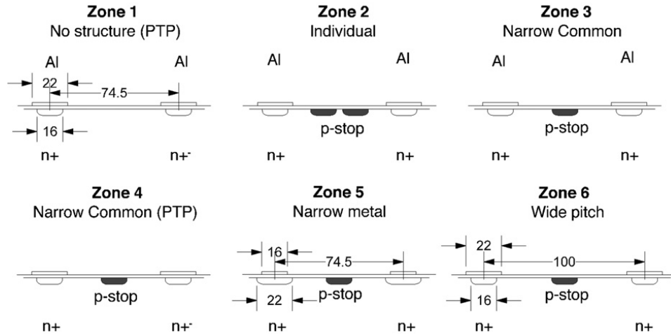
Figure 3.2: Sensor architectures for miniature sensors realised on ATLAS07 silicon sensor wafers. Starting from the standard sensor layout Z3 (strip implants with a width of 16\text{ }\mu\text{m} and a 22\text{ }\mu\text{m} aluminium top layer, arranged at a strip pitch of 74.5\text{ }\mu\text{m} and separated by a single p-stop implant), each of the architectures shows the variation of one aspect. Z1 has no p-stop implants, Z2 double p-stop implants, Z5 has wider strip implants and narrower aluminium top layers, Z6 has a larger strip pitch and Z4A-D have different punch-through protection structures.
