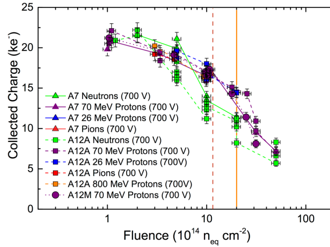
Figure 6.30: CCE measurements of ATLAS07 and ATLAS12 miniature sensors after irradiation with neutrons, protons and pions, from [12]. The orange line indicates the fluence used for the studies presented here.
