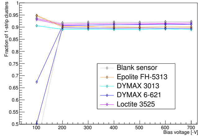
Figure 6.37: Fraction of 1-strip clusters for ATLAS07 sensors (FZ2, narrow strip pitch) with and without glue after 100 temperature cycles. Sensors with and without glue show a similar pattern as sensors after gluing, with blank sensors showing a higher fraction of 1-strip clusters than sensors with glue.
