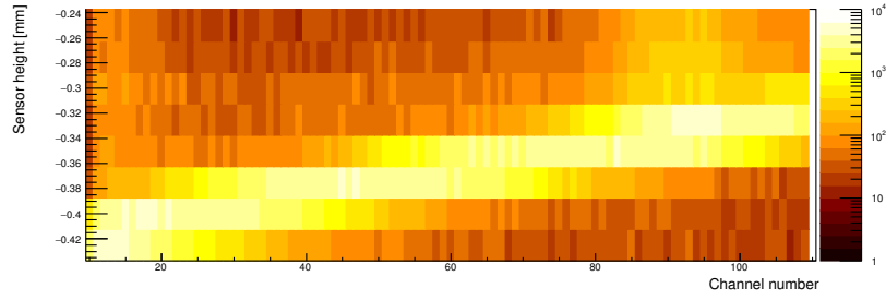
(a) Hit map for first beam position along the sensor strip ( x = -12 mm)
