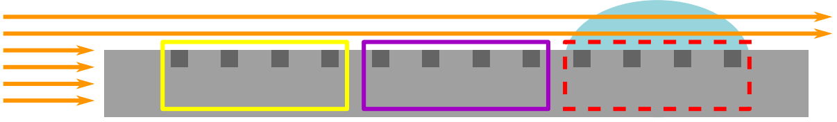
Figure 8.4: Scheme of a fluorescence measurement of a strip sensor with glue (not so scale): a beam is pointed at the sensor perpendicular to sensor strips (dark grey). While strips at the sensor edge (yellow area) are expected to see hits while the beam is pointed at the sensor, photon absorption inside the silicon will prevent strips further away from the sensor edge from registering hits (violet area). Strips beneath glue (red area) are thus expected to see hits only when the beam is pointed at the glue and if fluorescence occurs.
