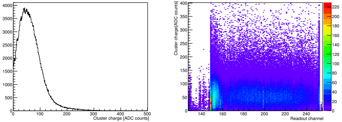
Figure 6.17: Cluster charges reconstructed from 500,000 events collected after clustering for a whole sensor (left) and individual sensor strips (right).
