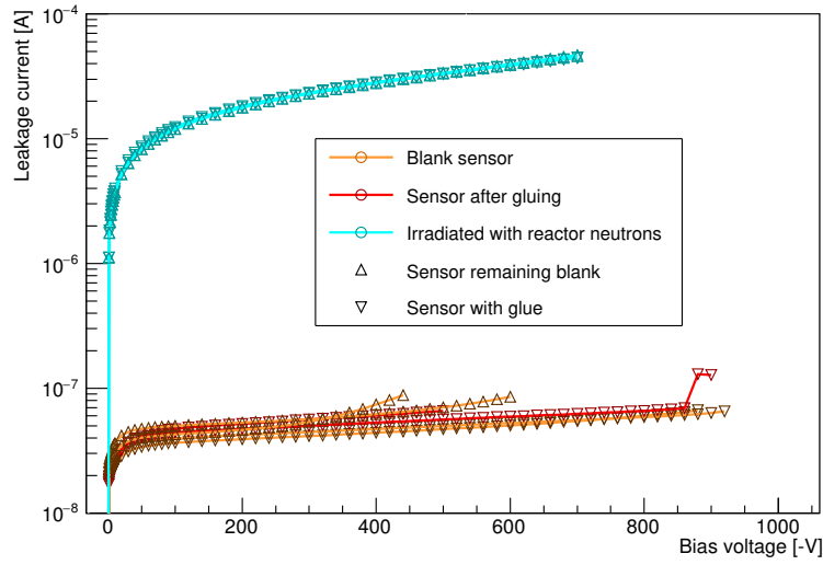
Figure 5.55: Leakage currents of ATLAS07 FZ2 sensors with p-spray after irradiation with reactor neutrons in comparison with leakage currents before and after gluing. Leakage currents of sensors with and without glue did not show any discrepancies after irradiation with reactor neutrons.
