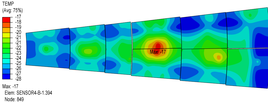
Figure 2.6: FEA temperature simulation of a petal in the strip tracker after 3000 \text{ fb}^{-1} , from [12]. Due to the position of the power board on Ring 3 between cooling tubes, its bPOL12V chip is expected to become the the hottest area on the petal, leading to a temperate difference of 10^\circ\text{C} on R3 modules.
