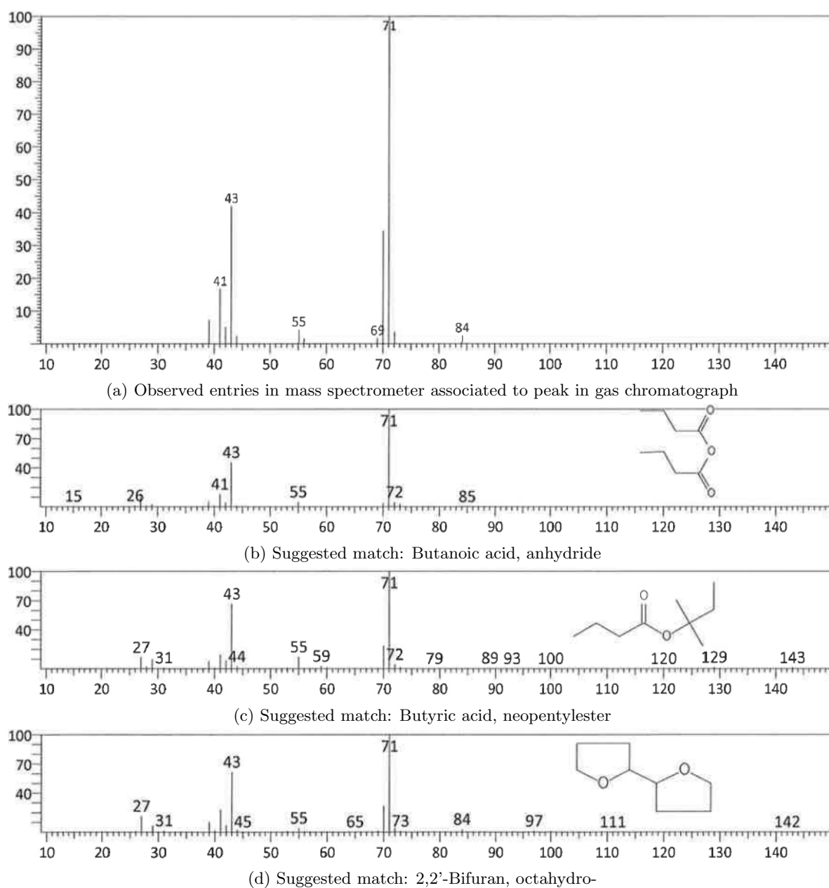
Figure 4.8: Mass spectrometer entries associated with peak at retention time 13.78 min in gas chromatography spectrum of DYMAX 3013, irradiated with 800 MeV protons up to 1 \cdot 10^{15} \text{ n}_{\text{eq}}/\text{cm}^2 and suggested matches from database. All pictures from Infrapark chemical analysis report.
