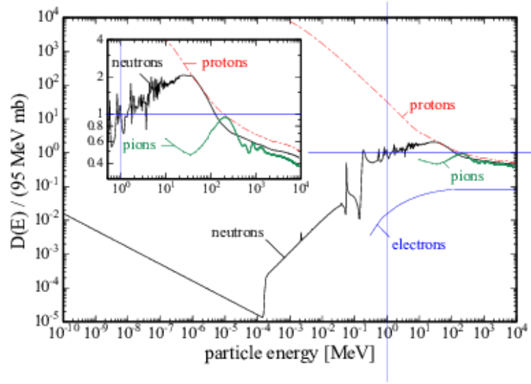
Figure 3.5: Displacement damages for different particles relative to the neutron equivalent fluence \Phi_{eq} [54]
