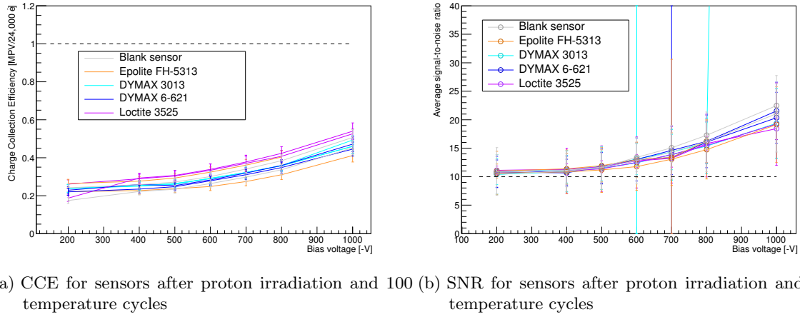
Figure 6.38: CCE and SNR for ATLAS07 sensors (FZ1, narrow strip pitch) with and without glue after proton irradiation and temperature cycling. CCE and SNR are comparable within uncertainties for sensors with and without glue.
