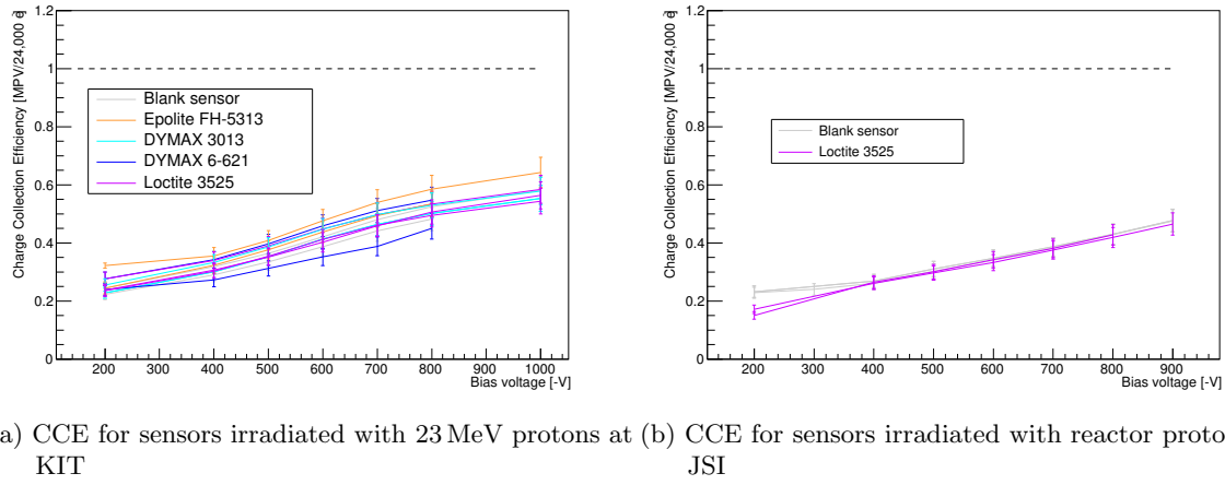
Figure 6.29: CCE for irradiated ATLAS07 miniature sensors (FZ2, narrow pitch) with and without glue. CCEs show variations for different sensors, but no systematic differences between sensors with and without glue or individual glues. CCE at -1000 V could only be measured for sensors with sufficiently low leakage current (see section 6.7.3.1).
