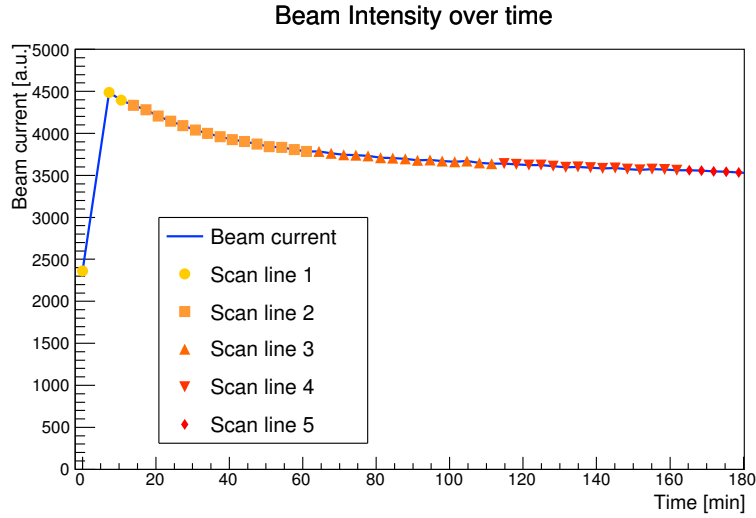
Figure 9.14: Synchrotron beam line current measured after a restart as a function of time. Markers represent one beam position of the scan grid, with one scan line consisting of 15 scan points across the sensor strips.
