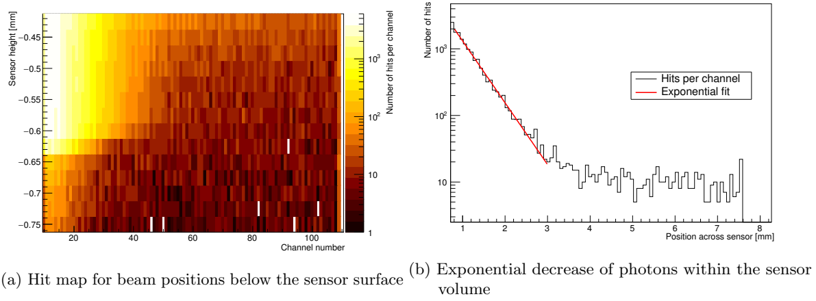
Figure 8.11: Hits registered within the sensor volume from a beam pointing at the sensor edge. The hit map (left) shows hits within the depleted sensor volume, with a lower hit rate in the undepleted sensor volume. For a given beam position, an exponential decay of photons within silicon leads to a corresponding exponential decrease of registered hits (right).
