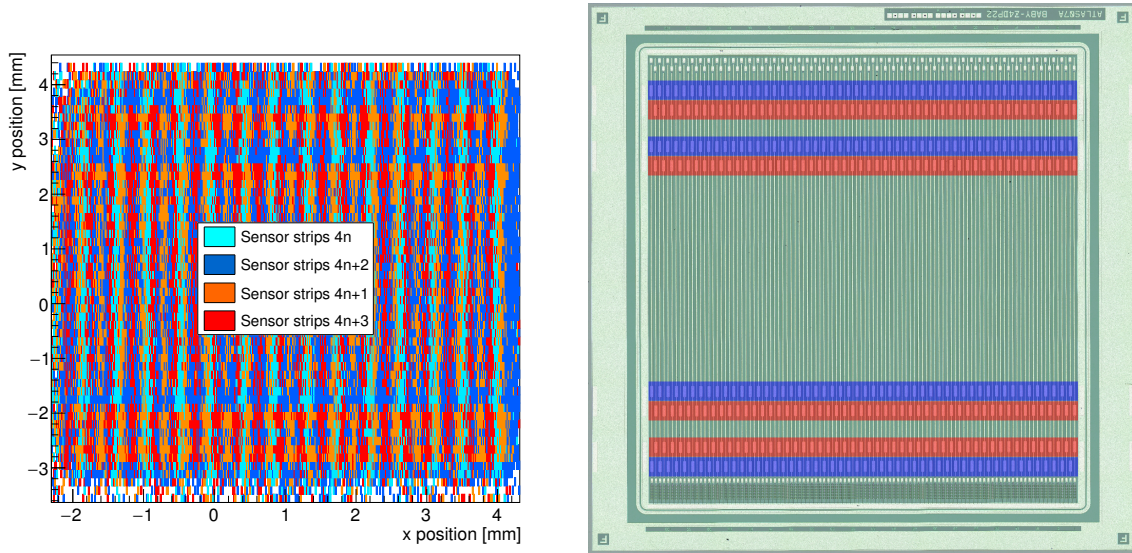
(a) ATLAS07 miniature sensor map showing the mainly responding sensor for a given position on the sensor: orange and red bins represent odd numbered channels, cyan and blue bins represent even numbered channels. (b) ATLAS07 miniature sensor in the same orientation as used in the testbeam. Bond pads of odd and even numbered channels are coloured red and blue, with a total of eight rows of bond pads on the miniature sensor.
