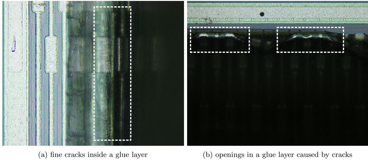
Figure 3.8: Cracks inside DYMAX 3013 glue layers on sensors after temperature cycling (left) and temperature cycling after irradiation (right).
