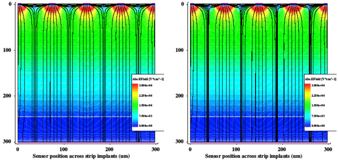
(a) Simulation of the standard sensor layout with (b) Simulation of the sensor layout with altered p-stop equidistant p-stop positions
