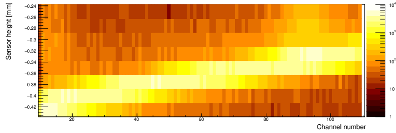
(b) Hit map for second beam position along the sensor strip ( x = -11.8 mm)
