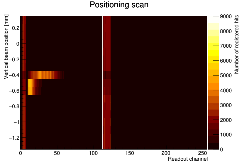
Figure 8.9: Hit map recorded in positioning scan for fluorescence measurements: the first bonded channels (beginning at channel 10) show hits for beam positions -0.6\text{ mm} and -0.5\text{ mm} , showing the expected decrease towards higher channel numbers. At a beam position of -0.4\text{ mm} the beam points at the sensor surface, leading to hits being registered in about 50 readout channels. Unbonded channels next to bonded channels have a high noise, leading to hits being registered over the full scan range (e.g. channels around 120).
