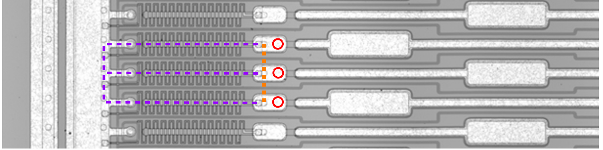
Figure 5.16: Measurement of the inter-strip resistance: if the inter-strip resistance is much higher than the bias resistance, the current measured on DC pads (red circles) goes through the bias resistor (violet lines) instead of the silicon bulk (orange line).
