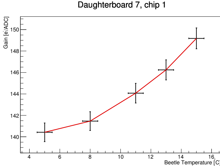
Figure 6.9: Gain of an ALiBaVa beetle chip using measured MPV for a fully depleted ATLAS07 sensor at different temperatures.
