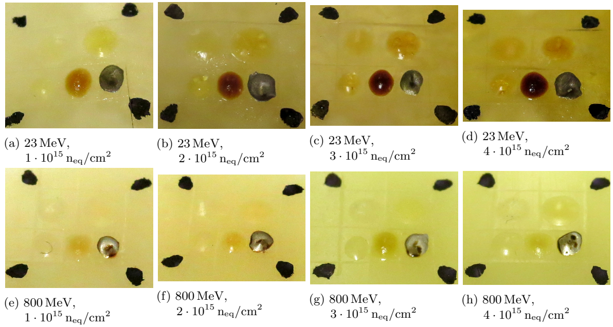
Figure 4.2: Glue samples on polyethylene after irradiations with 23 and 800 MeV up to different fluences. All UV glues samples, initially transparent, show colour changes with increasing fluences, with Epolite FH-5313 (bottom middle) showing the darkest colour after irradiation. Colour changes in samples irradiated with 23 MeV protons show much more significant colour changes than samples irradiated with 800 MeV protons.
