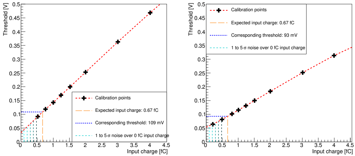
(a) Vt50 threshold depending on input charge, measured for end-cap module (b) Vt50 threshold depending on input charge, measured for barrel module
