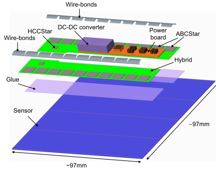
Figure 2.4: Layout of a silicon strip detector module for the Inner Tracker (from [12]): A module consists only of a sensor and the electronics required to read it out, which are glued directly on to the sensor.
