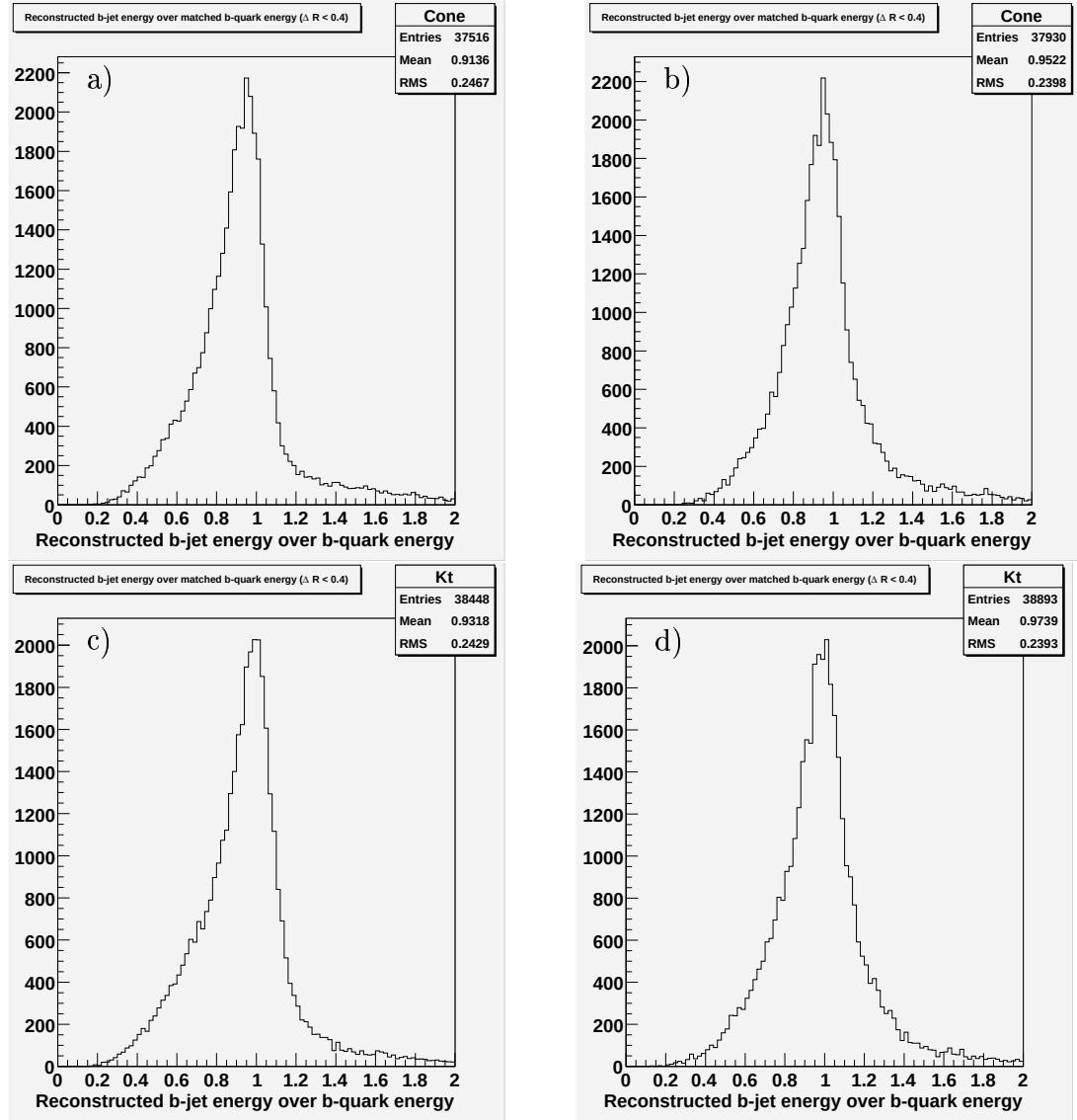
Figure 6.14: Energy resolution of reconstructed b-jets over b-quarks from the hard process, having been matched in a \Delta R cone of 0.4. The left hand side shows the raw jets, while the right shows those with muons added to improve the resolution.
