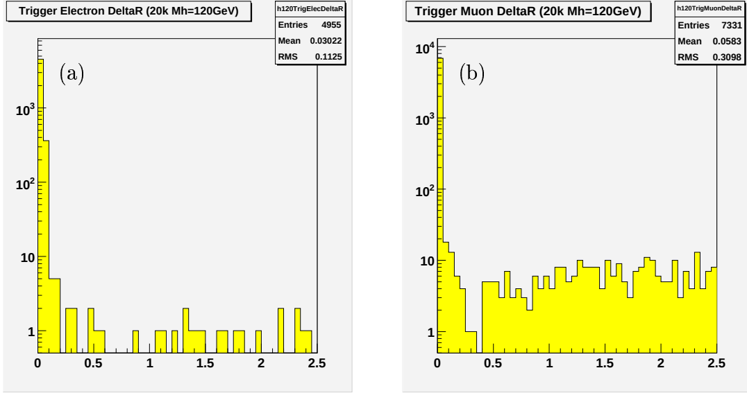
Figure 6.7: \Delta R between the high p_T lepton trigger candidate and the true lepton in 20k\ t\bar{t}H, H \rightarrow b\bar{b} events. The left-hand side shows electrons and the right-hand side muons, with both plots having a logarithmic scale.
