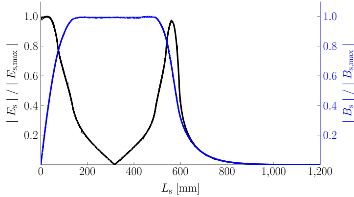
Figure 4.7: The normalized electric and magnetic field over the surface of the end cell. L_s is the contour length on the surface of the cavity.
