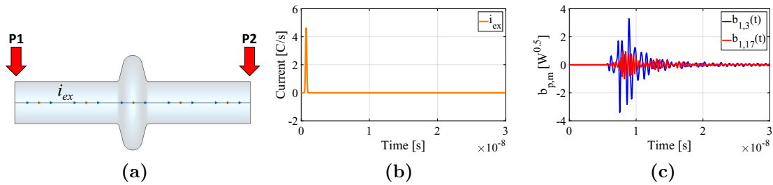
Figure 6.3: A single-cell cavity with two waveguide ports (a), excited by a particle beam with the bunch length of 25 mm and the bunch charge of 1 nC (b). Two signals excited into mode 3 and 17 of port 1 are depicted in (c).
