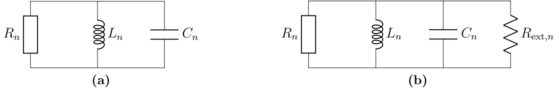
Figure 5.1: The cavity near a resonance mode can be described by a parallel RLC circuit. The HOM coupler adds an extra mean of loss to the HOMs ( R_{\text{ext},n} ).
