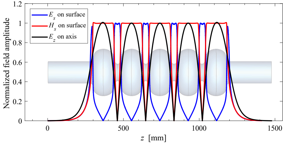
Figure 4.9: Five-cell cavity with the FM frequency at 801.58 MHz. The magnitude of the fields is normalized in each case.
