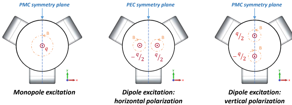
Figure 6.1: Monopole and dipole excitation schemes in 3D wakefield solvers [140]. If the cavity is symmetric with respect to a symmetry plane (indicated by the blue vertical dashed lines), appropriate boundary conditions on the symmetry plane could be used to reduce the simulation domain and thus the simulation time.
