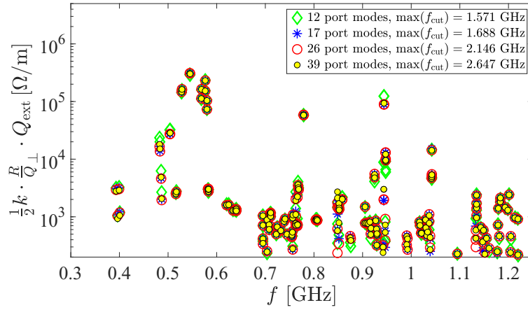
(c) Transversal impedance
