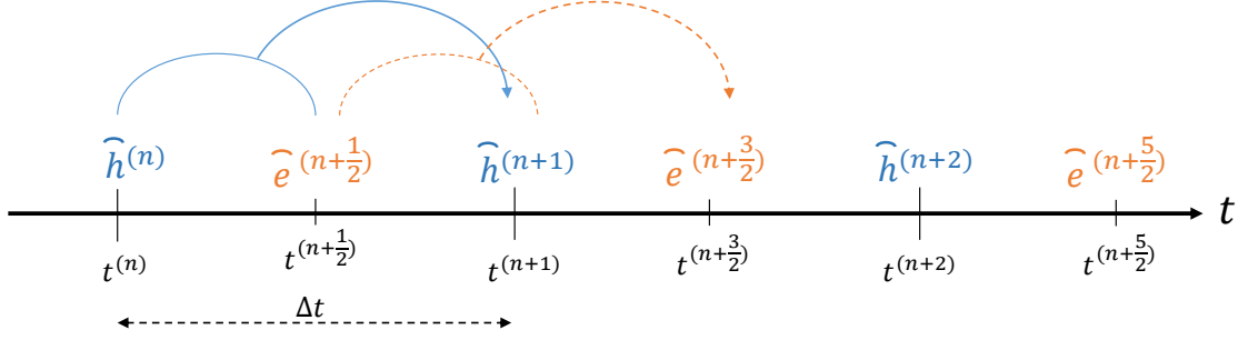
Figure 2.4: Leap-frog's time-updating scheme.
