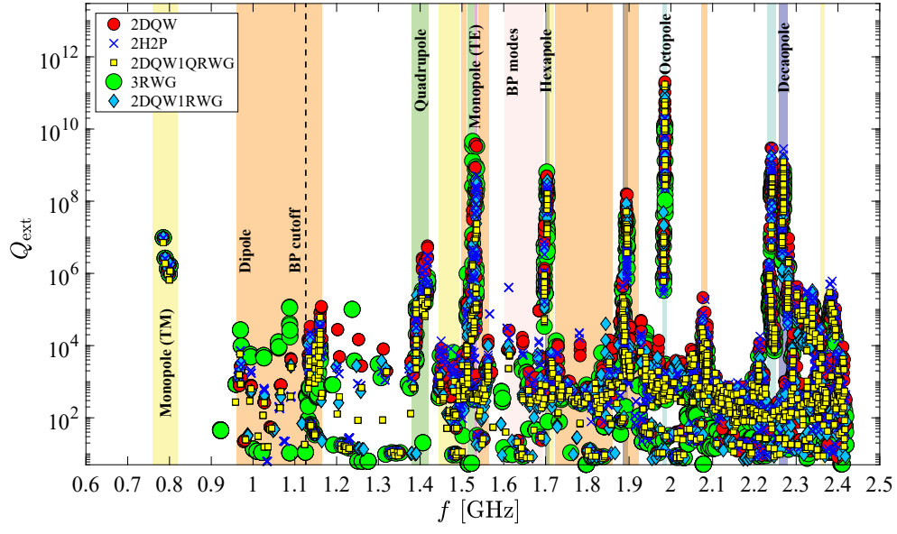
Figure 6.21: Q_{\text{ext}} of the four five-cell-cavity modules shown in Figure 6.16.
