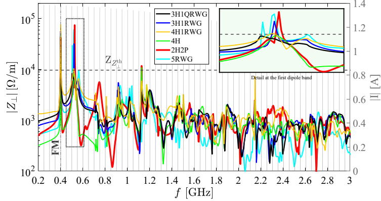
(a) Transversal impedance of the single-cavity module
