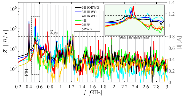
(b) Transversal impedance of the four-cavity module
