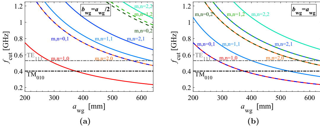
Figure 5.16: Cutoff frequencies of the lowest modes of a RWG with a 2:1 aspect ratio (a) and a 1:1 aspect ratio (b).
