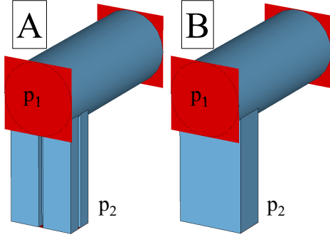
(a) QRWG vs. RWG
