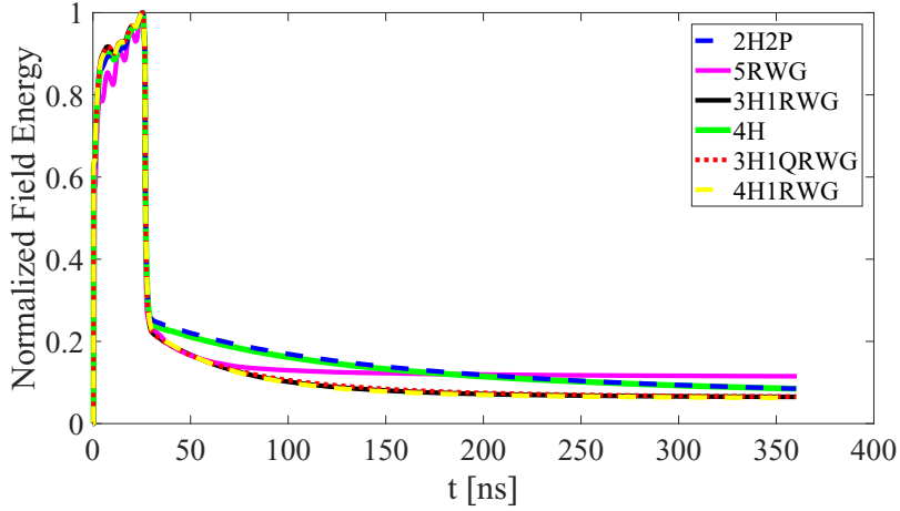
(b) Energy in the four-cavity module with tapering
