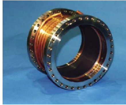
(b) BPA for KEKB. Figure reproduced from [110].
