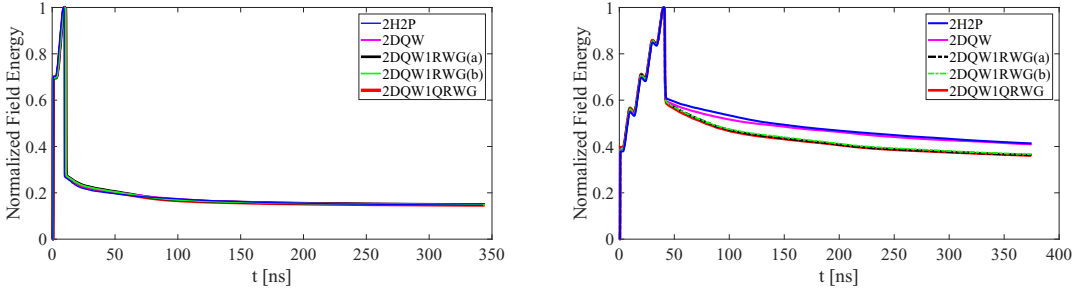
(a) Energy in the single four-cell-cavity module (b) Energy in the four four-cell-cavity module
