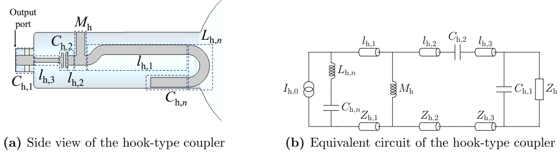
Figure 5.6: Side view of the hook-type HOM coupler with its equivalent circuit model for electric coupling [125, 105, 126]. The straight rods of the coupler are modeled by coaxial transmission lines with a length of l_{h,i} and a characteristic impedance of Z_{h,i} . Z_h is the characteristic impedance of the transmission line connected to the coupler (its standard value is 50 \Omega ).
