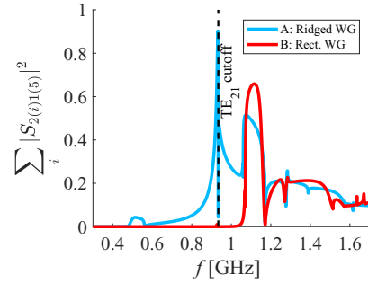
(f) Coupling of the second TE_{21} mode of P1 to P2
