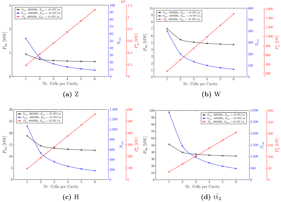
Figure 3.6: Wall plug power, number of cavities, and input power for different operating modes of FCC-ee. An aperture radius of 150 mm is chosen for the single-cell cavity and an iris radius of 120 mm is considered for the 400 MHz multi-cell cavities.
