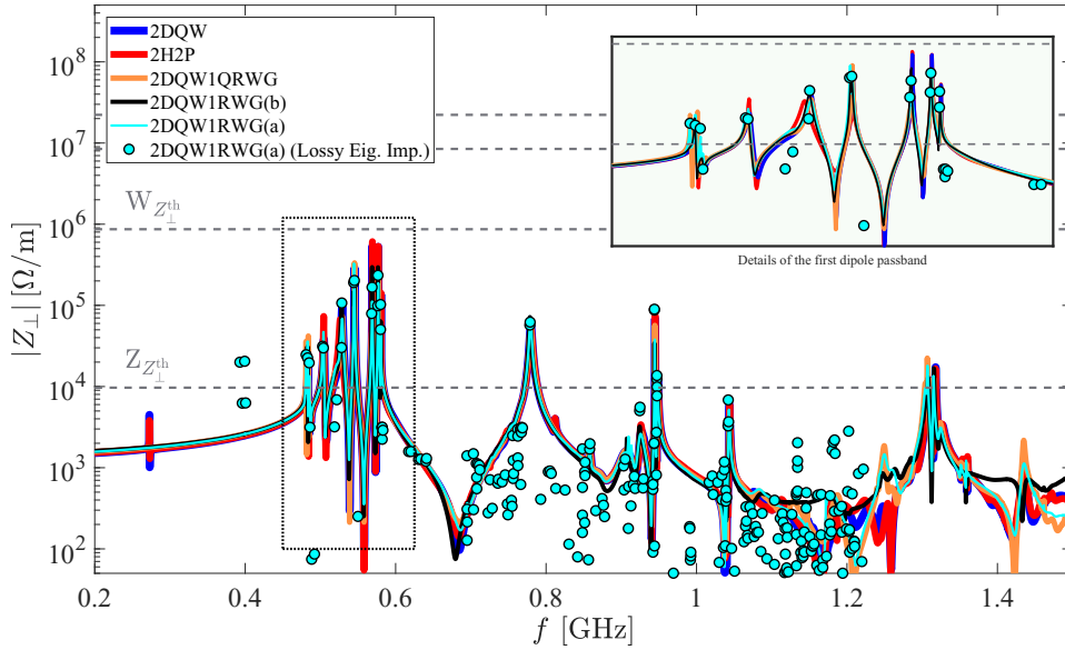
(b) Transversal impedance
