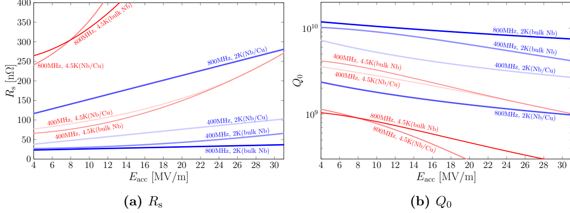
Figure 3.1: Surface resistance of bulk Nb and Nb/Cu at different frequencies and temperatures. Empirical formulas are used in each case to approximate the surface resistance [60]. In the approximation of R_s , B_{pk}/E_{acc} of 4.2 mT/(MV/m) is assumed. The quality factor is calculated by Q_0 = G/R_s where a value of 274 \Omega is assumed for G .
