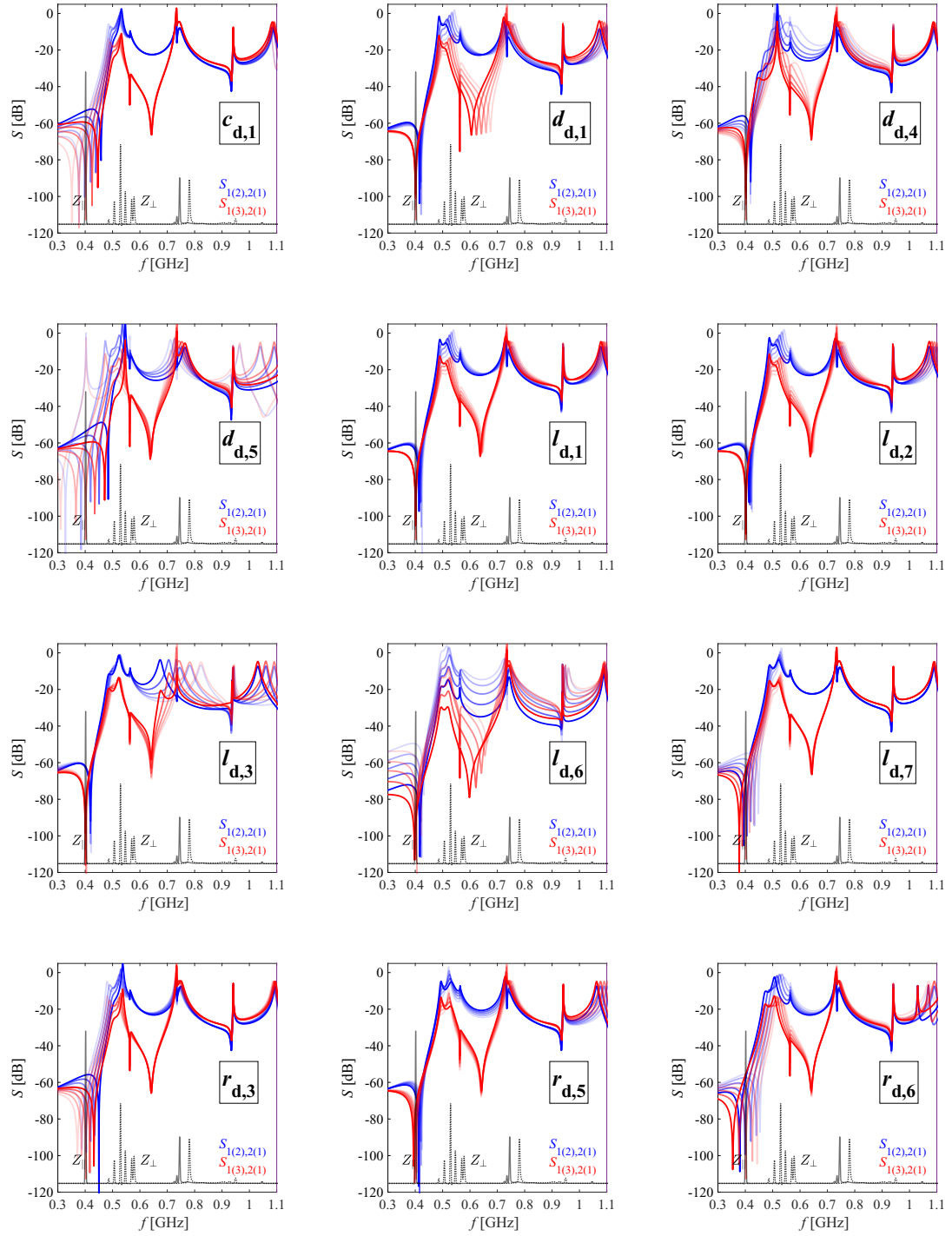
Figure 5.14: Dependency of the S-parameters on the geometrical parameters of the DQW coupler as parameterized in Figure 5.13. All of the geometrical parameters (except r_{d,6} ) are varied from -20\% (light color) to 20\% (dark color) around the nominal values given in Table 5.1. The parameter r_{d,6} is varied from -10\% to 10\% , and the value of d_{d,3} is changed in parallel to maintain the same capacitive distance c_{d,1} . The longitudinal and transversal impedance of the four-cell cavity are shown as black curves for reference.
