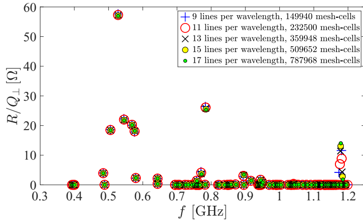
(c) Transversal shunt impedance
