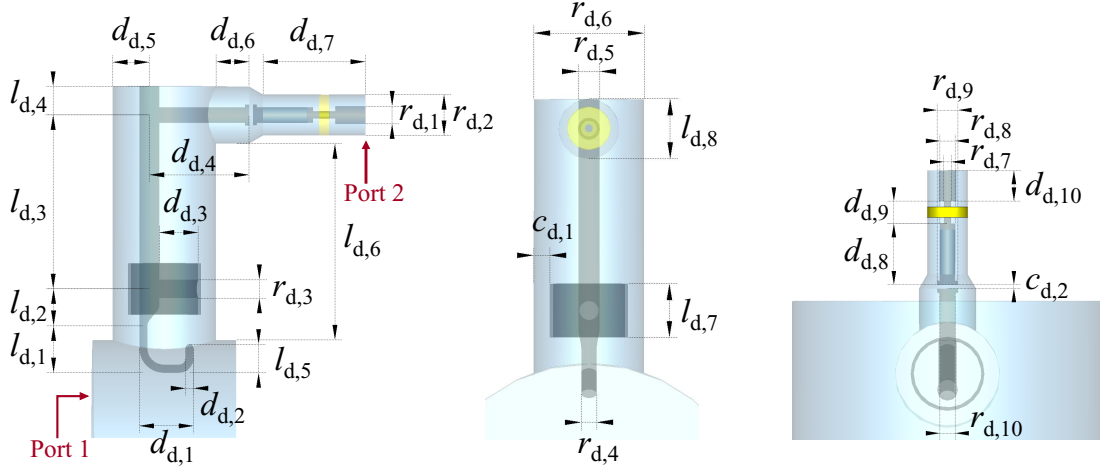
Figure 5.13: Parametrization of the DQW HOM coupler. A circuit model of the coupler is given in [129].
