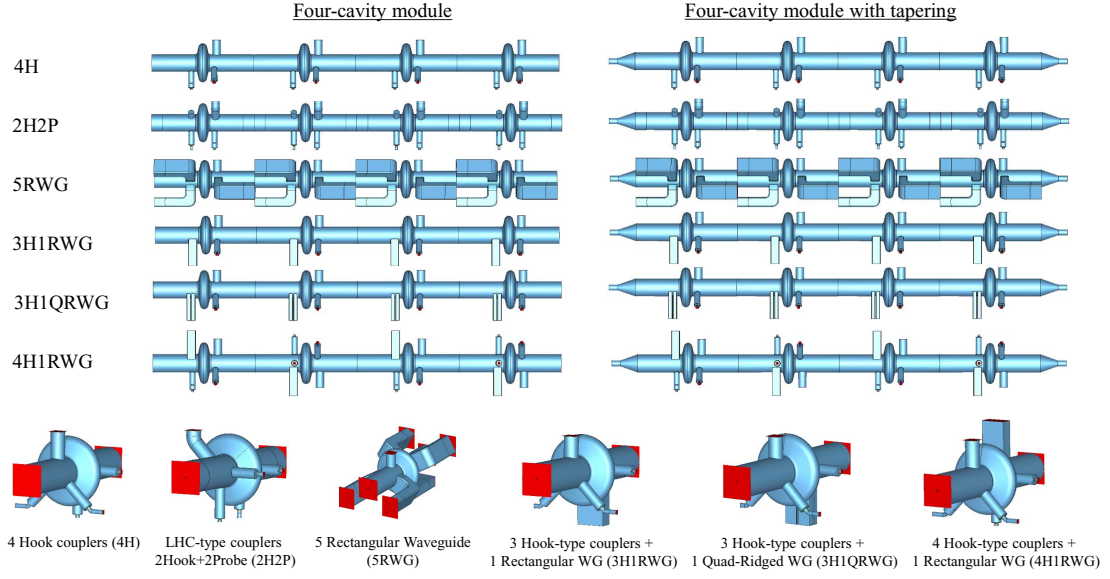
Figure 6.6: Various HOM damping schemes are applied to the single-cavity module, the four-cavity module and the four-cavity module with tapering. The tapers at the end of the module connect the large beam-pipe radius inside the module (here 156 mm) to the smaller beam-pipe radius outside the module (assumed to be 50 mm). A transition length of 300 mm is considered for the tapers.
