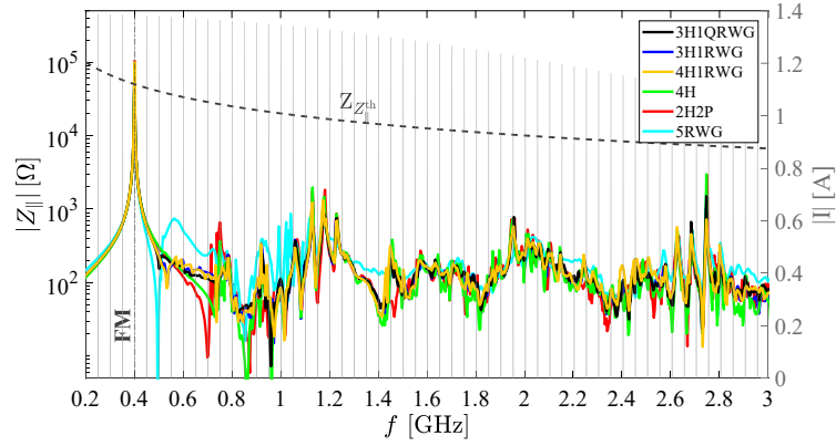
(b) Longitudinal impedance of the four-cavity module
