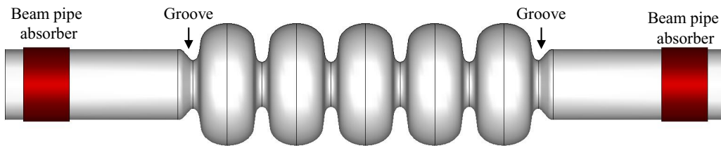
(c) A cavity with grooved beam pipe and beam pipe absorbers.
