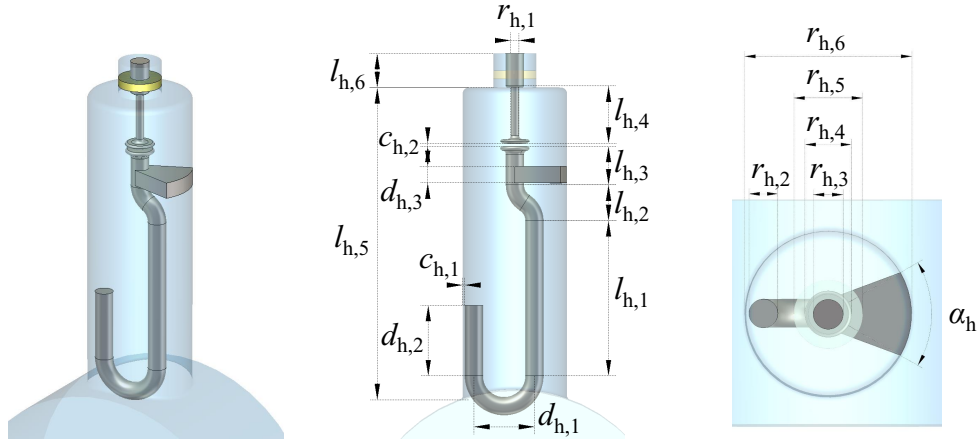
Figure 5.8: Parametrization of the hook-type LHC coupler.
