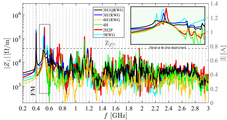
(c) Transversal impedance of the four-cavity module with tapering
