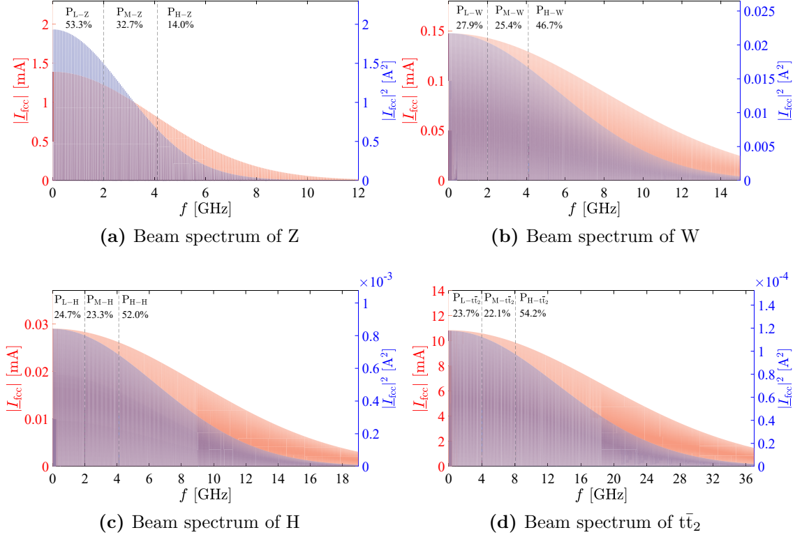
Figure 6.4: Beam spectra of different operating scenarios of FCC-ee using the parameters of Table 1.1. The spectra correspond to a simple beam filling scheme, assuming that all the bunches are uniformly distributed in the ring. Note that the beam spectra are symmetric around f = 0 , and here the positive frequency side of the spectra are shown. The distances between the spectral lines are 51 MHz, 6.1 MHz, 1 MHz, and 294 kHz for the Z, W, H, and t\bar{t}_2 working points, respectively (due to the condensed spectral lines, the spectra seem continuous). The current is doubled for the t\bar{t}_2 running, assuming that the same RF structure accelerates both beams.
