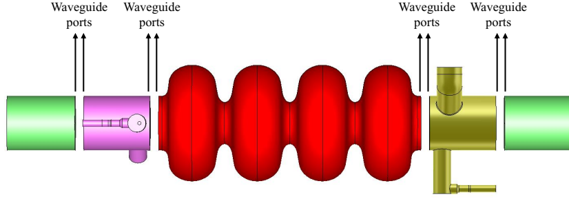
(a) Segments of the 2DQW damping scheme used by the SSC method
