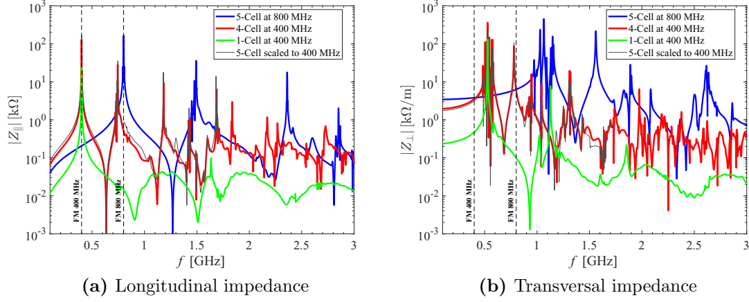
Figure 5.5: The longitudinal and transversal impedance of the single-cell, four-cell and five-cell cavities. The impedance is calculated for the bare cavity (without couplers) and the peaks are not fully resolved due to the truncated wake potential. In addition, the impedance of the five-cell cavity is scaled from 800 MHz to 400 MHz for comparison.
