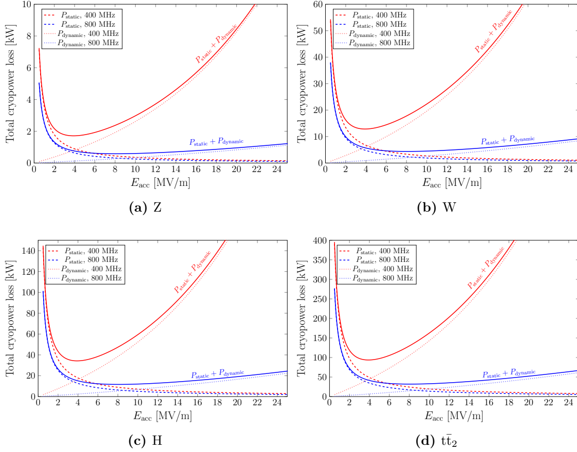
Figure 3.3: Dynamic and static power loss of the cavities at different operating modes of FCC-ee. A four-cell cavity at 400 MHz and a four-cell cavity at 800 MHz is assumed for each case. In the calculation of the static power loss, an extra length of twice the wavelength of FM ( 2\lambda_0 ) is considered for each cavity, i.e. L_{\text{cavity}} = L_{\text{active}} + 2\lambda_0 .
