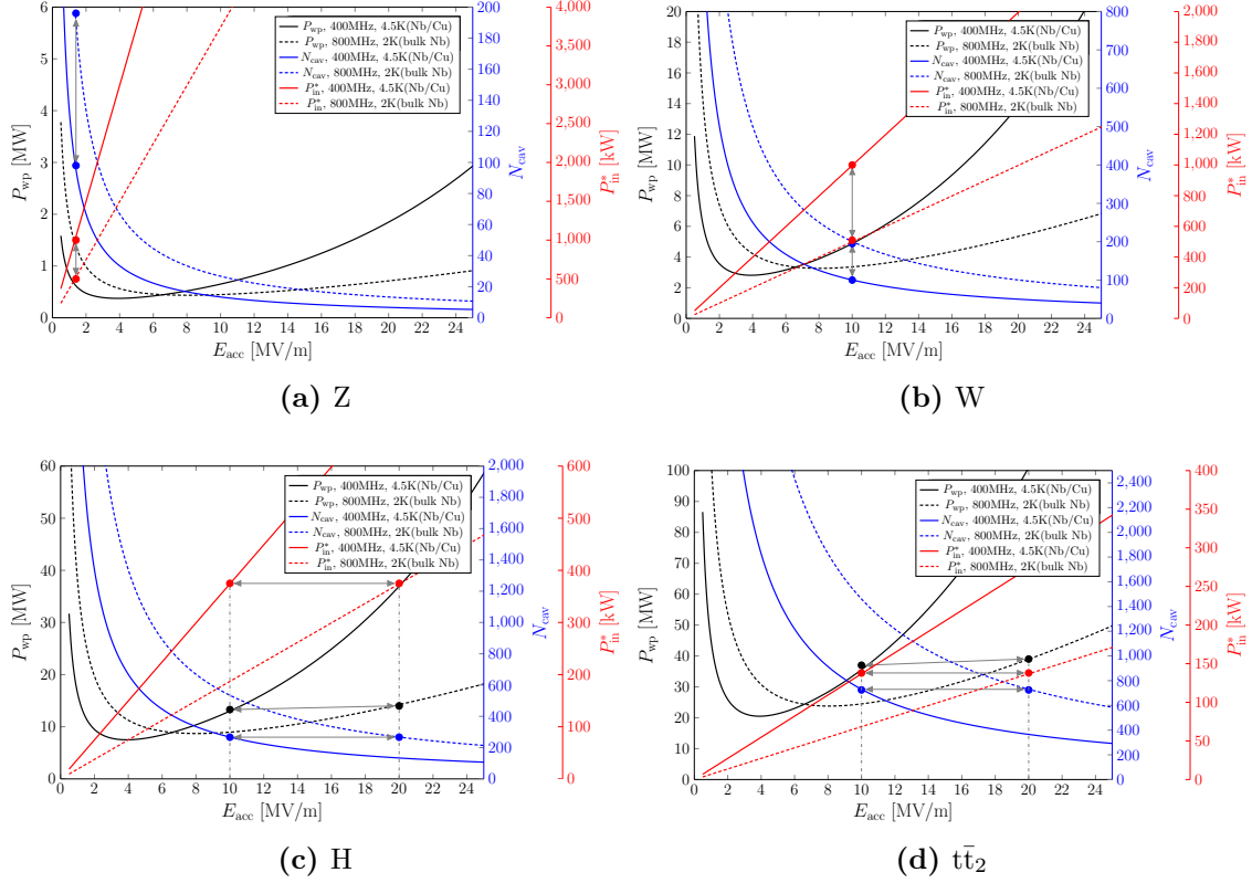
Figure 3.4: The wall plug power, the total number of cavities, and the required input power per cavity for different operating modes of FCC-ee. Four-cell cavities at 400 MHz and 800 MHz is assumed for each case. One RF system is considered to be used for both beams in the t\bar{t} working point. The number of cells for each case is determined in Subsection 3.2.2.
