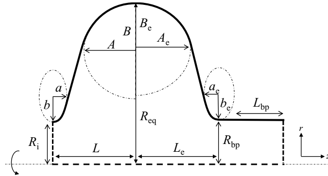
Figure 4.4: End cell parametrization of an elliptical cavity (parametrization is adapted from [93]). The inner side of the end cell is identical with the optimized middle cells, and the outer half-side, which is connected to the beam pipe, is changed in the end cell optimization. Note that the geometry is axisymmetric around the centerline, and only the upper part of the cross-section is shown.
