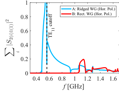
(b) Coupling of the first TE_{11} mode of P1 to P2
