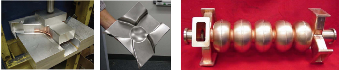
Figure 5.3: Niobium sheets are deep drawn (left) to form half of a three folded rectangular WG coupler (middle) [74] (©IOP Publishing. Reproduced with permission. All rights reserved). In the right picture, the WG coupler is electron-beam welded to a multi-cell cavity (figure is reproduced from [118] with author's permission).
