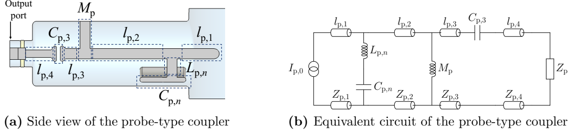
Figure 5.10: Side view of the probe-type HOM coupler with its equivalent circuit model for electric coupling [125, 105, 126]. The straight rods of the coupler are modeled by coaxial transmission lines with a length of l_{p,i} and a characteristic impedance of Z_{p,i} . Z_p is the characteristic impedance of the transmission line connected to the coupler.
