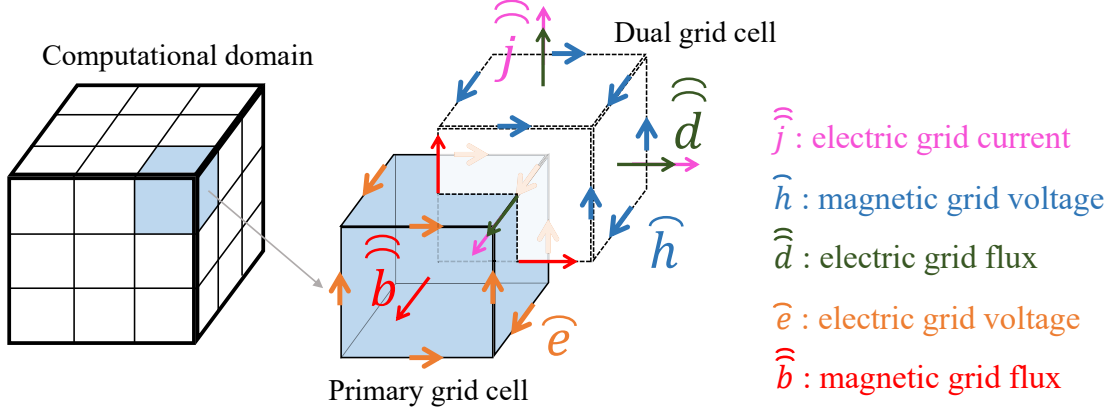
Figure 2.3: Topological FIT grid and state variables on hexahedral mesh.
