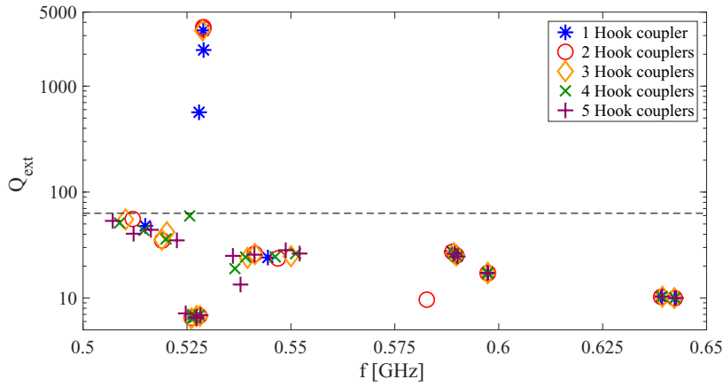
(b) Q_{\text{ext}} of the modes around the first dipole passband of the single-cell cavity
