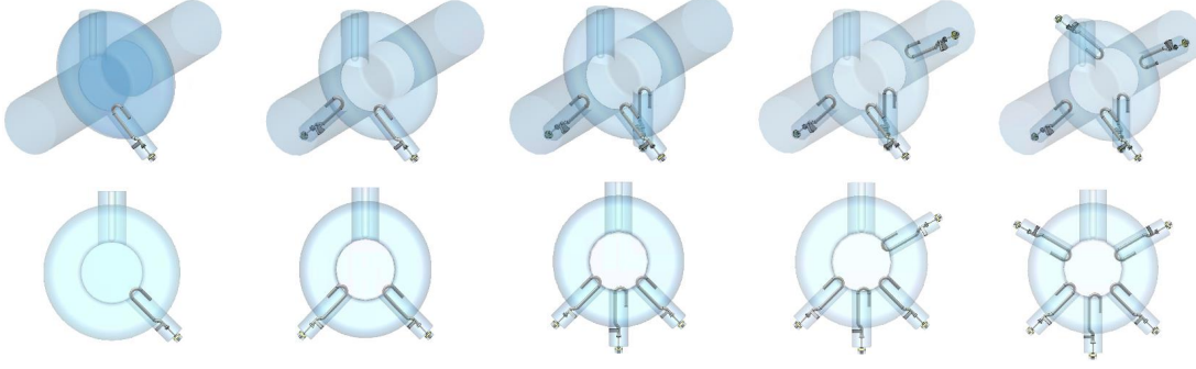
(a) HOM damping schemes using the hook-type HOM coupler
