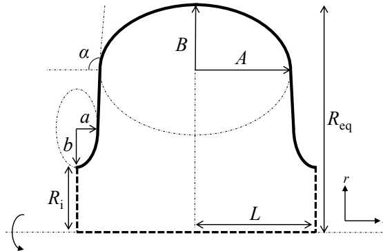
Figure 4.1: Middle cell parametrization of an elliptical cavity. The geometry is axisymmetric around the centerline, and here only the upper part of the cross-section is shown.
