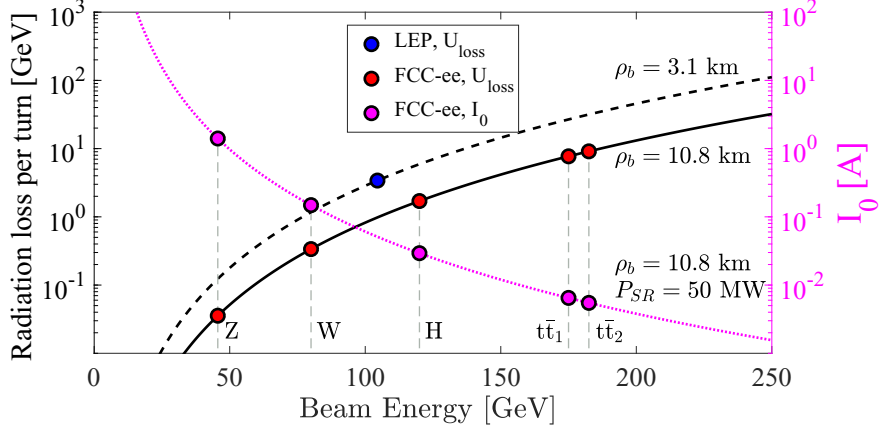
Figure 1.3: Radiation loss per turn for the FCC-ee and LEP as a function of beam energy is shown. For a given beam energy, the radiation loss in FCC-ee is lower than LEP due to the larger bending radius. Also shown is the beam current for the FCC-ee assuming 50 MW SR power loss per beam. For a fixed value of SR power loss, at lower energies higher beam current could be stored in the ring.
