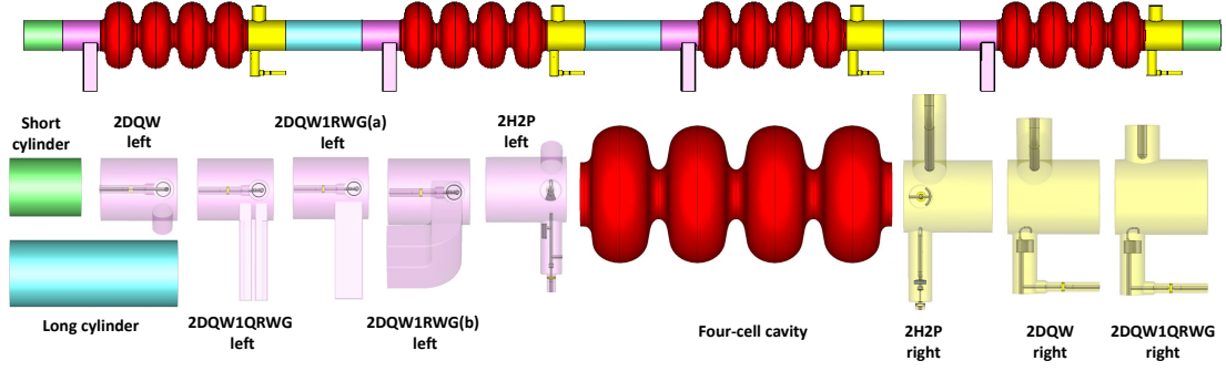
Figure 6.13: In the SSC method, the module is divided into 17 subsections. The top picture shows the complete module, while the bottom pictures show the different segments from which the whole modules shown in Figure 6.10 can be composed. The mesh density and the number of port modes for each segment are given in Appendix A.2.
