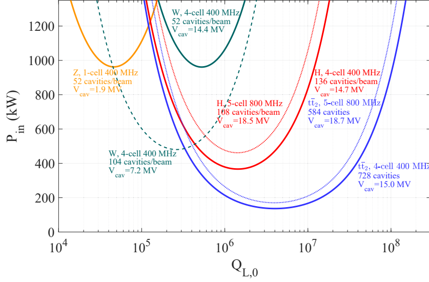
Figure 3.7: Input power as a function of Q_{L,0} with optimal detuning for different energy options.
