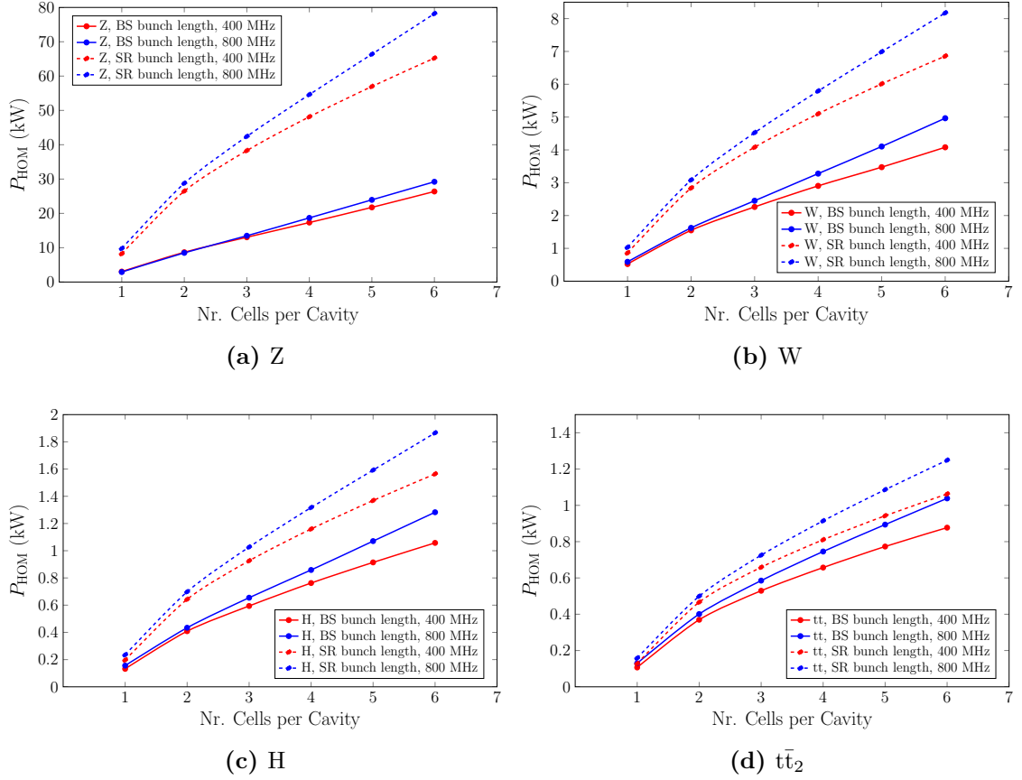
Figure 3.5: HOM power loss vs. the number of cells per cavity for different operating modes of FCC-ee. An aperture radius of 150 mm is chosen for the single-cell cavity and an iris radius of 120 mm is chosen for the 400 MHz multi-cell cavities (at 800 MHz the dimensions of the cavities are scaled by half).
