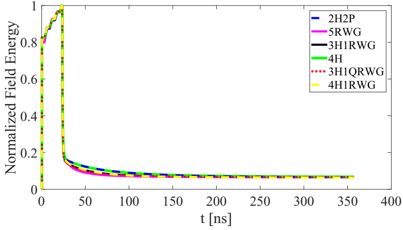
(a) Energy in the four-cavity module
