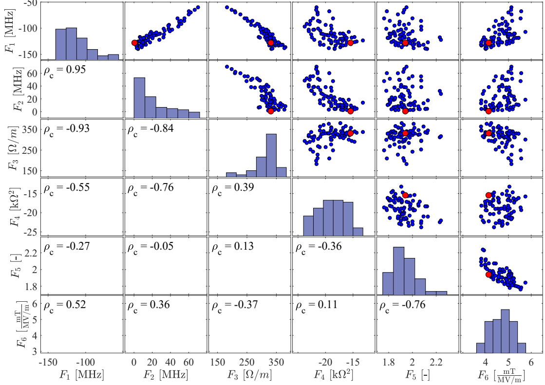
Figure 4.11: A scatter plot for each pair of objective functions of the individuals in the last generation of the GA. The numbers below the main diagonal are the correlation coefficients between the objective functions. The six objective functions cannot be minimized at the same time. The scatter plot shows the dependencies between the six objective functions, and the compromise one has to make for improving each objective function. The selected geometry is highlighted by red color.
