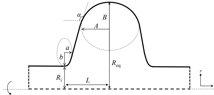
Figure 4.10: Single-cell parametrization of an elliptical cavity. The beam pipes should be considered during the optimization of the single-cell cavity. The geometry is axisymmetrical around the centerline, and only the upper part of the cross-section is shown.
