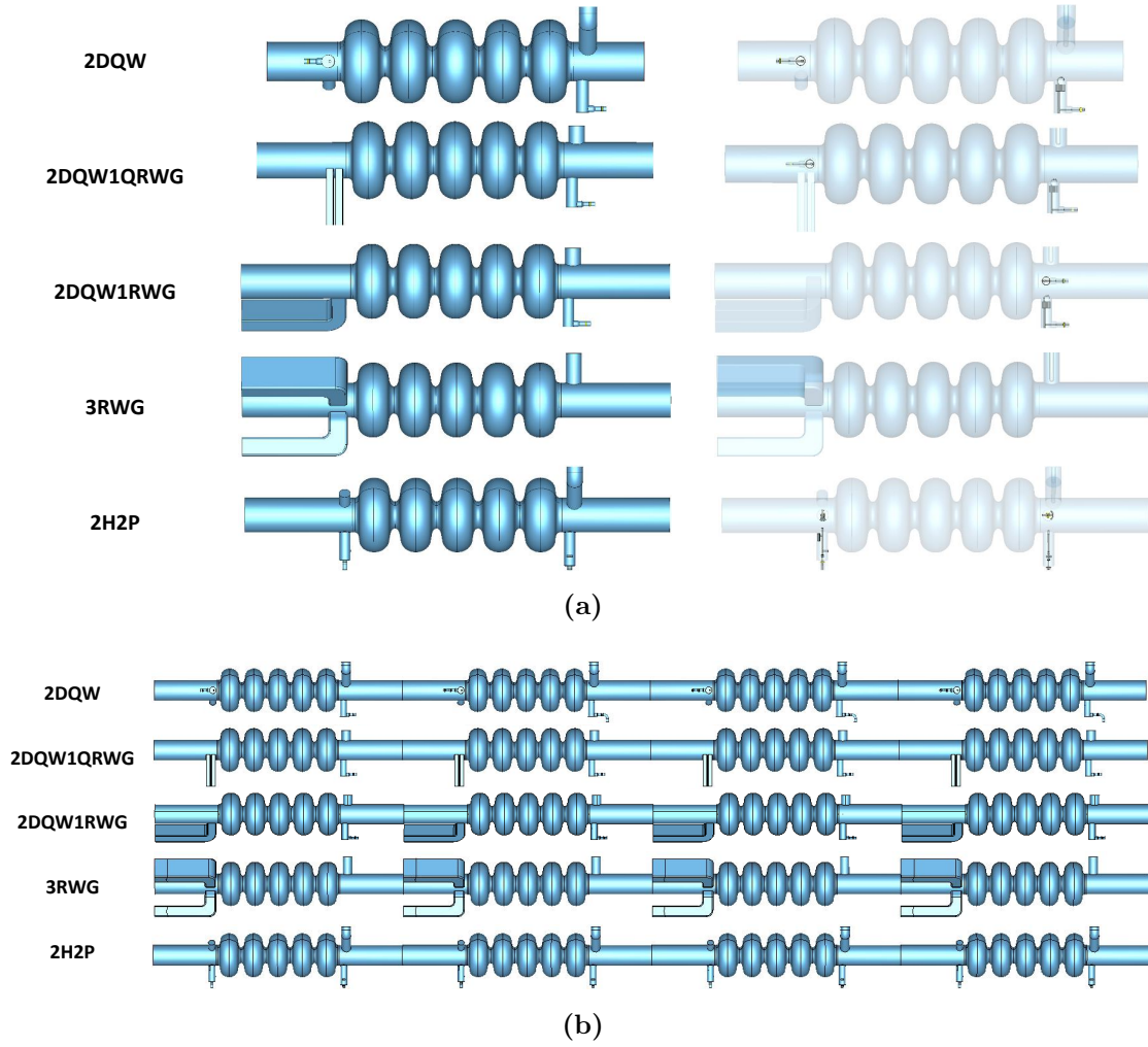
Figure 6.16: Layout of the five damping schemes considered for the five-cell 800 MHz cavities in a single five-cell-cavity module (a) and a four five-cell-cavity module (b).
