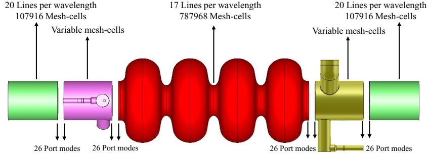
(a) Segments of the 2DQW damping scheme used by the SSC method
