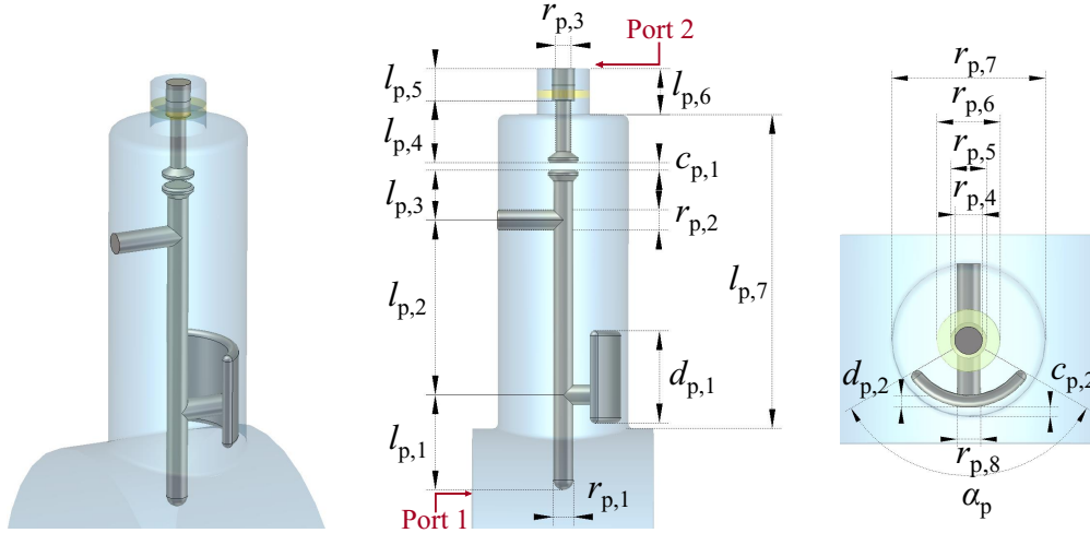
Figure 5.11: Parametrization of the probe-type LHC coupler.
