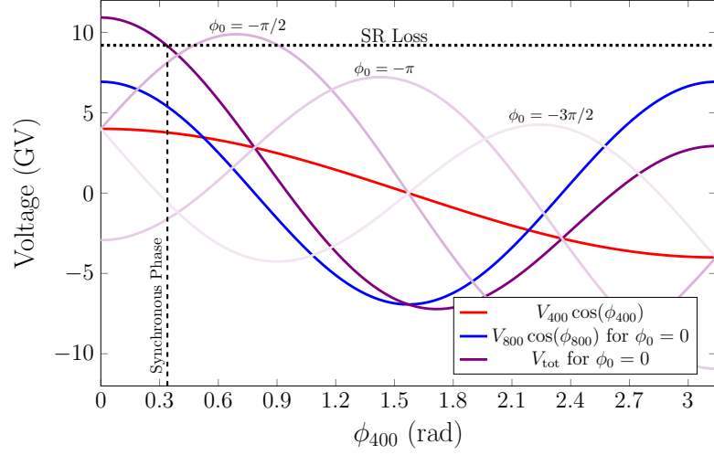
Figure 3.8: The total voltage of the t\bar{t} is a summation of 4 GV at 400 MHz and 6.93 GV at 800 MHz. Zero phase difference ( \phi_0 = 0 ) between the two frequencies provides the highest over-voltage (which corresponds to V_{RF} = 10.93 GV).
