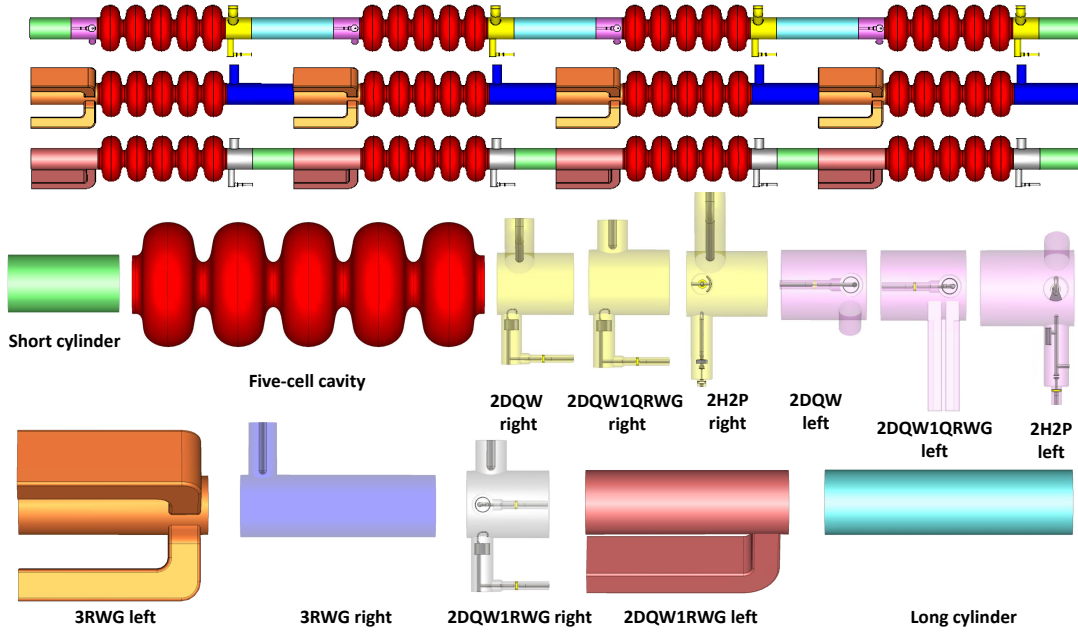
Figure 6.18: In the SSC method, the module is divided into several subsections. The first three pictures display the complete modules, while the last two rows show the different segments from which the whole modules shown in Figure 6.16 can be composed. The mesh density and the number of port modes for each segment are given in Appendix A.2.
