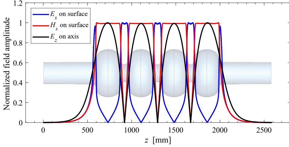
Figure 4.8: Four-cell cavity with the FM frequency at 400.79 MHz. The surface electric field, the surface magnetic field and the electric field along the longitudinal axis of the cavity are plotted. The magnitude of the fields is normalized in each case. The maximum value of the electric field is concentrated around the iris region of the cells, while the maximum value of the magnetic field is located around the equator of the cells.
