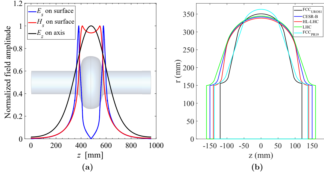
Figure 4.12: Field plot of the designed single-cell cavity (a) and a comparison between the surface profile of the designed cavity and some storage ring single-cell cavities (b).
