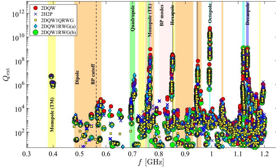
Figure 6.14: Q_{\text{ext}} of the modes in the four four-cell-cavity modules shown in Figure 6.10.
