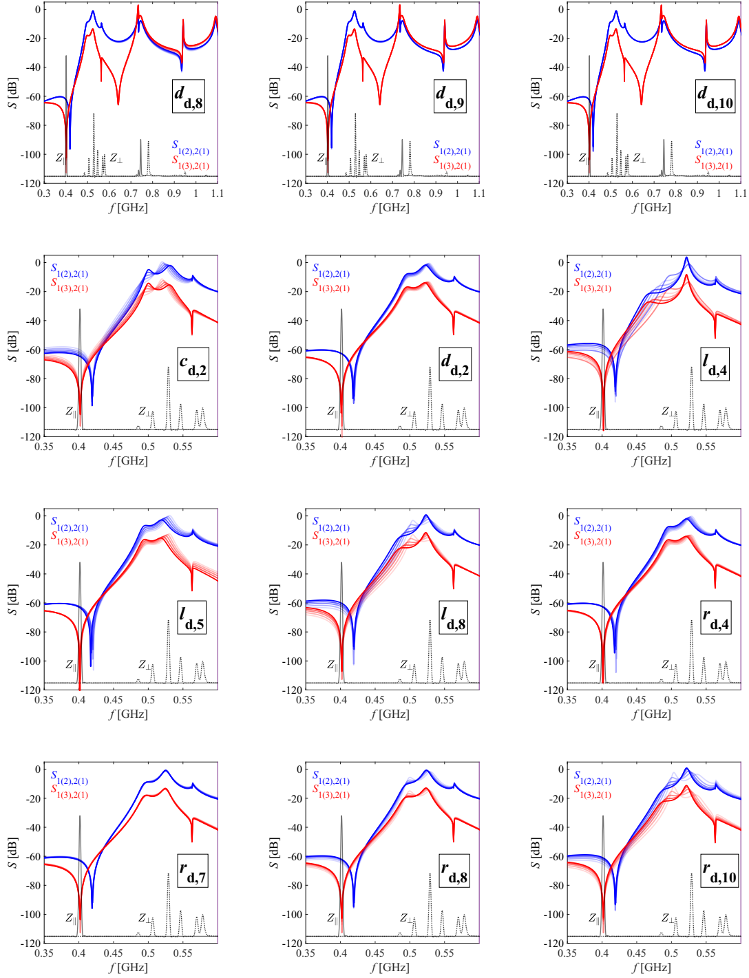
Figure 5.15: Dependency of the S-parameters on the geometrical parameters of the DQW coupler as parameterized in Figure 5.13. All the geometrical parameters (except l_{d,4} ) are varied from -20\% (light color) to 20\% (dark color) around the nominal value given in Table 5.1. The parameter l_{d,4} is varied from 0\% to 40\% . The longitudinal and transversal impedance of the four-cell cavity are shown as black curves for reference.
