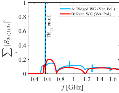
(c) Coupling of the second TE_{11} mode of P1 to P2
