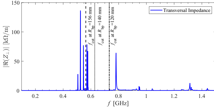
(b) Transversal impedance and the cutoff frequency of the TE_{11} mode of a cylindrical waveguide.
