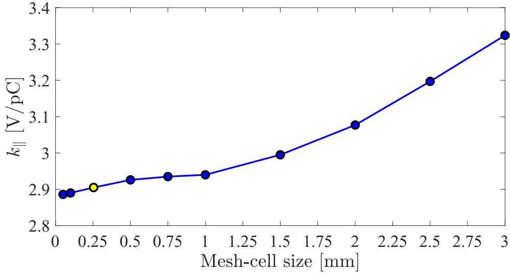
Figure A.1: Mesh convergence study for the loss factor of the five-cell cavity considering the BS bunch length of tt_2 using the ABCI software. The x -axis shows the mesh sizes in the r and z directions. The mesh-cell size of the yellow marker equals one-tenth of the bunch length. This mesh-cell size was used in the calculation of loss factors in Table 6.9.
