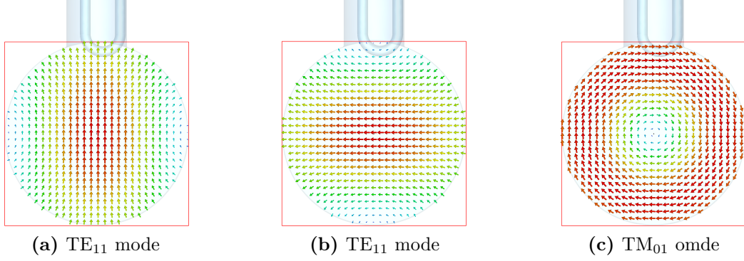
Figure 5.7: The first three modes of a circular waveguide. The electric field of the TE 11 mode is shown in (a) and (b), and the magnetic field of the TM 01 mode is shown in (c). The TE 11 mode is a degenerated mode and thus has two polarizations.
