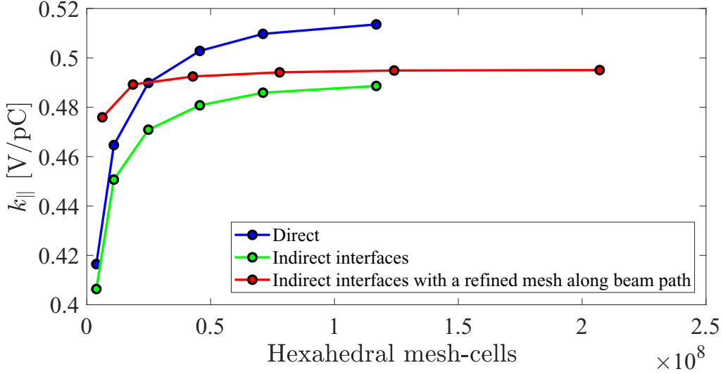
Figure A.2: Mesh convergence study for the loss factor calculation of the 2DQW single-cavity damping scheme shown in Figure 6.10. A Gaussian beam with a length of 25 mm is considered in the definition of the particle beam. Different wake integration methods are used in the wakefield calculations. In general, the “direct method” is less accurate than the indirect methods [51]. A detailed description of the graph is given in Table A.2.
