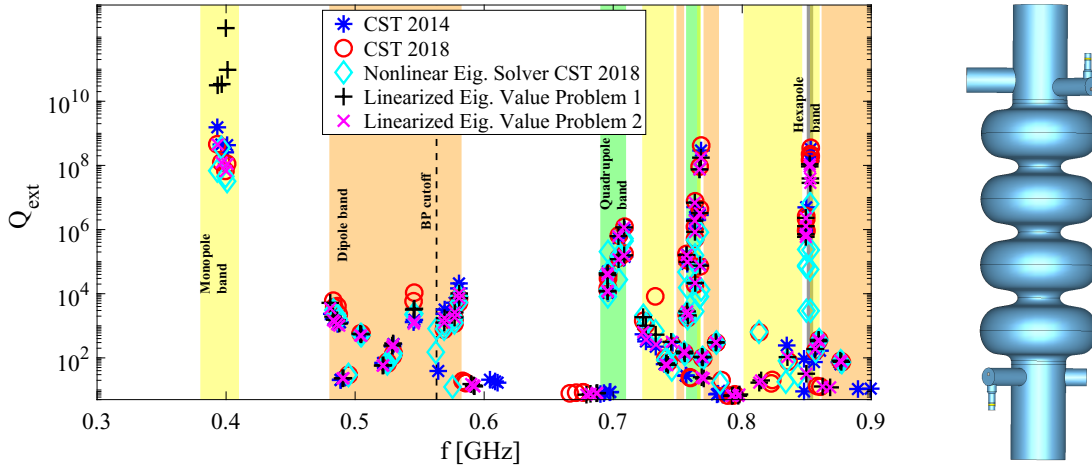
Figure 6.2: This plot shows the Q_{\text{ext}} of some passbands of a four-cell cavity with two DQW HOM couplers computed with different approaches. In the linearized case, the SSC method is applied to the system matrices that are exported from CST Studio Suite ® 2014. In the first linearized case, the complex wave impedance and in the second linearized case, the absolute value of the wave impedance is considered at the port boundaries. In CST 2014, CST 2018 and the nonlinear eigenmode solver of CST 2018, a tetrahedral mesh is used, and in the linearized cases (in the SSC method) a hexahedral mesh is employed.
