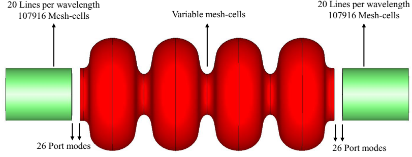
(a) Segments of the bare cavity used by the SSC method
