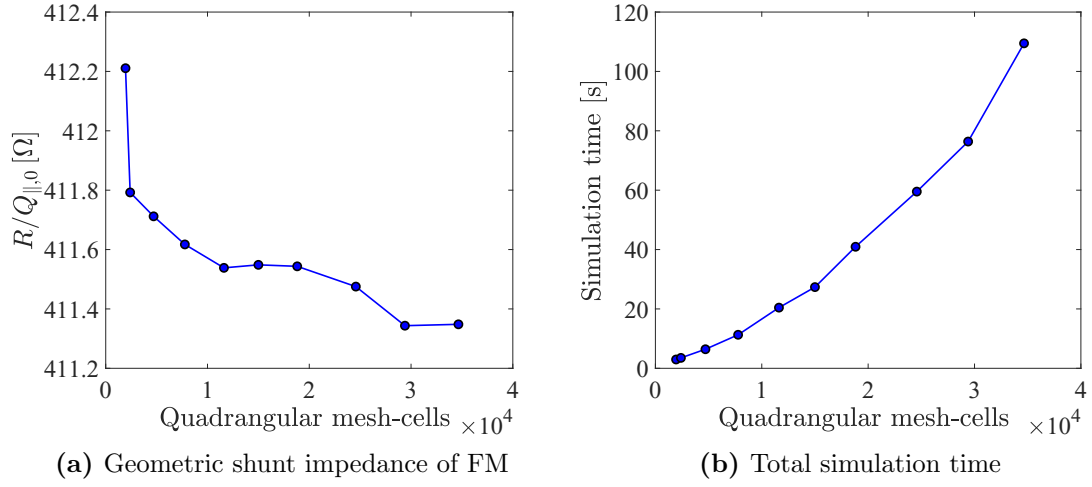
Figure A.3: Mesh convergence study for the calculation of R/Q_{||,0} of the four-cell cavity given in Table 4.3 using SUPERLANS. The simulation time represents the total time required to calculate four modes in the first monopole passband.
