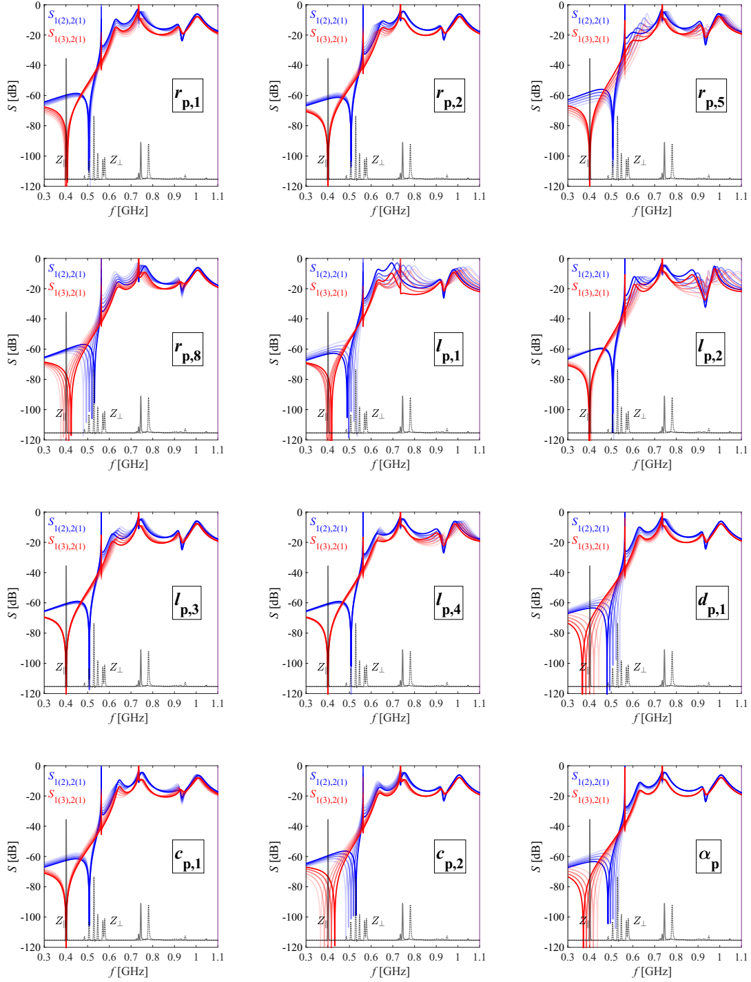
Figure 5.12: Dependency of the S-parameters on the geometrical parameters of the probe-type coupler as depicted in Figure 5.11. The geometrical parameters are varied from -20\% (light color) to 20\% (dark color) around the nominal values given in Table 5.2. The longitudinal and transversal impedance of the four-cell cavity are shown as black curves for reference.
