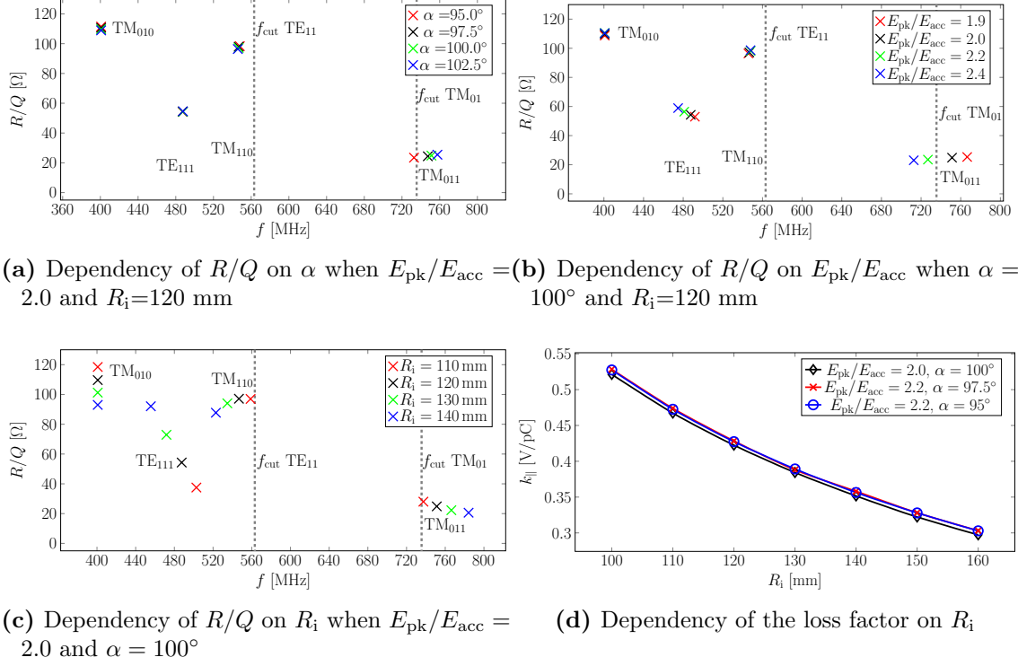
Figure 4.3: Dependency of the frequency and R/Q of the first two monopole and dipole modes of the cavity on the constraints of (4.3). The longitudinal shunt impedance R/Q_{||} is calculated for the TM_{010} and TM_{011} modes and the transversal shunt impedance R/Q_{\perp} for the TE_{111} and TM_{110} modes, using (2.41) and (2.44), respectively. The vertical dashed lines represent the cutoff frequencies of the TE_{11} and TM_{01} modes of a cylindrical beam pipe with a radius of 156 mm. The TE_{111} and TM_{110} modes in the cavity couple to the TE_{11} mode, and the monopole mode TM_{011} couples to the TM_{01} mode of the cylindrical beam pipe. The drastic change in the R/Q_{\perp} of the TE_{111} mode in (c) arises from the non-zero tangential electric field values at both ends of the cell (the second bracket in (2.39) and (2.40) is not zero because of the PMC boundary condition). In a multi-cell cavity or in the presence of beam pipes this dependency is not observed.
