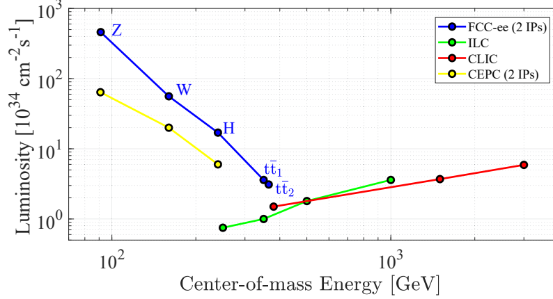
Figure 1.2: Expected luminosity of different lepton colliders as a function of center-of-mass energy. FCC-ee and CEPC [15] are circular colliders with two Interaction Points (IP) and ILC [16] and CLIC [17, 18] are linear colliders.
