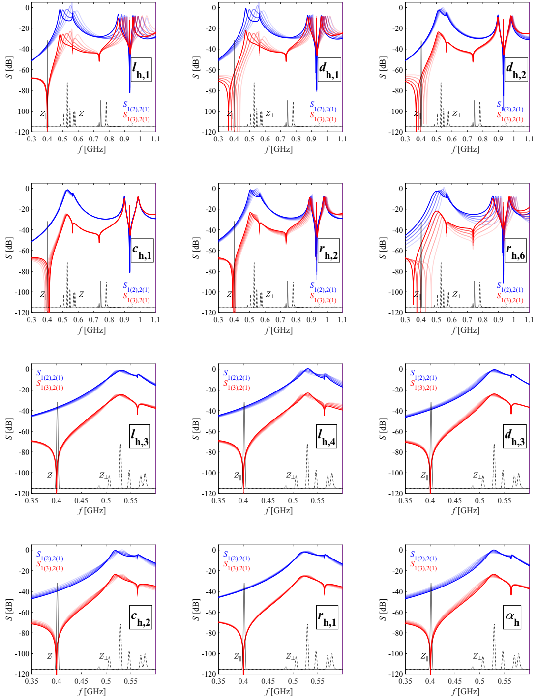
Figure 5.9: Dependency of the S-parameters on the geometrical parameters of the hook-type coupler as depicted in Figure 5.8. All the geometrical parameters (except d_{h,1} ) are varied from -20\% (light color) to 20\% (dark color) around the nominal values given in Table 5.1. Due to the lack of space, d_{h,1} is varied from -10\% to 10\% . The longitudinal and transversal impedance of the four-cell cavity are shown as black curves for reference.
