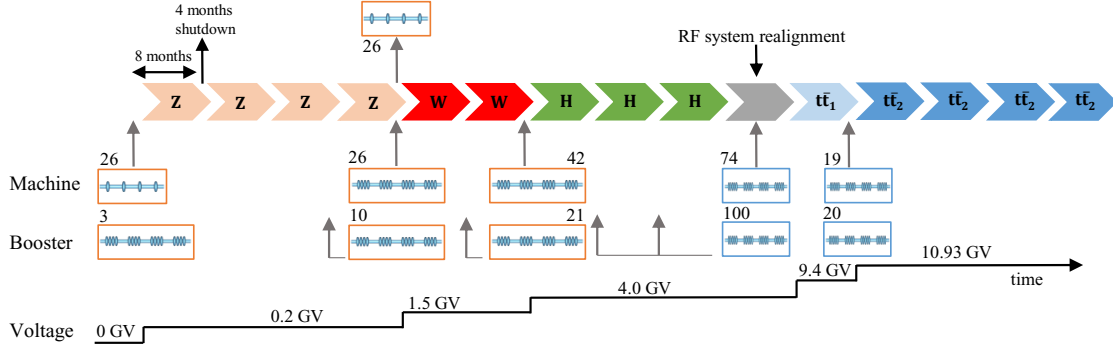
(b) Development of the machine voltage from 0 GV to 10.93 GV (picture is adapted from [10, p. 416]).
