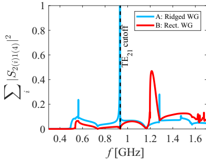
(e) Coupling of the first TE_{21} mode of P1 to P2
