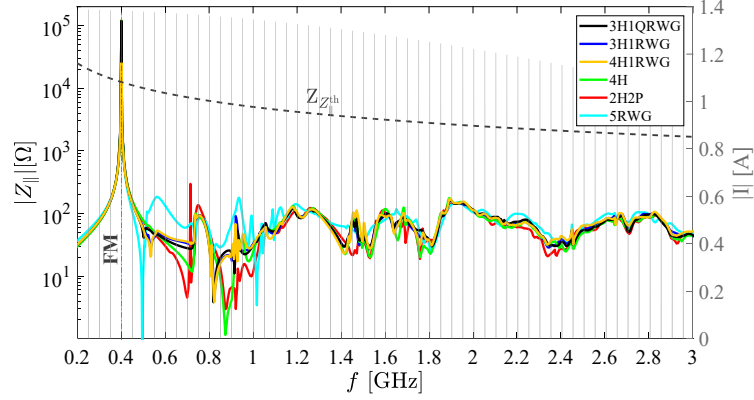
(a) Longitudinal impedance of the single-cavity module
