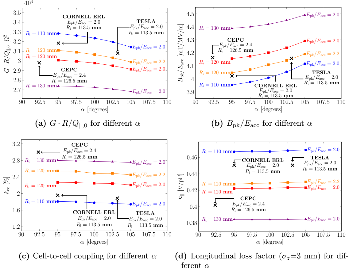
Figure 4.2: Middle cell optimization for different values of E_{pk}/E_{acc} , \alpha and R_i . The dimensions of the CEPC [63], TESLA [65] and CORNELL ERL [93] cavities are scaled to 400.79 MHz for comparison. For each point in the graphs, the optimization problem of equation (4.3) is solved for the TM_{010} - \pi mode. Each curve in (b) represents a Pareto front that depends on the constraints of the optimization problem (4.3).
