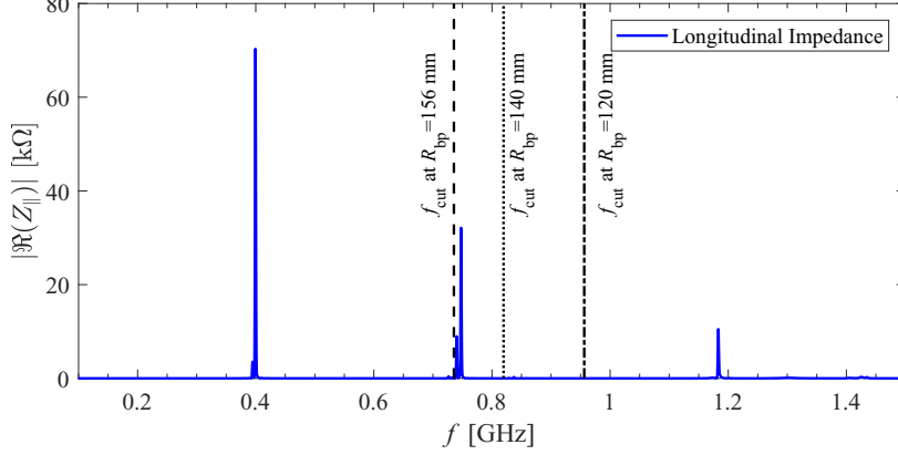
(a) Longitudinal impedance and the cutoff frequency of the TM_{01} mode of a cylindrical waveguide.
