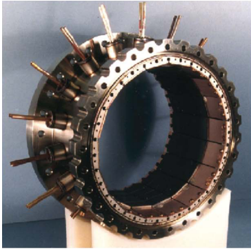
(a) BPA for CESR. Figure reproduced from [109]: ©[1999] IEEE.
