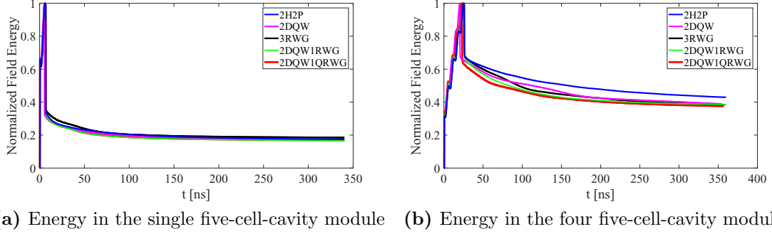
Figure 6.17: Energy remaining in the cavities (as shown in Figure 6.16) after excitation by a relativistic Gaussian beam with a length of 12.5 mm and a charge of 1 nC. The energy is computed from the wakefield calculation with a simulated wakelength of 100 m.
