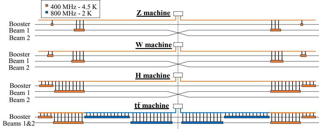
(a) Machine development after each operation. The picture shows only the RF section of the 100 km ring. Both beams are re-aligned for the t\bar{t} machine (picture is adapted from [10, p. 466]).
