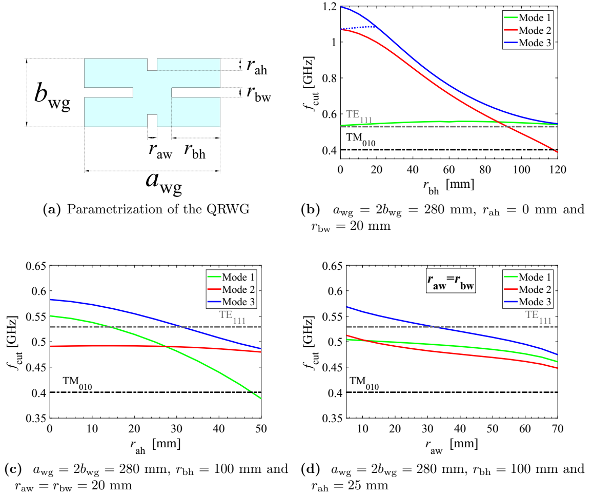
Figure 5.17: QRWG parametrization (a) and the cutoff frequencies of the first three modes plotted with respect to the ridge dimensions (b-d). The field distribution of modes 1, 2 and 3 corresponds to the TE_{10} , TE_{01} and TE_{11} modes of a RWG, respectively. For small values of r_{bh} in (b), the TE_{20} mode is the third smallest mode (indicated by the dotted blue line). The frequency of the FM and the first dipole mode of the single-cell cavity are shown in dashed horizontal lines.
