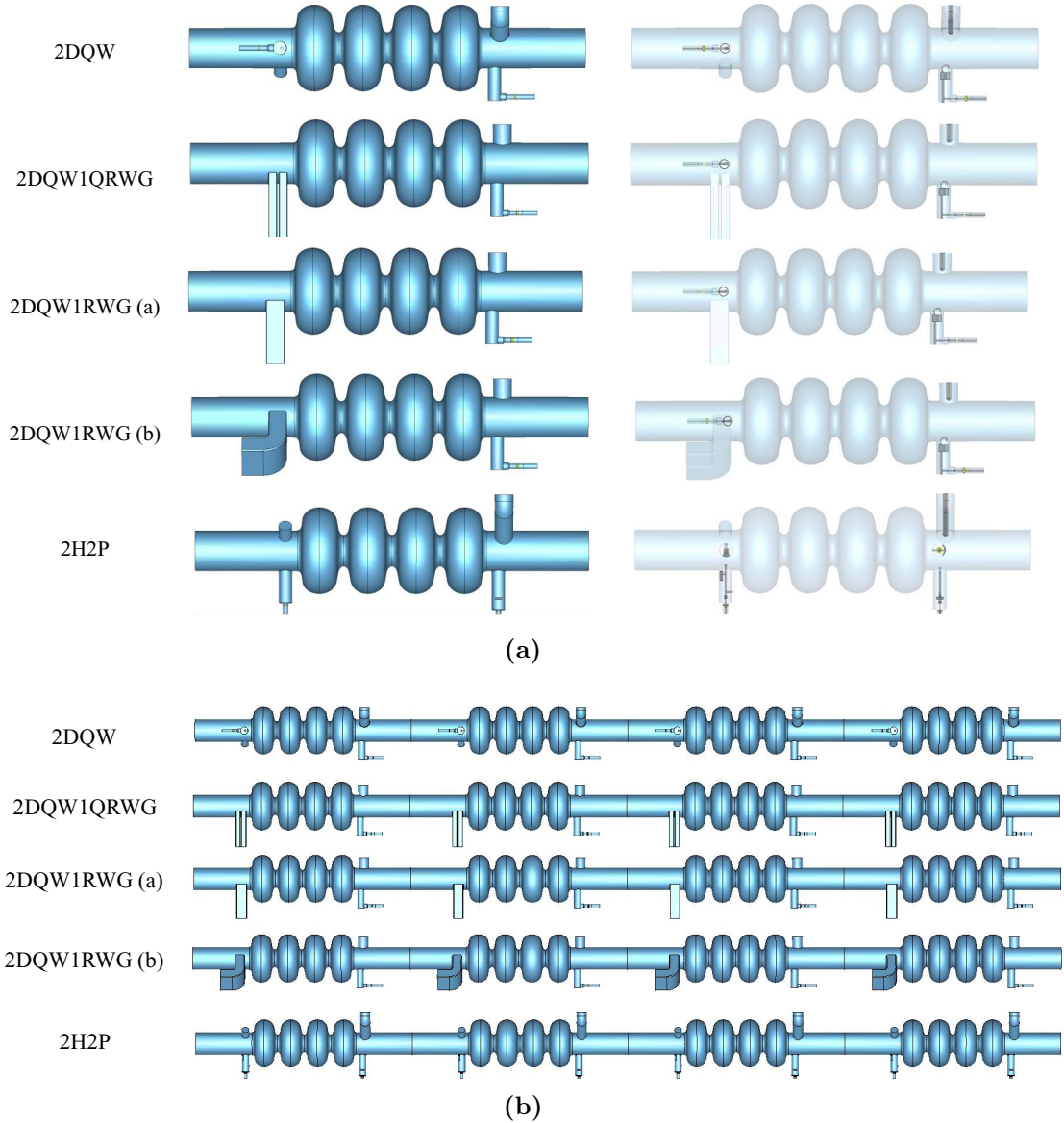
Figure 6.10: Layout of the five damping schemes considered for the four-cell 400 MHz cavities in a single four-cell-cavity module (a) and a four four-cell-cavity module (b).
