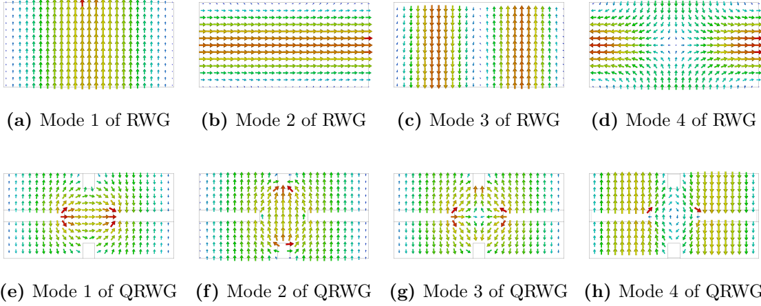
Figure 5.18: The first four modes of the RWG and the QRWG. Depending on the dimensions of the ridges, the order and the field pattern of the modes change when transforming the RWG into the QRWG.
