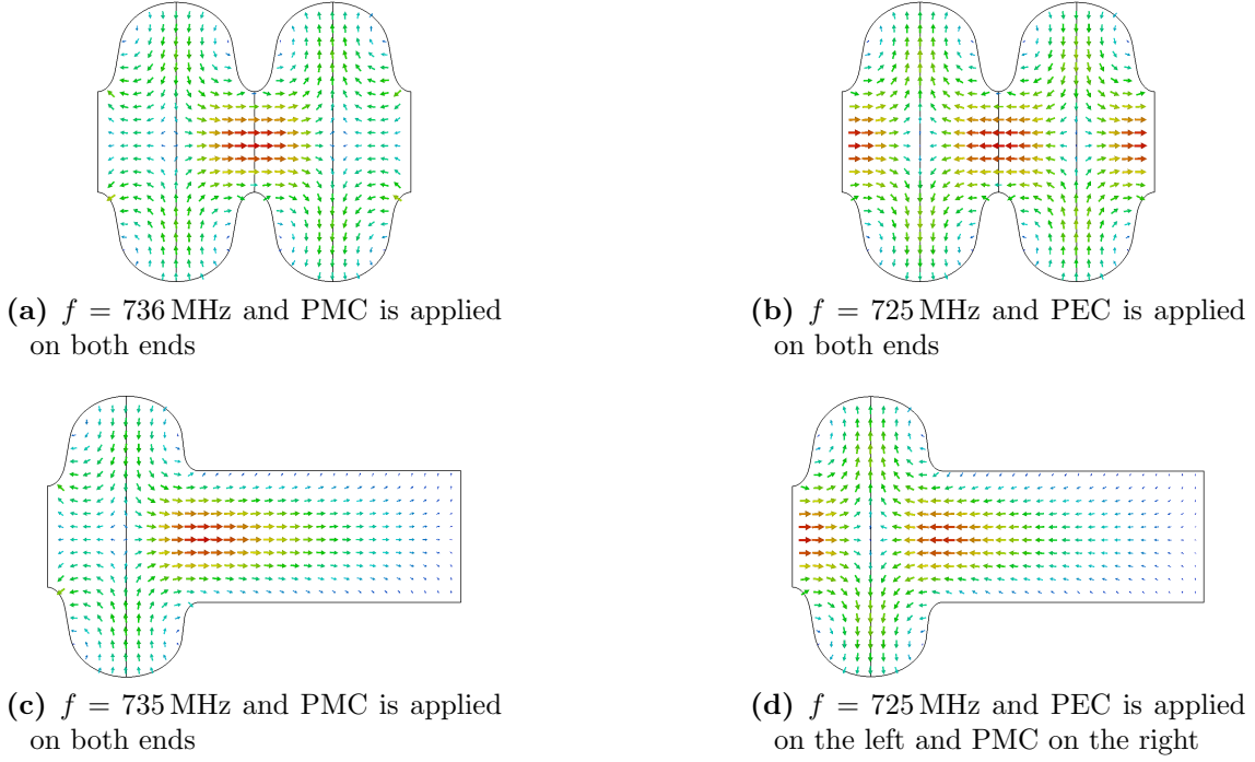
Figure 4.6: Field distribution of the first TM_{011} -type mode in the two inner cells (a)-(b) and the end cell (c)-(d) under different boundary conditions. At the end of the beam pipe in (c) and (d) PMC boundary condition is applied, while in the inner side that connects to the middle cells different boundary conditions are used.
