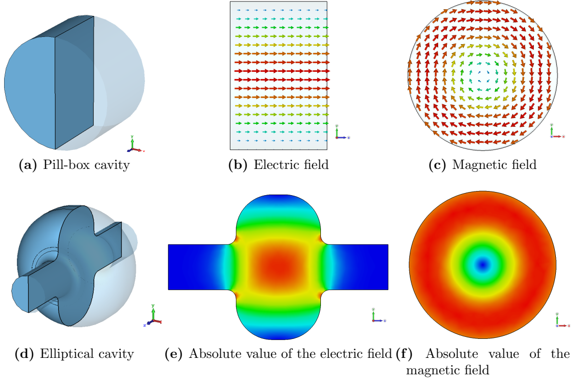
Figure 2.1: 3D model of a pillbox cavity (a) and a more realistic shape derived from the pillbox cavity with beam pipes and rounded edges (d). The electric and magnetic field distribution of the TM_{010} mode is also shown. The red color indicates a high magnitude of the electric and magnetic field, and the blue color corresponds to zero magnitude of the field.
