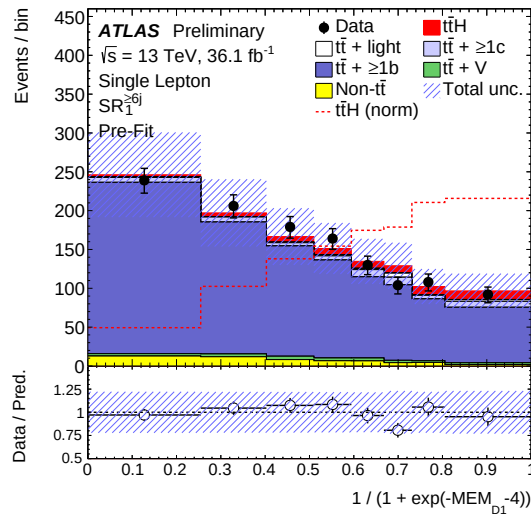
Figure 57: Distribution of the MEM_{D_1} discriminant in the SR_1^{\geq 6j} region. From Ref. [91].
