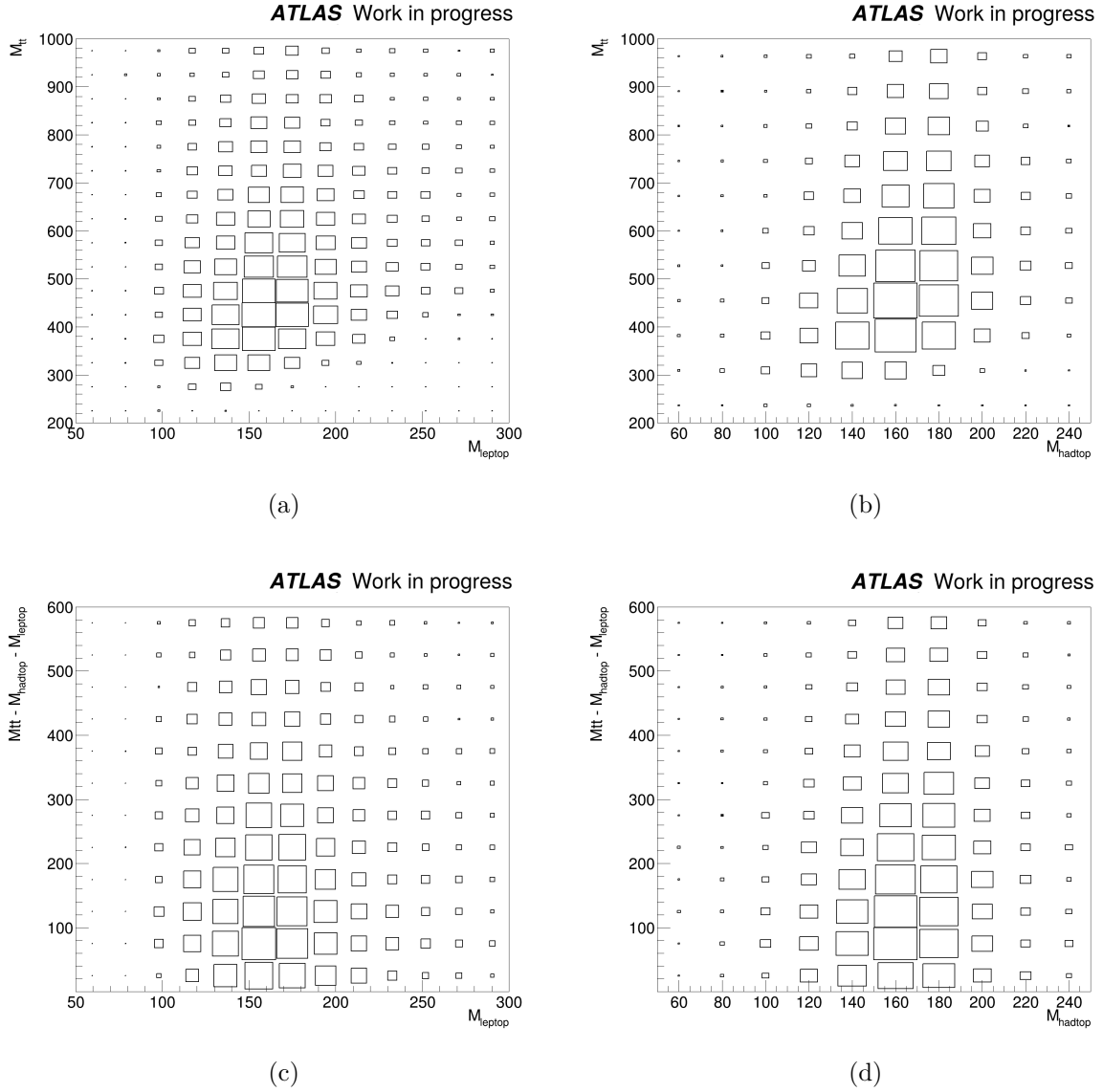
Figure 67: Two-dimensional distributions of M_{t\bar{t}l} vs (a) M_{t_l} and (b) M_{t_h} , and M_{t\bar{t}} - M_{t_l} - M_{t_h} vs (c) M_{t_l} and (d) M_{t_h} in t\bar{t}H MC events with \geq 6 jets and \geq 4 b -tagged jets (at the tight working point).
