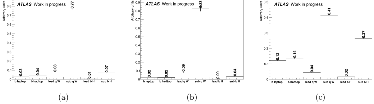
Figure 73: Distributions of the partonic origin of the missing jet in the t\bar{t}H events with (a) \geq 6 jets, \geq 4 b -jets, (b) 5 jets, \geq 4 b -jets and (c) \geq 6 jets, 3 b -jets. The number of b -jets is evaluated at the tight working point.
