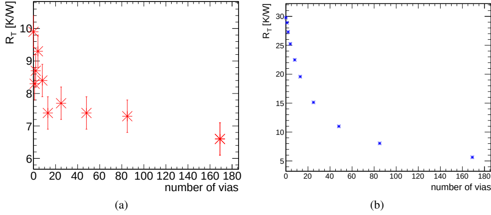
Figure 4.9: Thermal resistance in dependence of the number of vias a): Measured. b): Computed.
