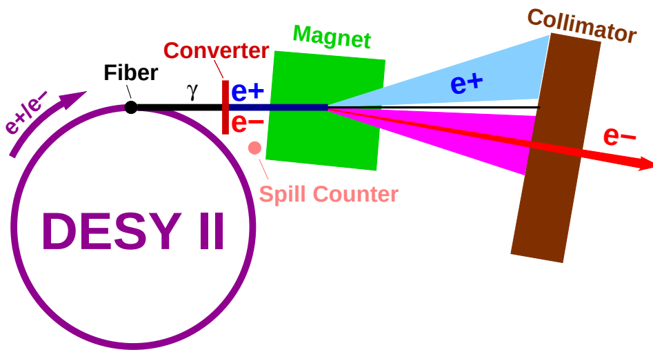
Figure 4.1: Schematic of the electron generation at the DESY II testbeam. [35]
