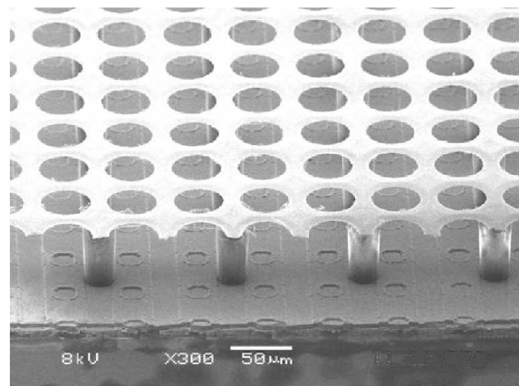
(b) Microscopic image of a Micromegas (InGrid)[26]
