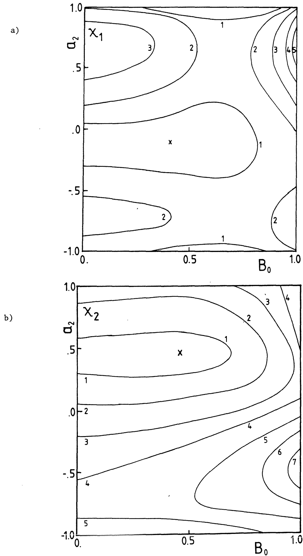
Fig.4.12: Likelihood contours in the B_0 - a_2 plane for the x_1 (a) and x_2 (b) events. Contour number n corresponds to a decrease of the likelihood function by a factor \exp(-0.5n^2) with respect to its maximal value. The maximum of the likelihood function is indicated by a cross.
