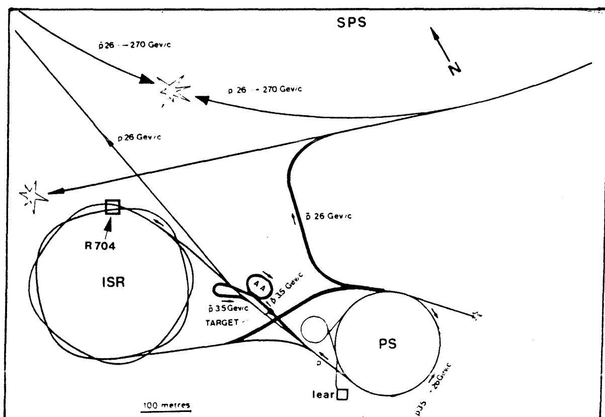
Fig. 2.1: The CERN antiproton complex. From [45].
