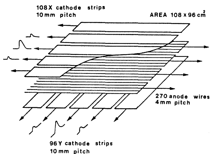
Fig.2.12: Layout of the analog chambers. From [44].
