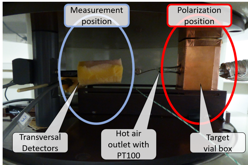
(A) The photo shows the system in polarization position with the hot air tube connected, as well as the transversal detectors and the cable of the PT100 temperature sensor measuring the hot air exiting the target vial.
