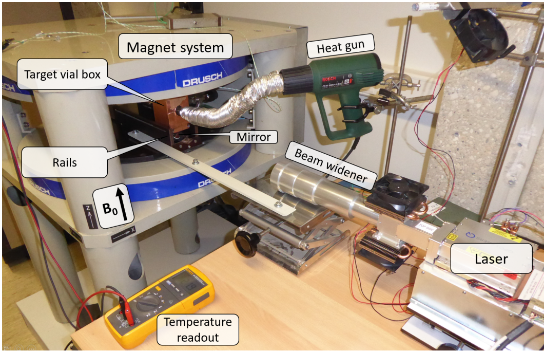
FIGURE 6.1: Overview photo of our gamma-MRI setup. Visible on the right is the diode laser for SEOP pumping, mounted on a cooling unit. It is directly coupled to a beam widener which appears on the picture as a incrementally widening aluminum tube. The laser beam is reflected upwards by a mirror under the target vial, which is later moved to its polarization position within the MRI magnet system. A conventional heat gun blows hot air through an aluminum hose on the target vial in order to heat it to the required temperature. A multimeter connected to a PT100 temperature sensor measures the temperature of the target vial. The detectors around the measuring position are not visible in this picture, since they are located in the center of the magnet.
