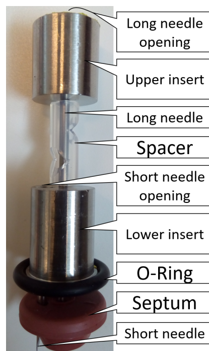
FIGURE 5.5: Manufactured insert for the source container, including the inner O-ring. Needles are still puncturing the septum of the test source vial after a test-run.
