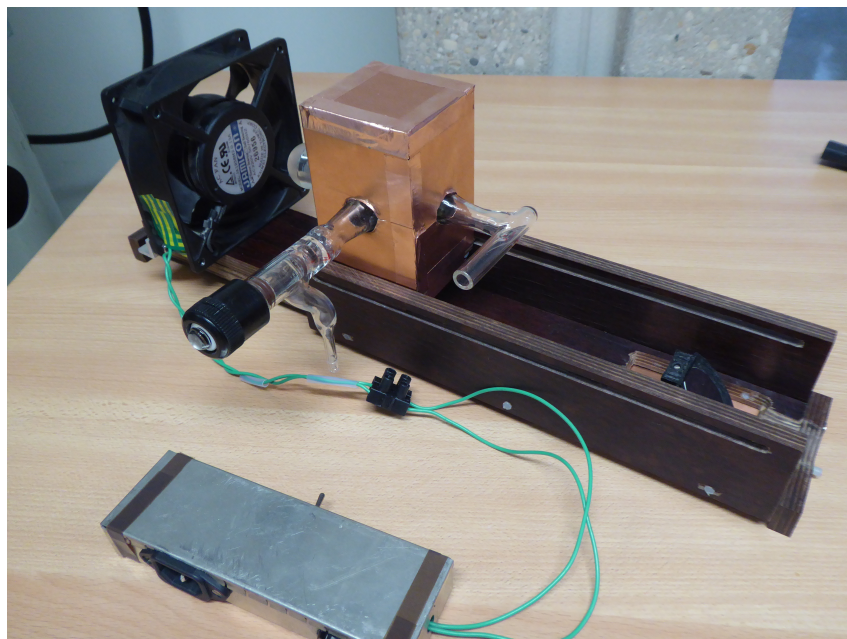
FIGURE 6.4: Rail system with mounted target vial chamber, mirror and cooling fan after its initial assembly in the workshop.
