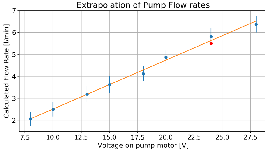
(B) Calculated flow rates generated by the membrane pump. Values are based on the nominal flow rate (red point) and extrapolated based on an acoustic analysis of the motor frequency.
