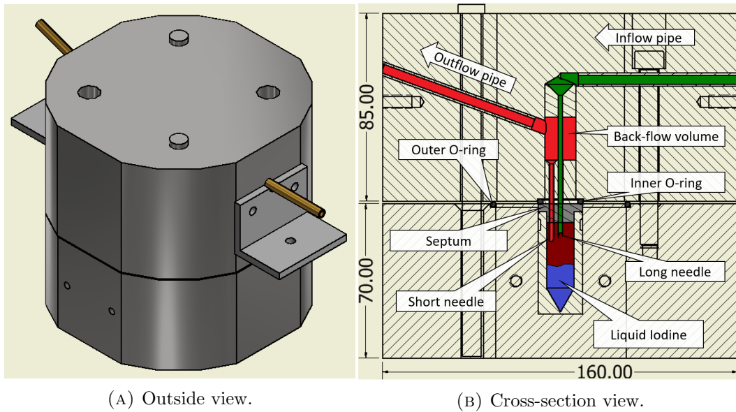
FIGURE 5.4: Final CAD design of the iodine source container. The clean nitrogen gas (indicated in green) enters through the horizontal pipe followed by the long vertical needle. Once enriched with the radioactive trace gases (indicated in red), it exits through the short needle, the back-flow volume and the slanted pipe. Measurements in mm.
