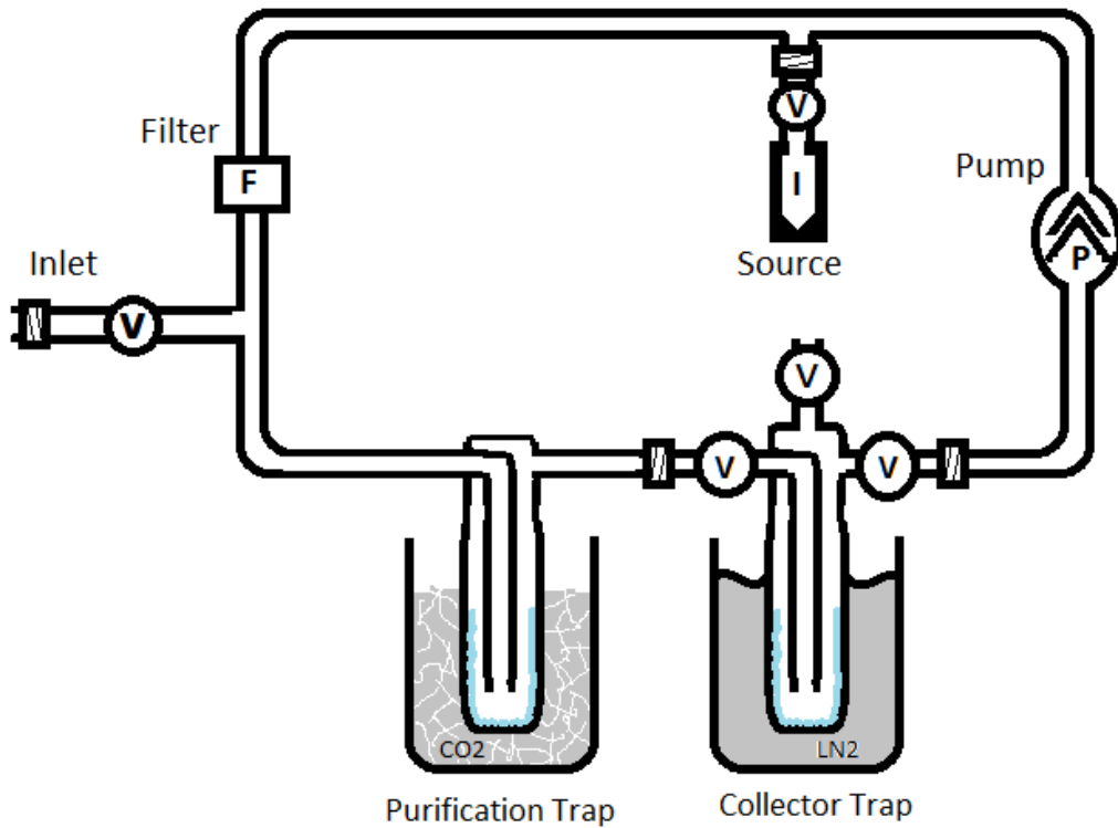
FIGURE 5.2: Concept of the decay loop setup.
