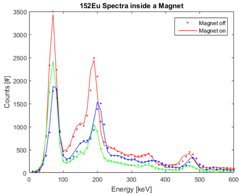
(A) Spectra of all three detectors, each plotted in one color (red, green and blue) using lines and dots, representing a measurement within and without the magnetic field, respectively.
