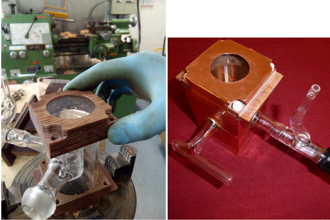
(A) Target vial chamber during manufacturing.
