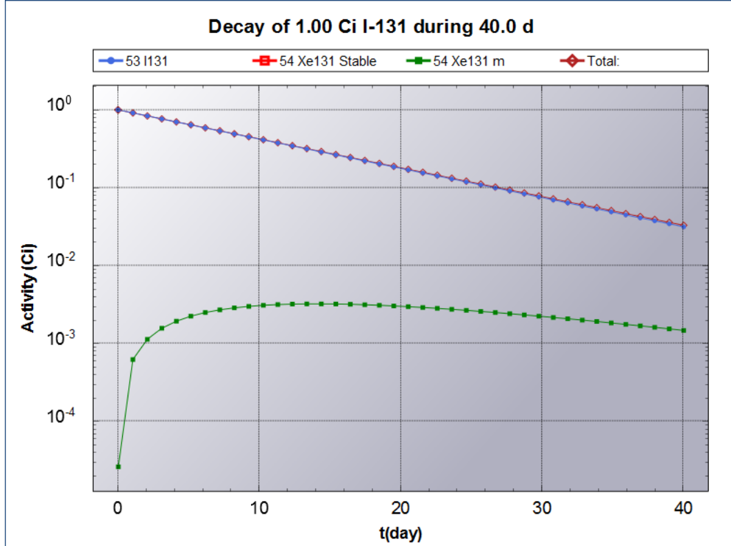
FIGURE 5.8: Decay of 1Ci of ^{131}\text{Iodine} and the produced quantity of ^{131m}\text{Xe} , calculated using the decay engine software of Nucleonica.
