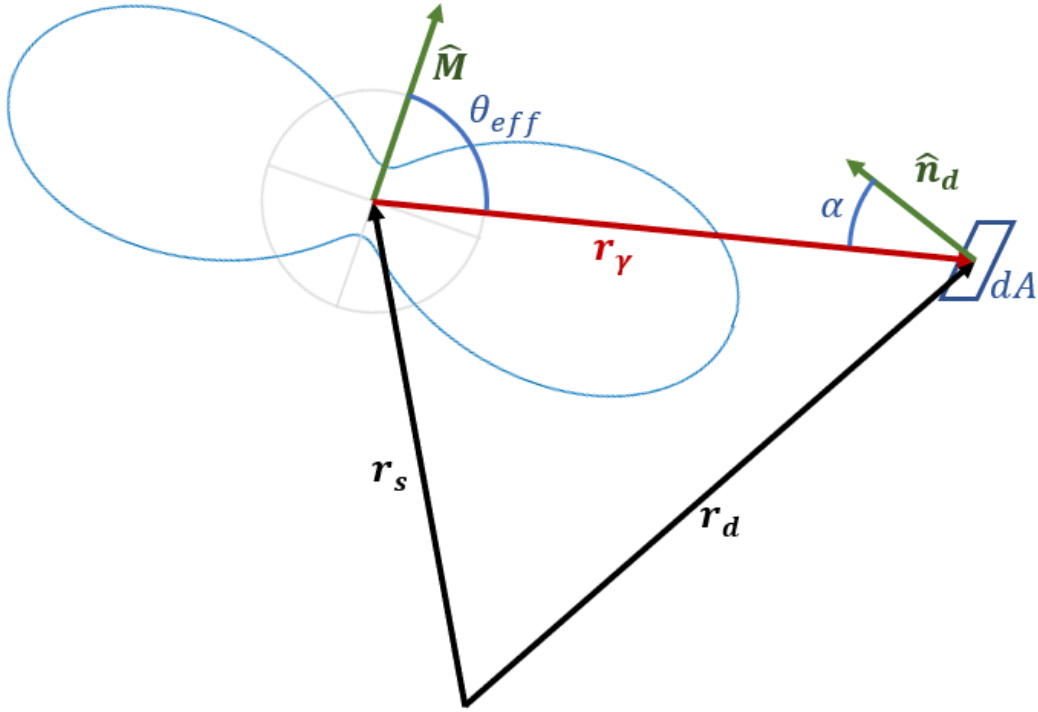
FIGURE 3.2: Illustration of point-sized polarized sample and its relation to a detector element.
