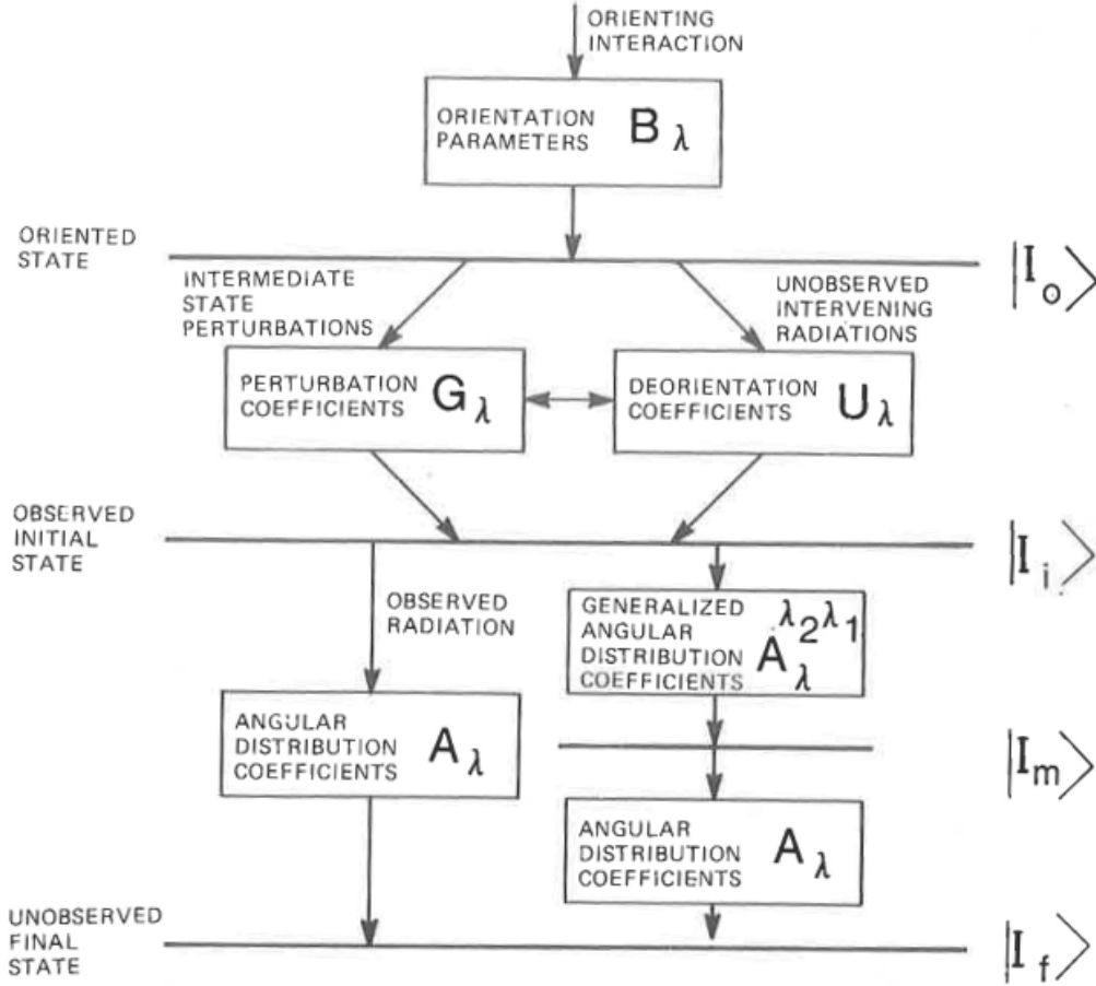
FIGURE 2.1: Illustration of the different parameters necessary for describing radiation from oriented nuclei. Adapted from [2], Chapter 2: Nuclear Orientation Formalism by K.S. Krane.
