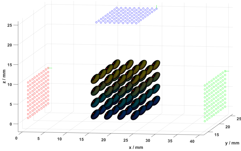
FIGURE 4.2: Plot of a simple gamma-MRI simulation. In this example, three detectors with each 10x10 sensors are located around a sample of 4x4x4 voxels, each represented by a red vector indicating its direction of magnetization and a surface plot visualizing the directional distribution of its radiation, just like in figure 2.2b. The ray vectors are not visible in the plot, but one ray connects each voxel to each sensor.
