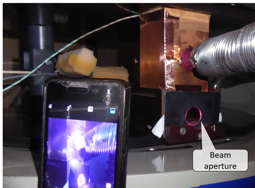
FIGURE 6.7: Photo of the chamber during laser operation. The infrared radiation appears as a weak purple in the main photo, but as a bright blue-white on the smartphone camera.
