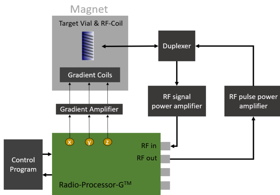
FIGURE 6.11: Simplified scheme of the RF architecture for the gamma-MRI setup.
