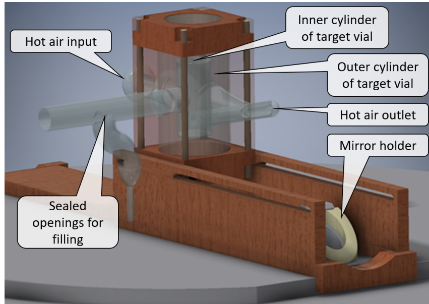
(B) CAD-drawing, showing the box in "measuring position". The copper casing of the target vial box is set to transparent to show the inner design. The holder for the laser mirror is visible on the right.
