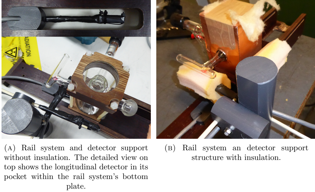
FIGURE 6.8: Rail system in measurement position and detectors, both with and without insulation, set up outside the magnet to allow a clear view.
