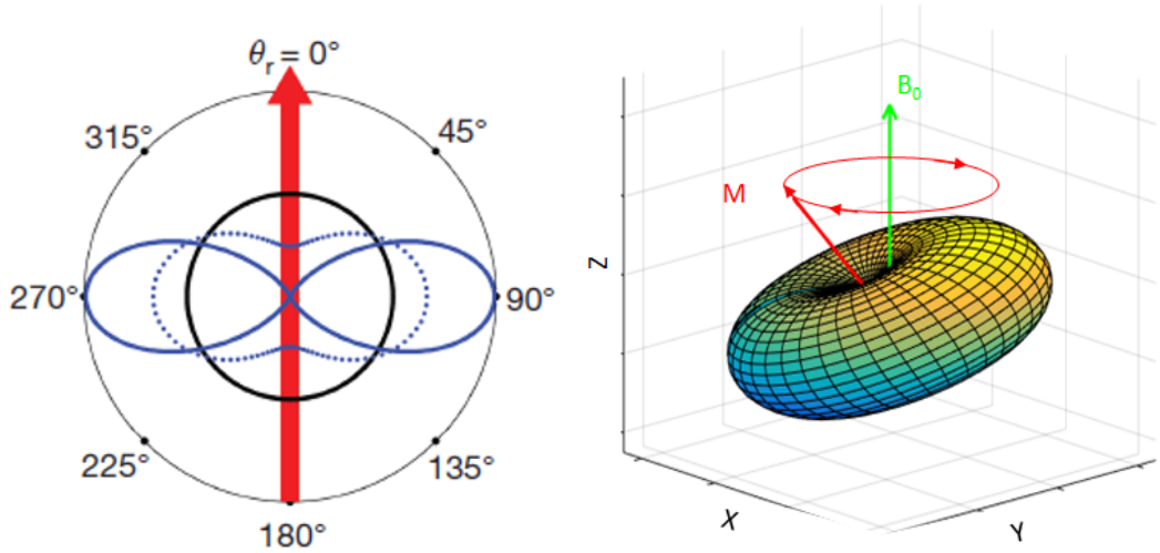
(B) A three-dimensional plot of the expected gamma anisotropy of a nucleus that precesses around the magnetic field axis B_0 after an RF pulse, as will be described in section 2.2.1.1.
