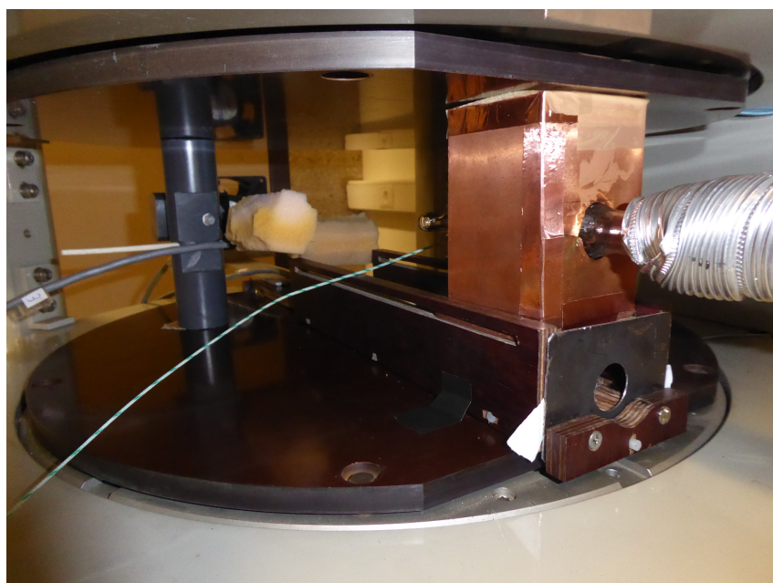
FIGURE 6.5: Complete rail system, detectors and target vial chamber in polarization position within the magnet.
