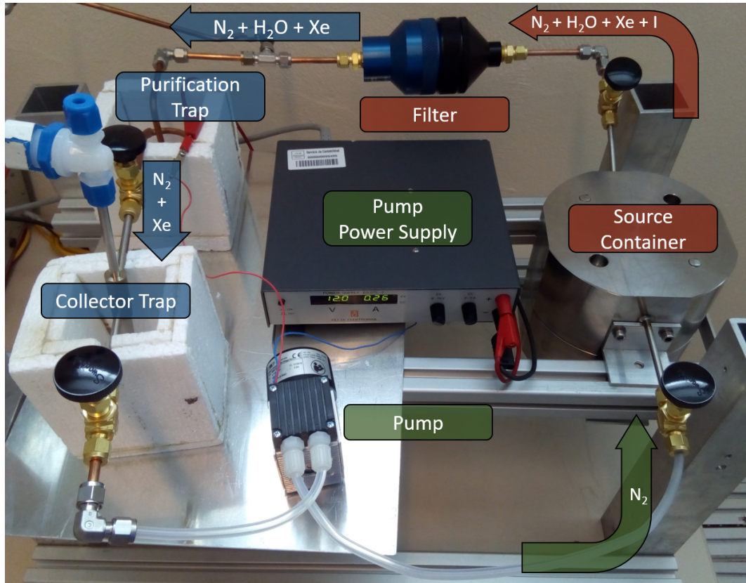
FIGURE 5.3: Foto of the assembled decay setup with component names. The flowing gas mixture is indicated in the arrows. Note that all gases but the nitrogen are only present in trace quantities.
