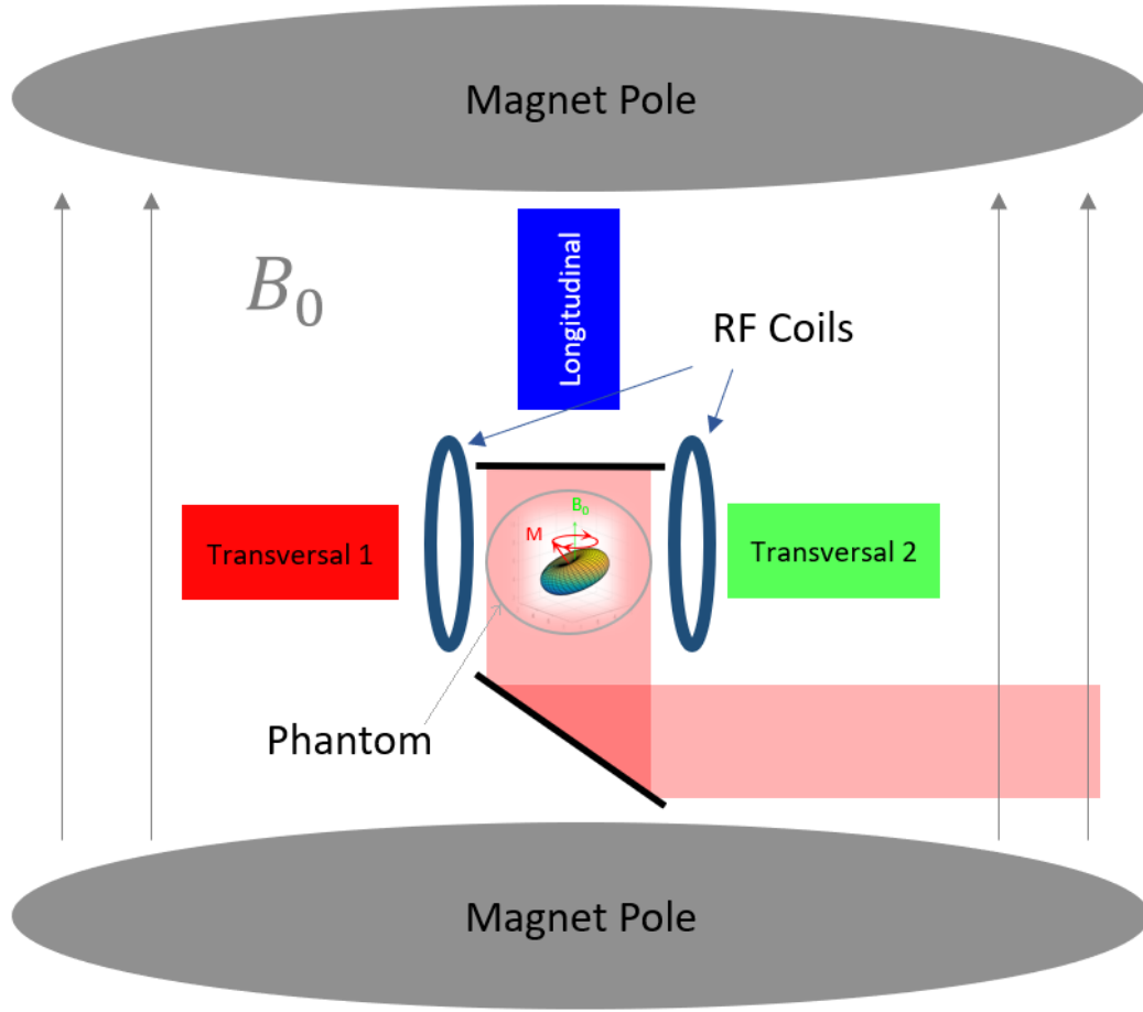
FIGURE 3.1: Simplified schematics of a gamma-MRI setup. Gradient coils are omitted for simplicity.
