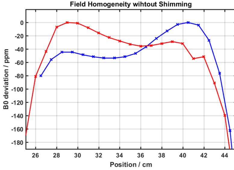
FIGURE 6.6: Measured magnet field homogeneity in the central x (blue) and y (red) axis. The central value of the x-axis was measured at 1.001054T , while the center of the y-axis was at 1.000852T
