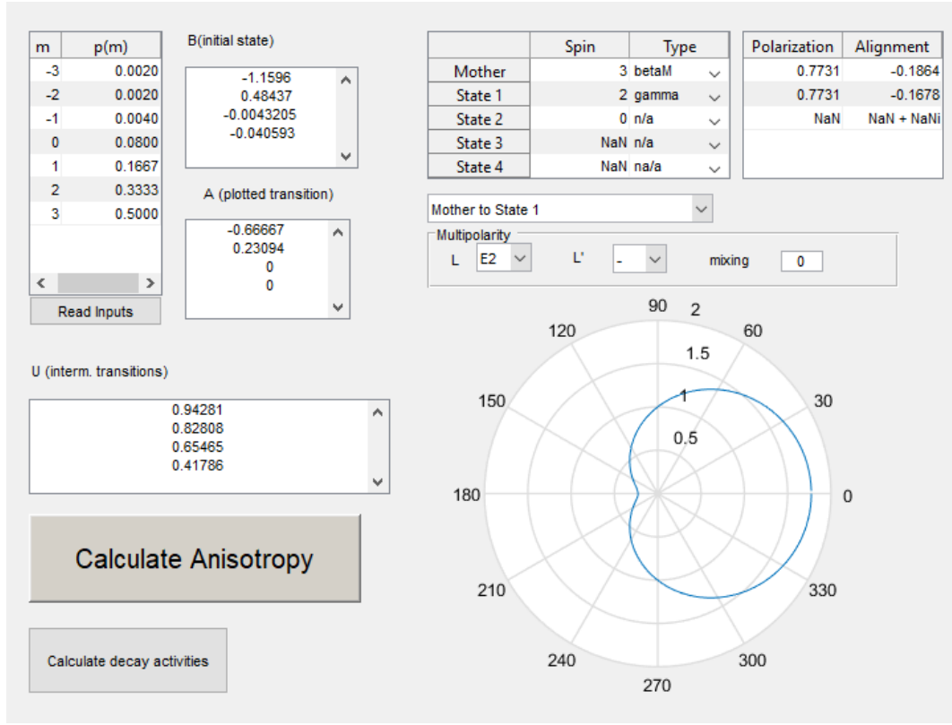
FIGURE 4.1: Graphical interface of the anisotropy tool. The values describe a strongly polarized nucleus with I = 3 , decaying in a \beta^- -decay to a I = 2 nucleus, which in turn emits a gamma-photon while dropping to I = 0 . The dropdown-menu selection causes the polar plot to display the angular distribution of the initial \beta^- -decay.
