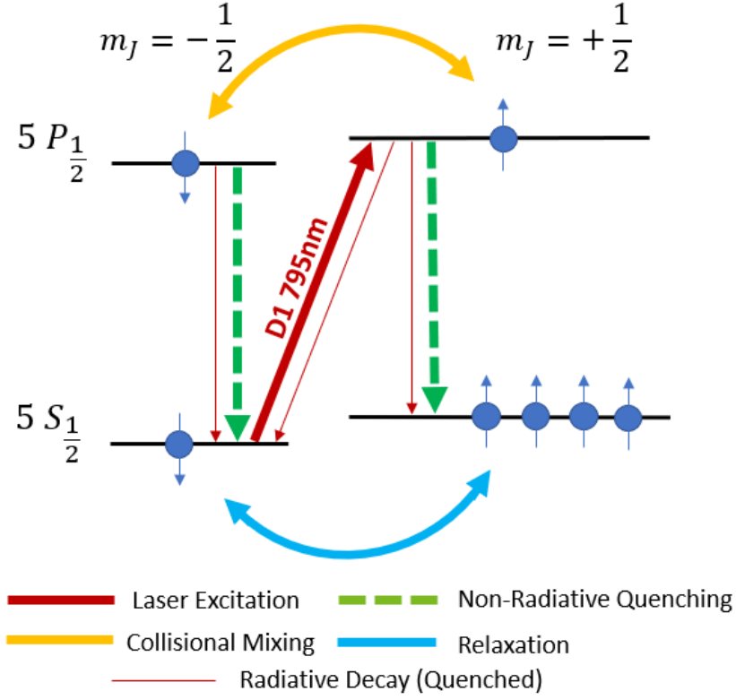
FIGURE 2.4: Illustration of the state transitions of rubidium atoms due to different processes during SEOP.
