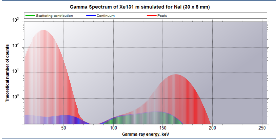
FIGURE 6.10: Simulated Spectrum of 1MBq ^{131m}\text{Xe} in 5cm distance to a NaI detector.
