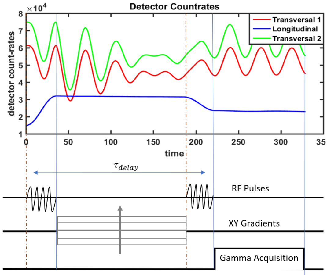
FIGURE 3.3: Detector count-rates during a CMZ-pulse sequence, as calculated with the gamma-MRI simulation software discussed in section 4.2.
