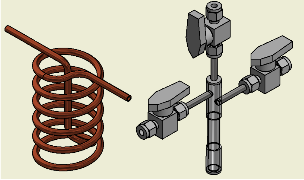
FIGURE 5.7: Design of purification trap (left) and collector trap (right) for the xenon extraction setup.
