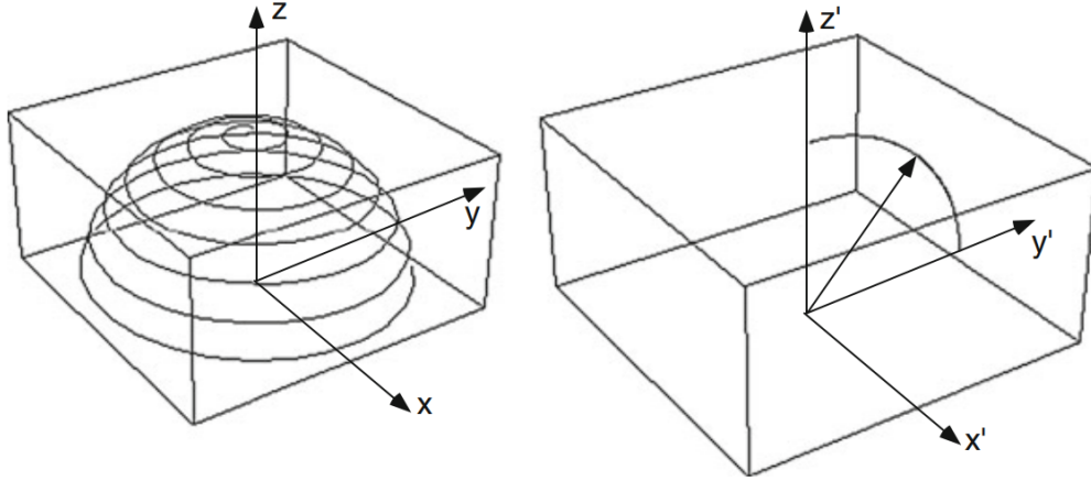
FIGURE 2.3: Motion of the magnetization vector \mathbf{M} under the influence of the rotating magnetic field B_1 . The left side shows the laboratory coordinate system and the right side the rotating coordinate system. Figure adapted from [3].
