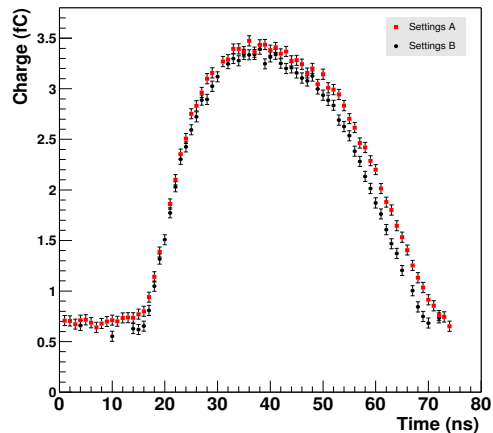
Figure 9.9: Pulse shapes for the two front-end setting configurations A and B , for the full-dose irradiated end-cap module K5 308: it is visible the better timing response in case of higher analogue voltage.
