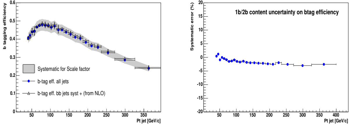
Figure 4.25: Effect of changing the double b content on the inclusive b tagging efficiency (on the left). The resulting uncertainty on the cross section is less than 2% on the whole transverse momentum spectrum (on the right).
