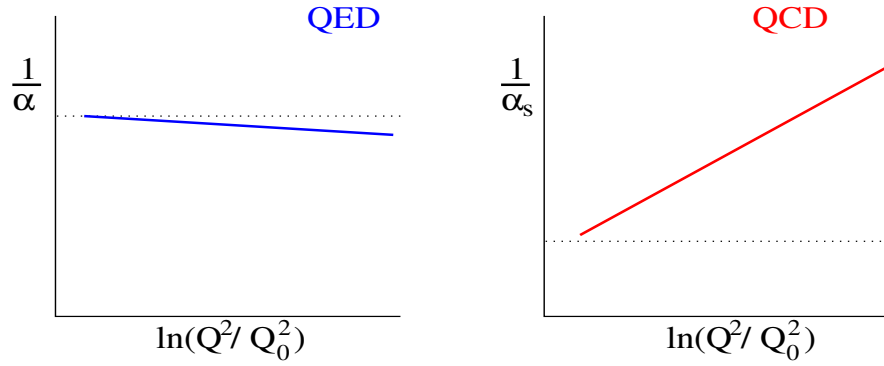
Figure 1.2: Reciprocal of the running coupling constant as function of Q^2 , for (left) QED, and (right) QCD.
