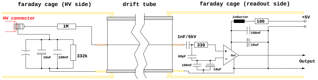
Figure 4.10: Electronics on the high voltage side (left) and readout side (right) of a single drift tube. The circuits on both sides are surrounded by a Faraday cage made of brass.
