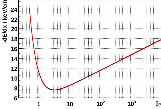
Figure 2.2: Qualitative progression of the Bethe-Bloch formula Eq. 2.2. At \beta\gamma \approx 3 \dots 4 a minimum is obtained. The curve shown here was calculated for argon at 3 bar and a charge of the incident particle of Q = \pm 1 .
