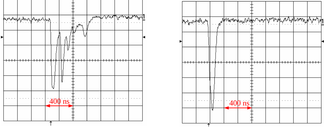
Figure 2.5: Signals in a MDT, generated by a muon ( left ) and by a photon with E \approx 22 keV ( right ) from a ^{109}\text{Cd} source. The muon signal shows several peaks from different clusters along the track. The photon signal shows only a single peak due to the localized primary ionization. The pictures were taken from [25].
