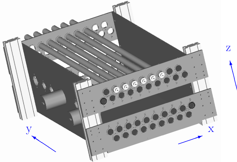
Figure 4.1: Rendered image of the mechanical setup: The strong ^{241}\text{Am} sources could be inserted from the left. During pulse height measurements they were pulled out of the box; then they were completely covered by thick brass cylinders (two of them can be seen on the left side). The axes of the coordinate system, shown in blue, are used throughout the following chapters.
