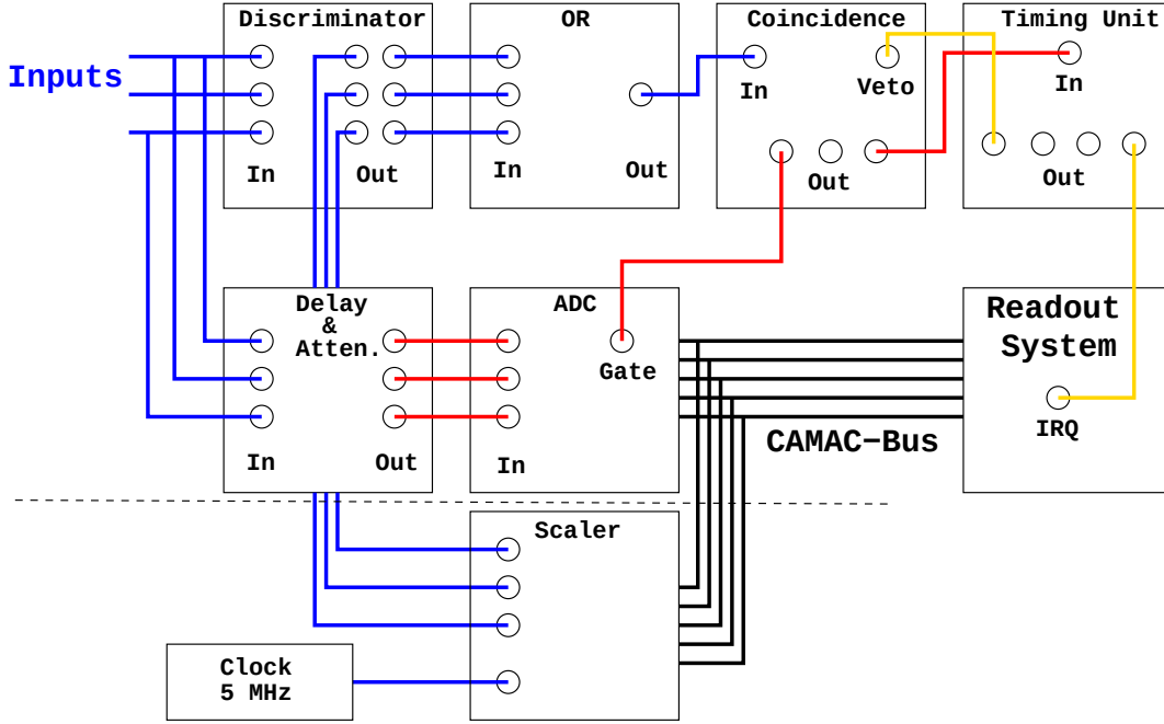
Figure 4.11: Time-to-colour coded readout cycle for pulse height scans. The colour code has to be read in the following order: blue, red, orange, black. The readout system (realized with two computers, see Fig. 4.12 and section 4.1.4) on the lower right side of the scheme is the end of the cycle. The part below the dotted line belongs to the slow control system and is only shown for the sake of completeness.
