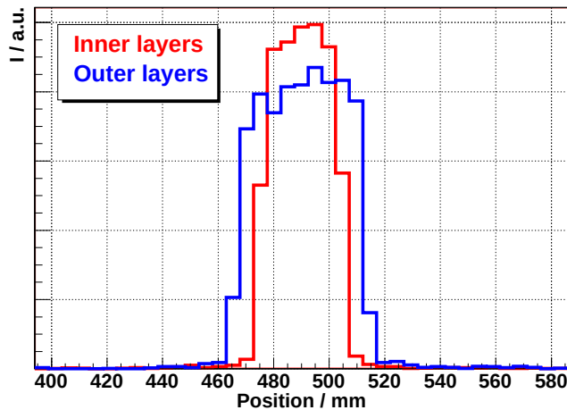
Figure 5.14: Length of the scanned section along the tube in pulse height scans as result of the MC simulation. For the tubes in the inner (outer) two layers a length of \approx 3 ( 4.5 ) cm is retrieved. This is in good agreement with a simple geometrical estimation.
