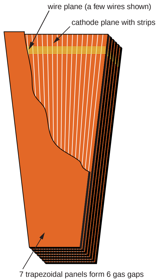
Figure 2.21: Schematic view of a CSC chamber.
