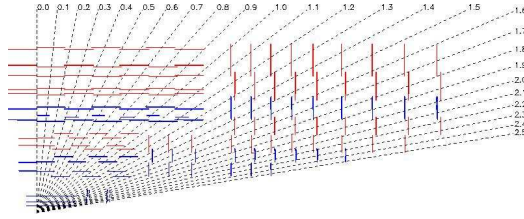
Figure 2.9: Longitudinal view of one quarter of the CMS silicon strip tracking system. The red lines are modules composed of one detector only, the blue lines are detectors composed of two modules.
