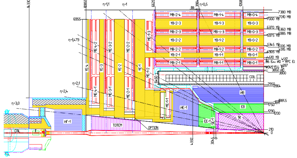
Figure 2.5: One quarter longitudinal view of the CMS Experiment. Dimensions are in units of mm.
