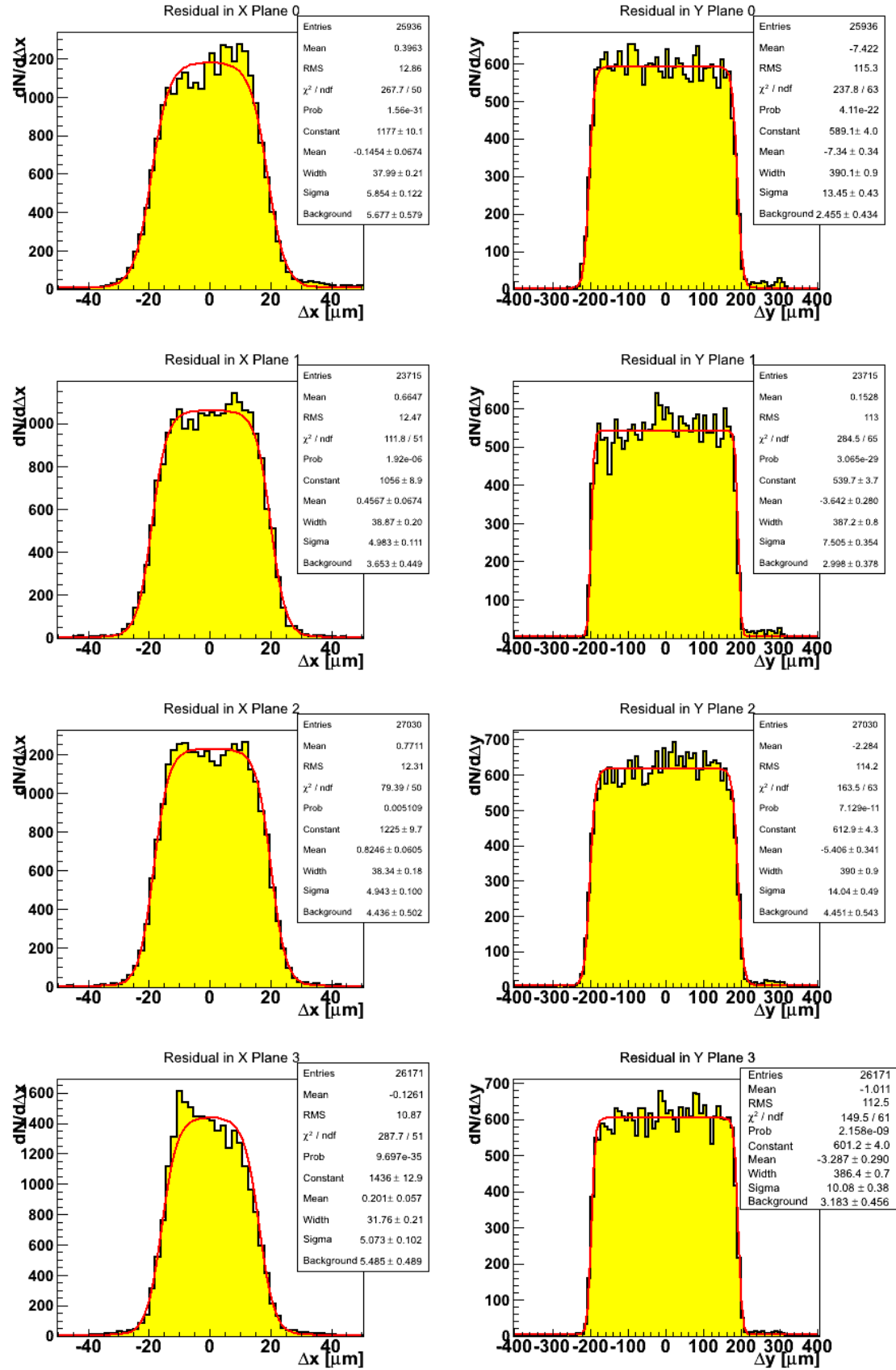
Figure B.2.: Unbiased residuals of DUTs 0-3. The track fitting was done using the EUDET telescope planes. Only five planes out of six are used for track fitting. The data from the DUTs are not used for fitting. The underlying data is the run 11250 of the July 2010 testbeam at CERN
