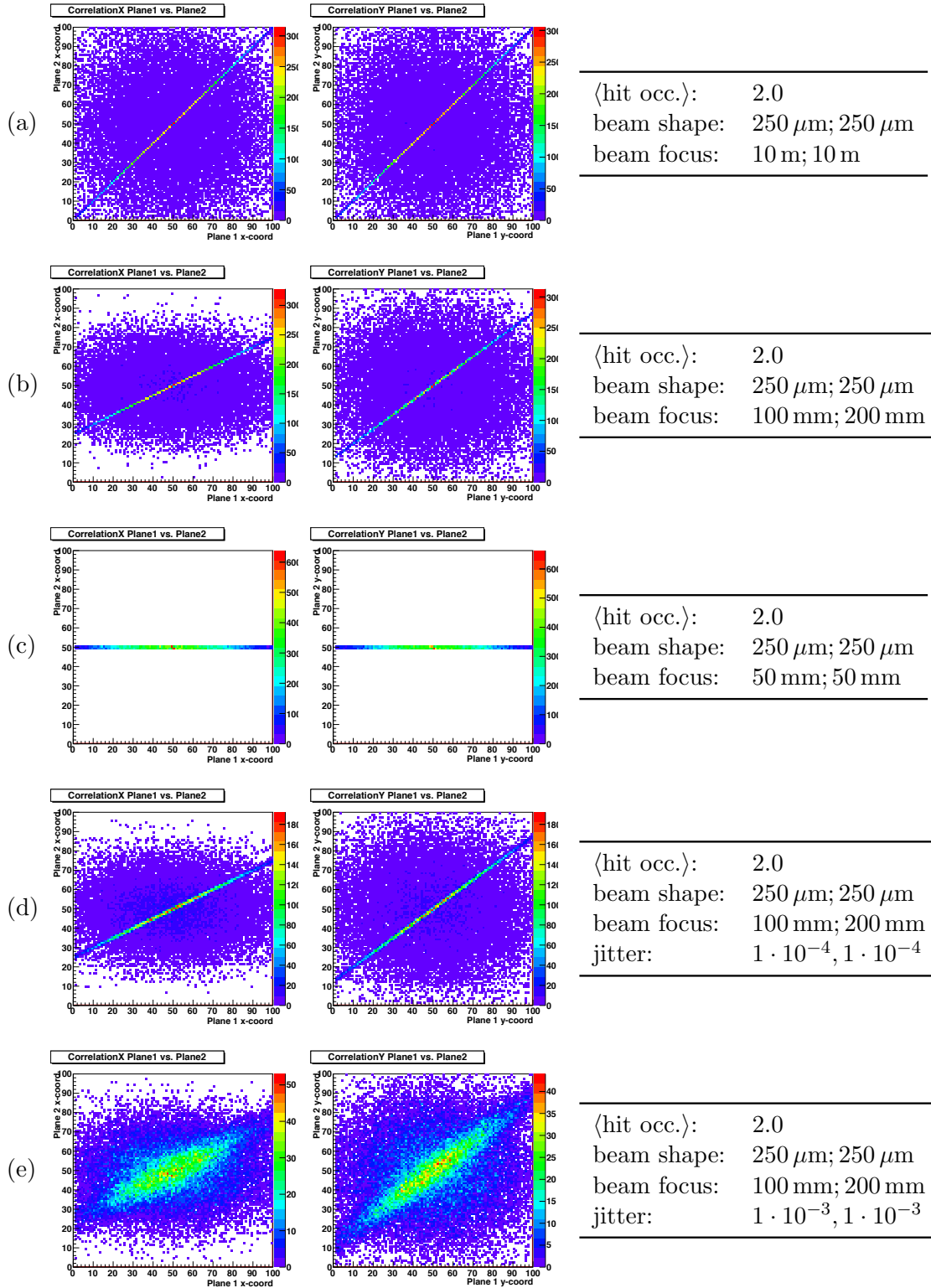
Figure 9.8.: Simulated correlations. The illustration shows the influence of different beam-focus points and jitter on the correlations. In the cases (a) to (c) all tracks are exactly focussed without jitter. (d) and (e) use the focus-setting of case (b) by applying jitter. In case (b) the focus-point of the beam in both directions is exactly in the second sensor. The distance between the simulated sensors is 50 mm. The number of event, used for the simulation is 10 000
