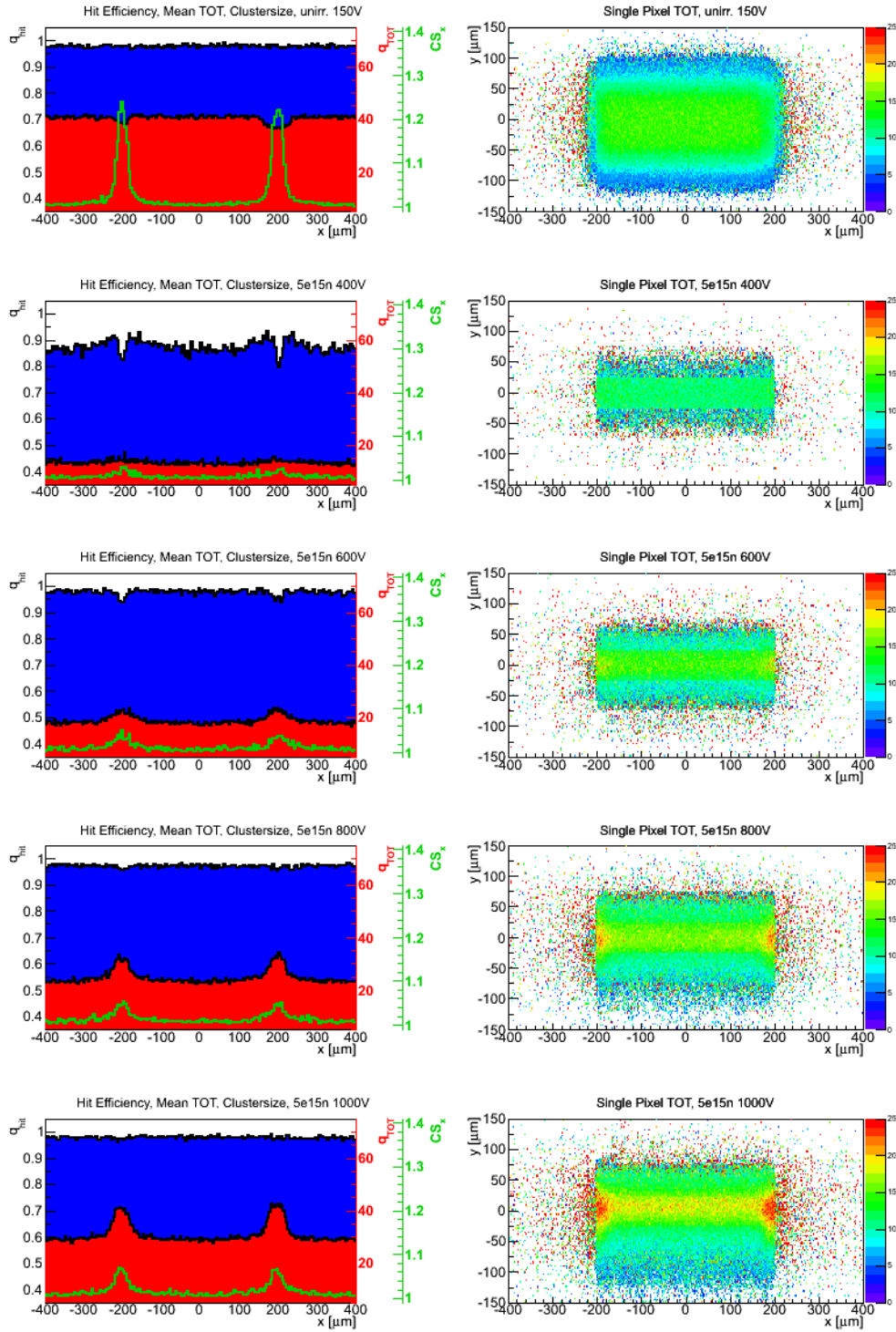
Figure 13.19.: Left: Subpixel hit efficiency (blue), mean TOT (red) and the mean cluster size in x (green) as a function of the incidence point in x (different scales) for an unirradiated sensor (1) and 5 \cdot 10^{15} \text{ n}_{\text{eq}} \text{ cm}^{-2} with neutrons (2) to (5) at an incidence angle of \varphi = 30^\circ . Right: Mean TOT of a single pixel in dependency of the incidence position. As the incidence angle is \varphi = 30^\circ , an incidence point at lower y -values hits the pixel only in its lower region
