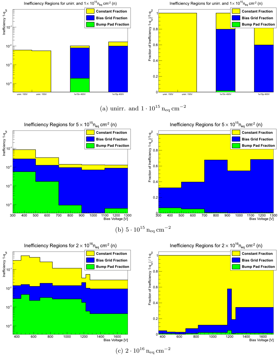
Figure 13.13.: Stacked histograms illustrating inefficiencies caused by the pixel gap at the bump pad region (green), the pixel gap at the bias grid region (blue) and a constant inefficiency of the whole sensor (yellow). The plots on the left show the absolute magnitude of inefficiency and those on the right show the respective relative fractions of the inefficiency
