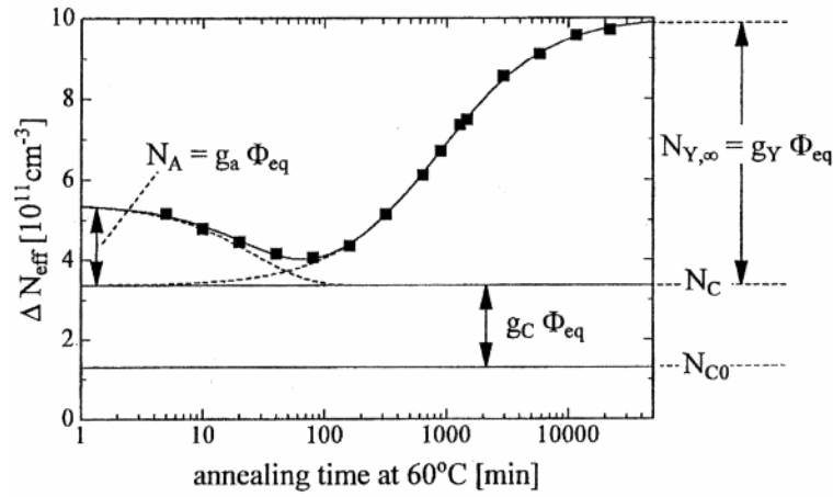
Figure 3.5.: Diagram illustrating the time dependency of the annealing behaviour by showing the effective doping concentration vs. the time at a fixed temperature of 60 °C. The measured points are taken with a diode structure of 25 kΩ cm after an irradiation of 1.4 \cdot 10^{13} \text{ n}_{\text{eq}} \text{ cm}^{-2} [58]
