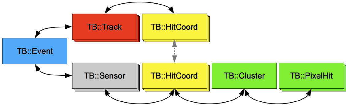
Figure 10.5.: Illustration of the object oriented TB::Event object and its children
