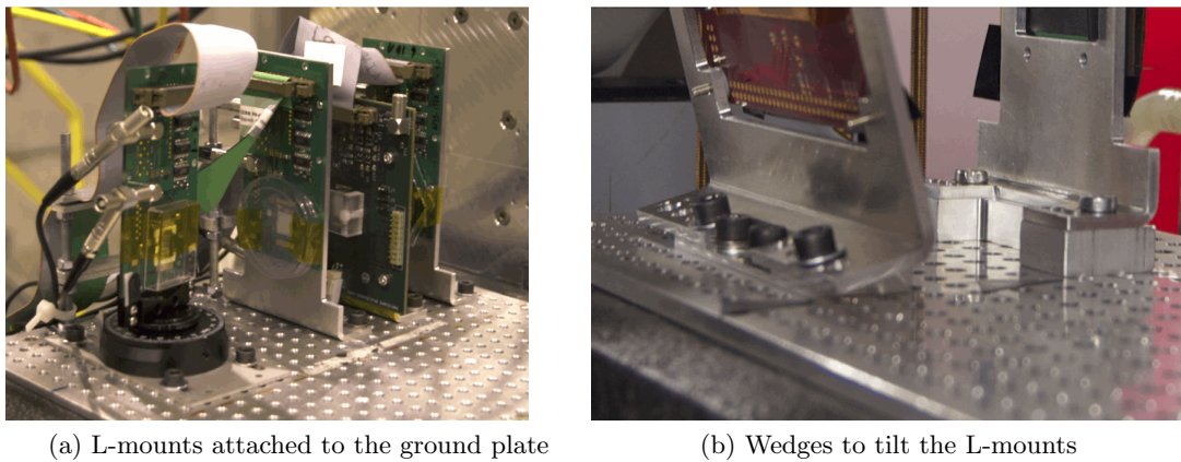
Figure 7.11.: Photograph of the L-Mounts with SCAs attached to the DOBOX. Wedges are used to tilt the L-mounts.
