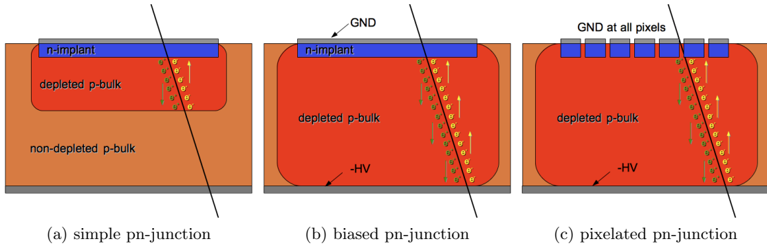
Figure 3.2.: Working principle of (a) a simple non-biased sensor diode, (b) a depleted sensor diode and (c) a pixelated sensor. Particle tracks and the production of electron hole pairs are visualised as well
