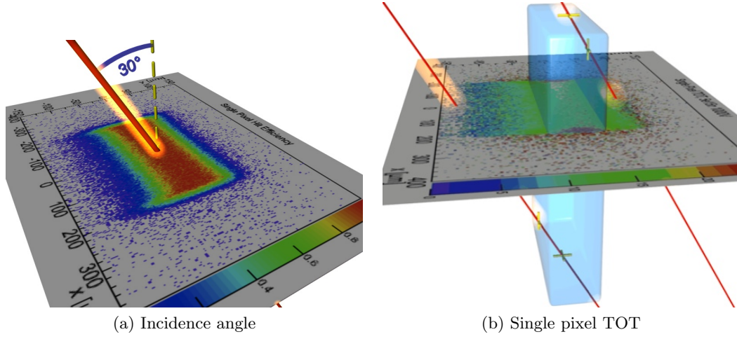
Figure 13.16.: Computer aided illustration to explain (a) the incidence direction in the plots shown in figure 13.15, (b) the meaning of the single pixel TOT illustration in figure 13.19. The blue box indicates the 3-dimensional volume of a pixel
