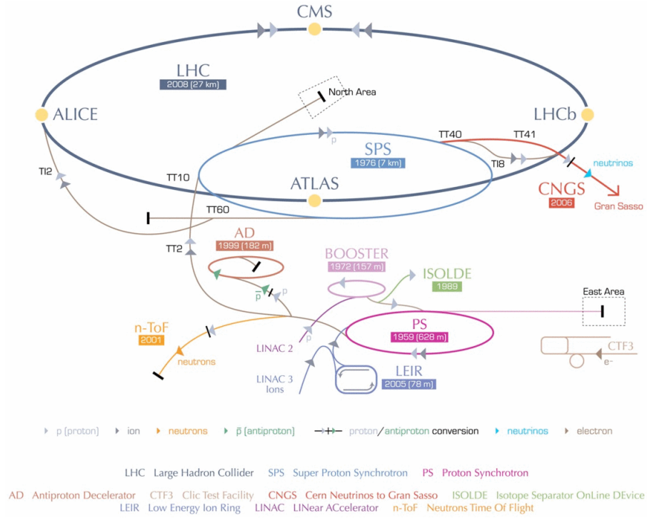
Figure 2.1.: Schematical illustration of CERN's accelerator complex [14]
