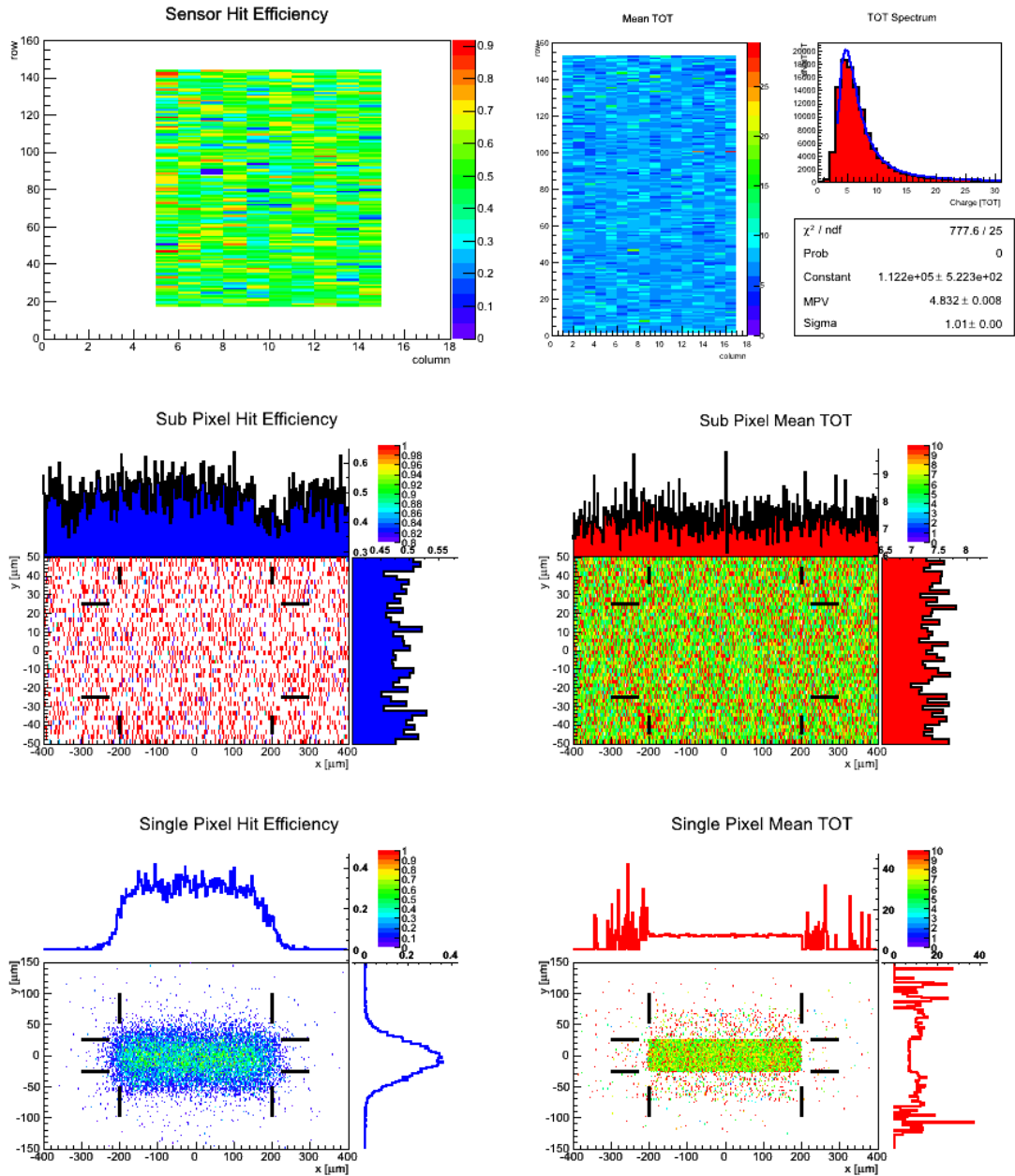
Figure C.11.: Sensor overview of sensor DO10 irradiated to \Phi_{\text{eq}} = 2 \cdot 10^{16} \text{ n}_{\text{eq}} \text{ cm}^{-2} with neutrons, running at 500 V
