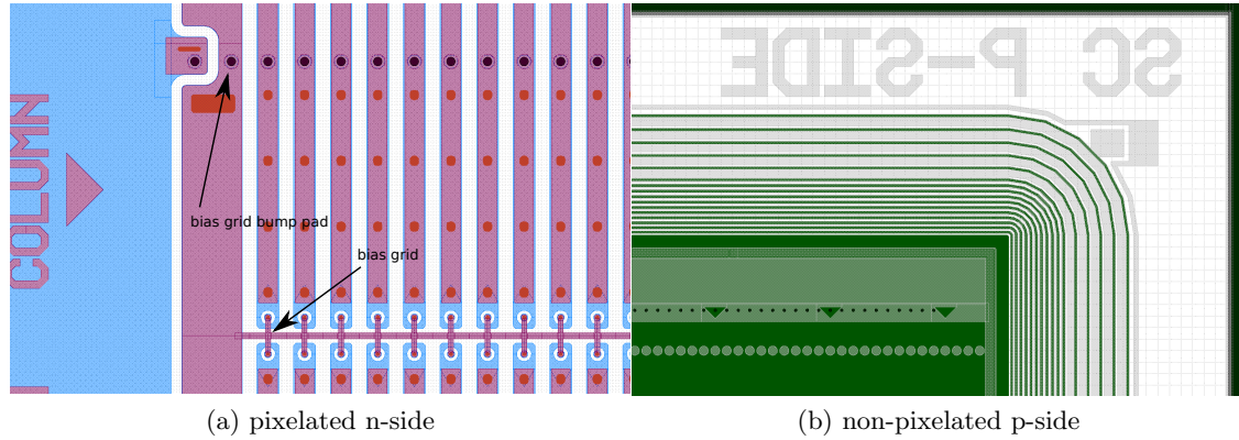
Figure 4.3.: Computer aided drawing of the sensor design. In (a) one can see the rectangular pixels, the bump bond contact pads and the bias grid. (b) shows the edge of the sensor's backside with the guard rings [73]
