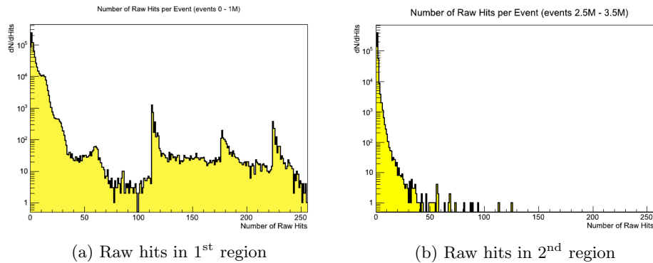
Figure 12.6.: Explanation for the Efficiency Puzzle. The two regions visualized in figure 12.5b are shown in (a) and (b). The data used here are the runs 11193 to 11282 of July 2010
