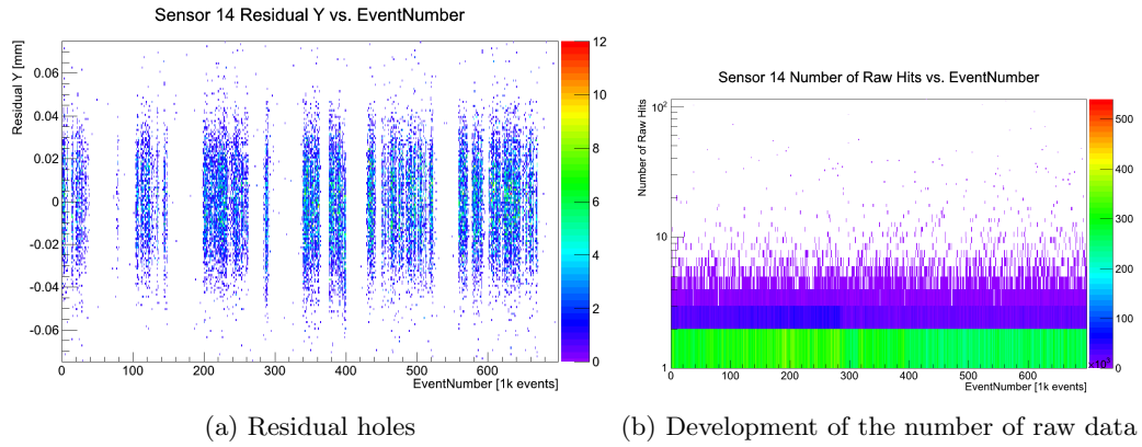
Figure 12.7.: (a) Development of the residual of y and (b) the number of raw hits of DO13. The matching algorithm cannot calculate the residuals interrimly, which leads to the residual holes
