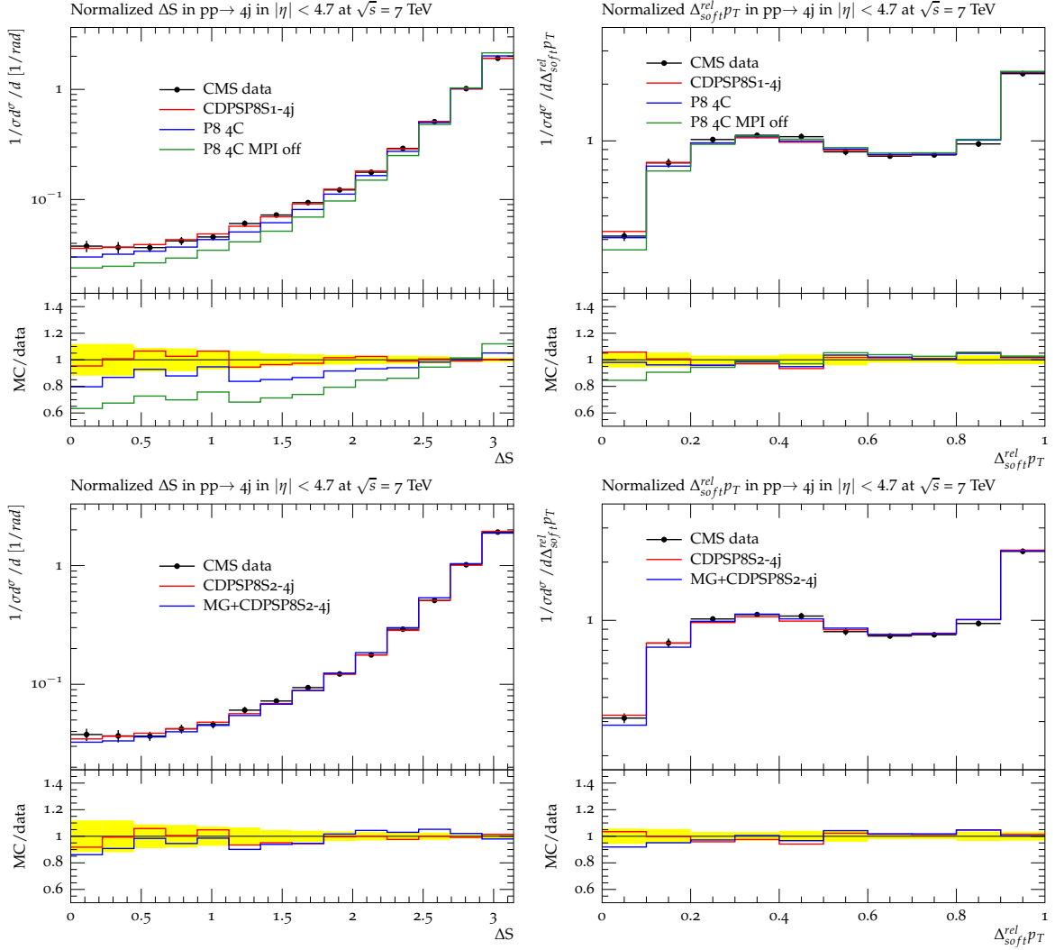
Figure 13: CMS data on the normalized distributions of the correlation observables \Delta S (left) and \Delta^{\text{rel}} p_T (right) measured in 4-jet production compared with PYTHIA 8 Tune 4C, Tune 4C with no MPI, and the new PYTHIA 8 partial tune (top row) and compared with the new PYTHIA 8 tune and with MG interfaced with the new full tune (bottom row). Also shows the ratio of the tunes with the data.
