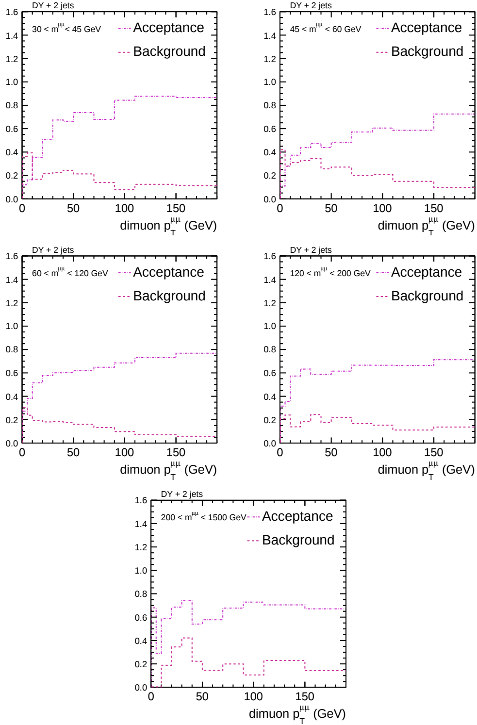
Figure D.5: Background and acceptance for DY + 2 \text{ jets} transverse momentum distribution p_T^{\mu\mu} in bins of the dimuon mass.
