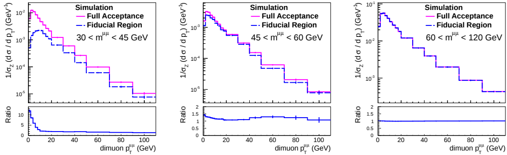
Figure 4.16: Dimuon p_T^{\mu\mu} distribution comparing the fiducial region ( |\eta^\mu| < 2.1 and p_T > 20 (10) GeV) and the full acceptance. The effect of an acceptance correction is presented for three invariant mass ranges.
