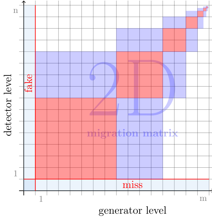
Figure 4.24: Illustration of the unfolding response matrix. Contributions from fake and miss events are considered in the unfolding procedure. The effect of bin migrations is shown in the 2d matrix.
