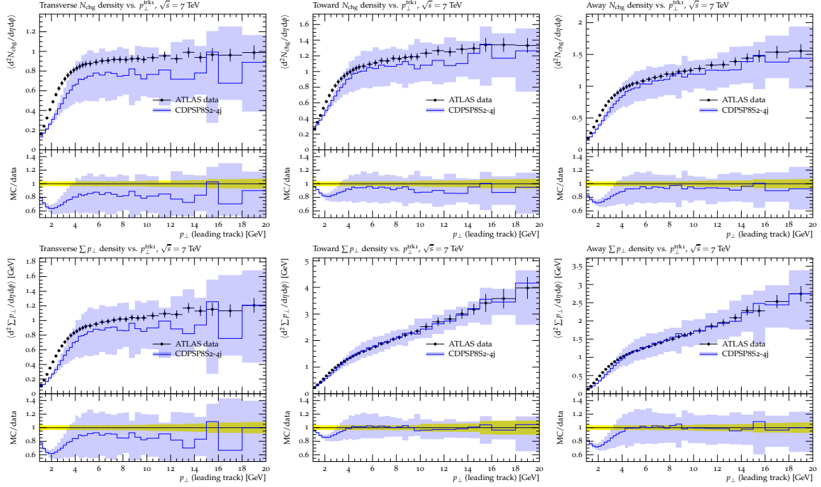
Figure 14: ATLAS data on the charged particle multiplicity N_{ch} (top) and p_T sum (bottom) measured in the transverse (left), toward (center) and away (right) regions compared with CDPSTS2-4j. Also shows the ratio of the tunes with the data and the uncertainties of the predictions based on the Professor eigentunes.
