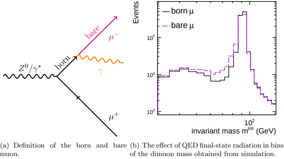
Figure 4.6: An illustration of the definition of the born and bare muons in the final state is shown in (a) and the number of events as a function of the dimuon invariant mass for bare and born muons is presented in (b).
