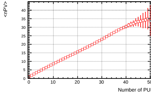
Figure B.1: Average number of reconstructed primary vertices < nPV > as a function of the number of pileup interactions (PUI) in simulation.
