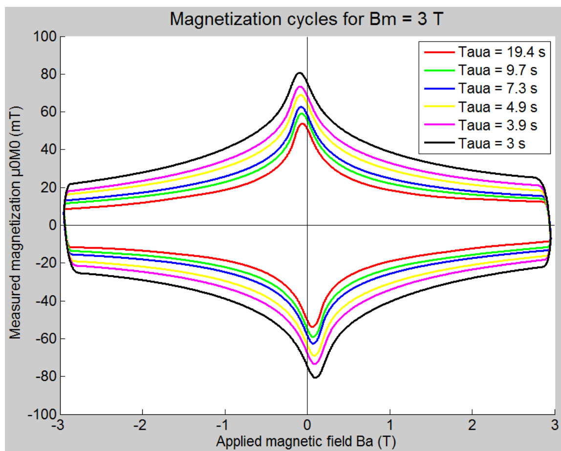
Figure 101 : Magnetization cycles of K006-01C JT-60SA TF strand measured in Speedy facility for trapezoidal cycles with B_m = 3T
