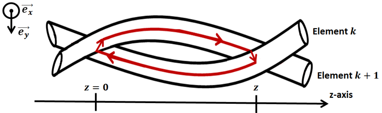
Figure 42 : Scheme showing the integration path of equation (135)
