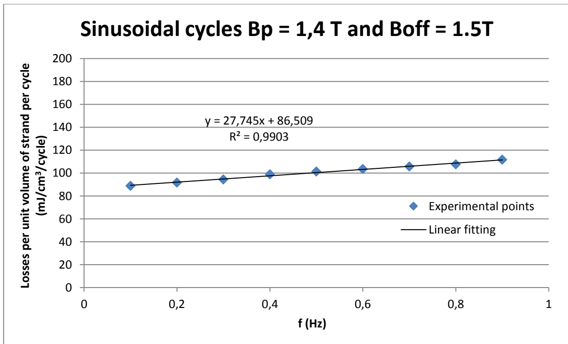
Figure 122 : Losses of F 0796-1 ITER TF strand per unit volume of strand per cycle measured in Speedy facility for sinusoidal cycles with B_p = 1.4\text{ T} and B_{off} = 1.5\text{ T}
