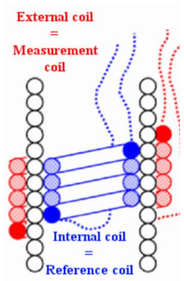
(c) : Schematic view of pick-up coils and composite for assembled holders
