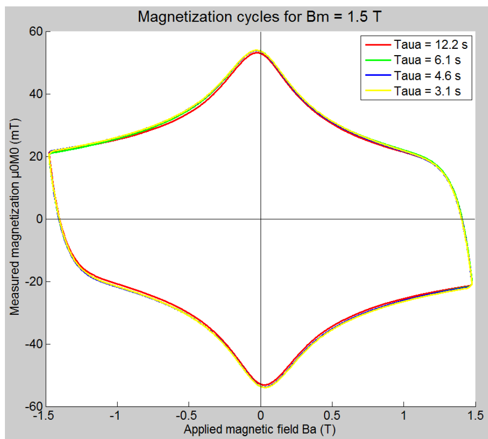
Figure 115 : Magnetization cycles of F 0796-1 ITER TF strand measured in Speedy facility for trapezoidal cycles with B_m = 1.5\text{ T}
