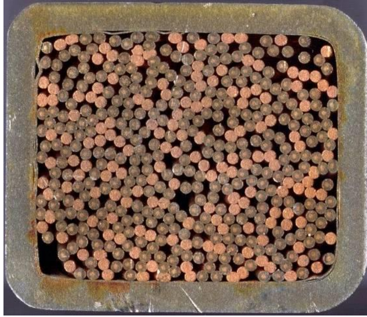
Figure 68 : Photograph of a cross-section of a sample of JT-60SA TF conductor
