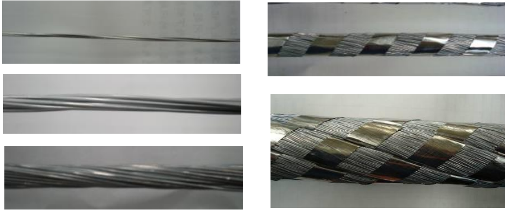
Figure 9 : Examples of successive cabling stages for ITER CICC. Note the addition of wrappings at the 4th stage
