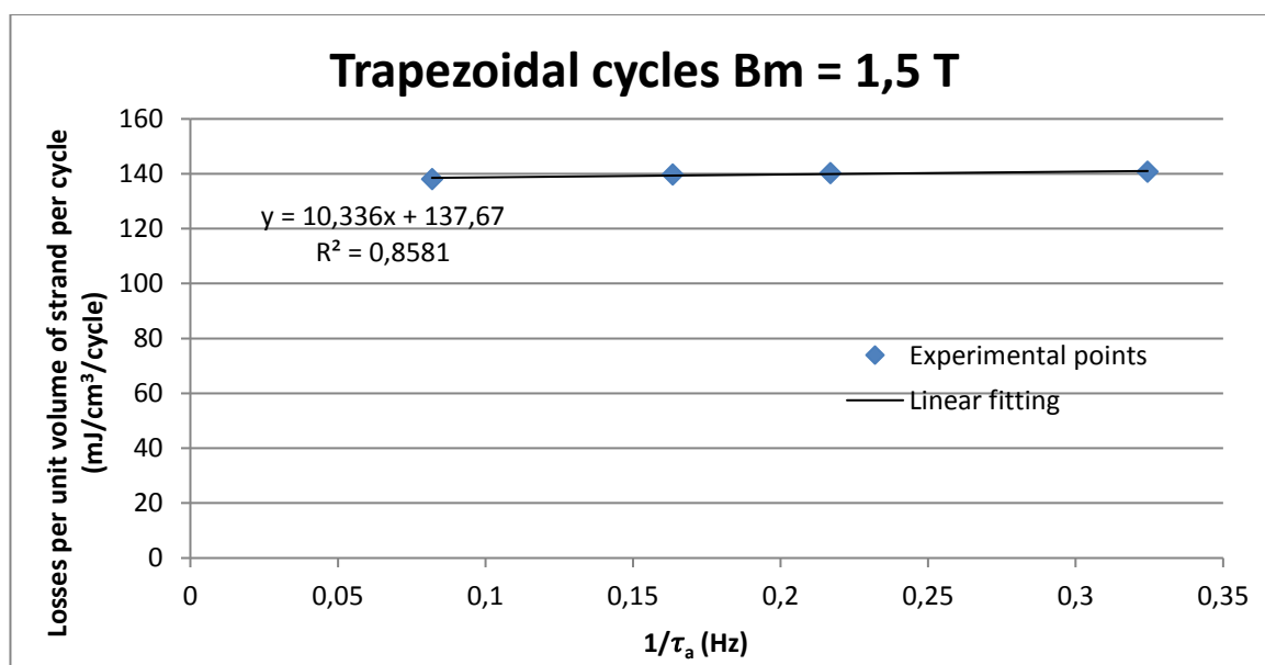
Figure 116 : Losses of F 0796-1 ITER TF strand per unit volume of strand per cycle measured in Speedy facility for trapezoidal cycles with B_m = 1.5\text{ T}
