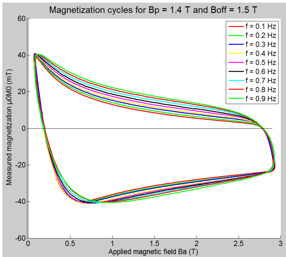
Figure 121 : Magnetization cycles of F 0796-1 ITER TF strand measured in Speedy facility for sinusoidal cycles with B_p = 1.4\text{ T} and B_{off} = 1.5\text{ T}
