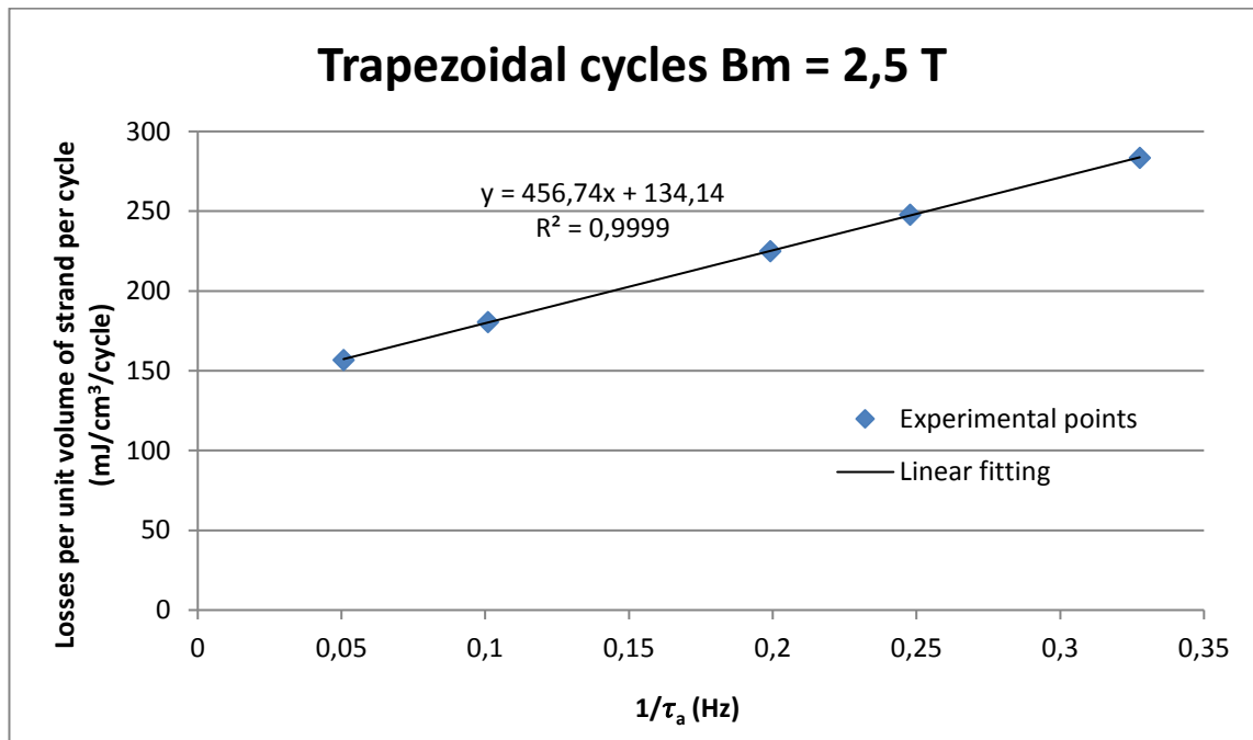
Figure 100 : Losses of K006-01C JT-60SA TF strand per unit volume of strand per cycle measured in Speedy facility for trapezoidal cycles with B_m = 2.5T
