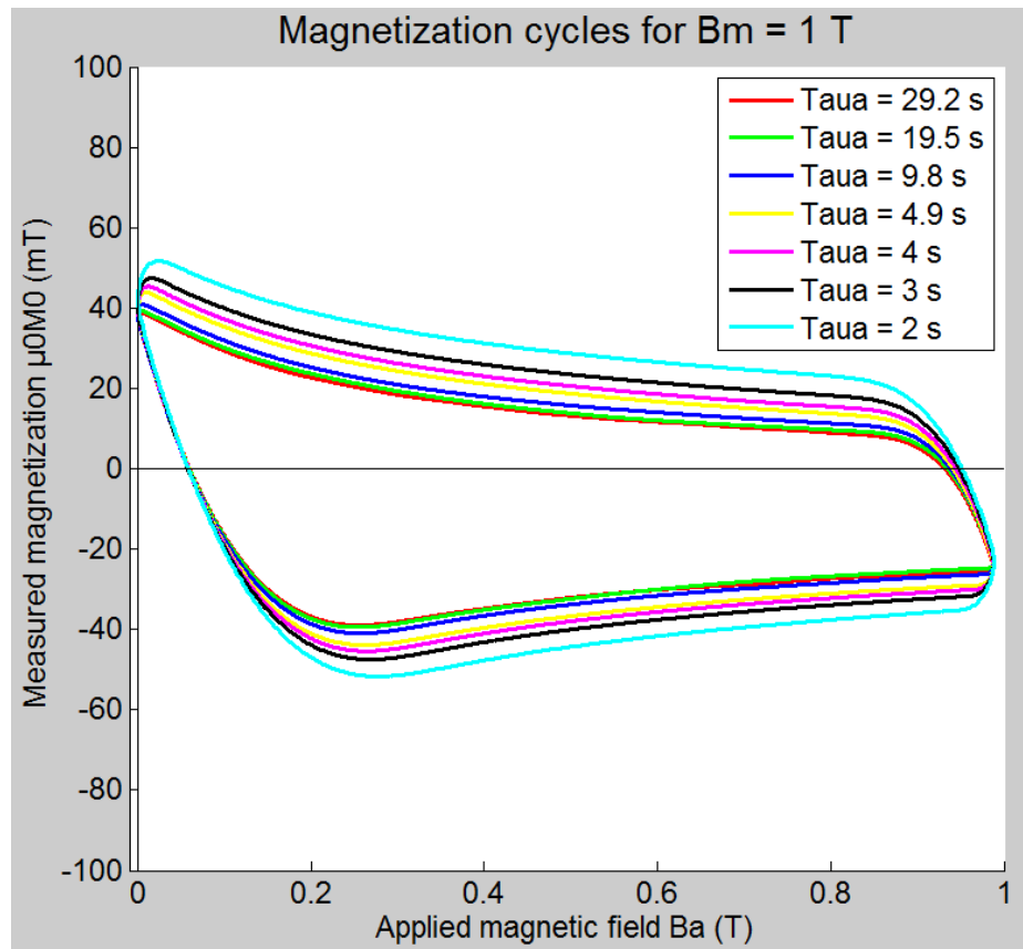
Figure 103 : Magnetization cycles of K006-01C JT-60SA TF strand measured in Speedy facility for positive trapezoidal cycles with B_m = 1T
