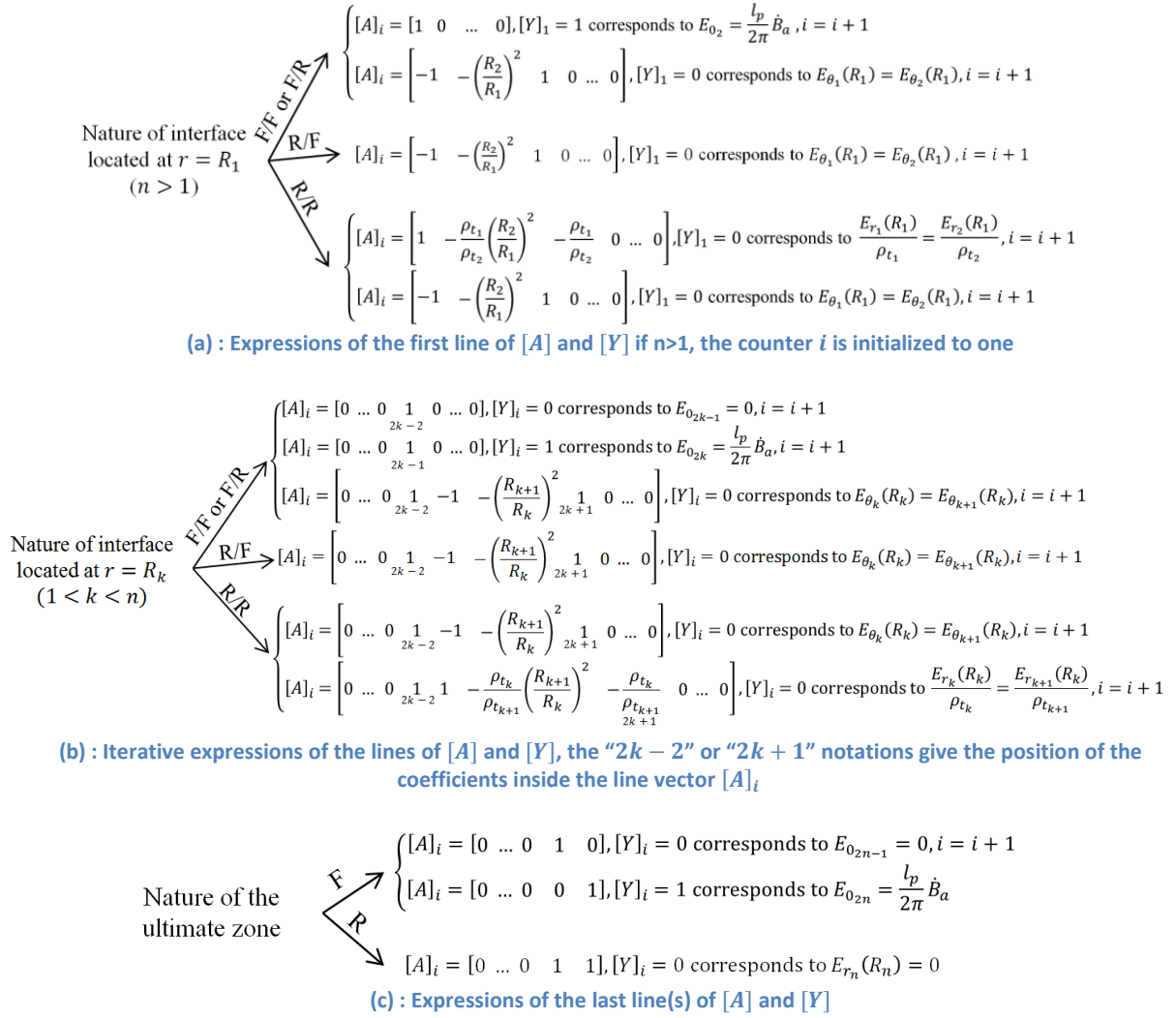
Figure 78 : Logical trees used to build [A] and [Y]
