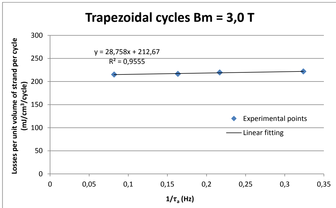
Figure 120 : Losses of F 0796-1 ITER TF strand per unit volume of strand per cycle measured in Speedy facility for trapezoidal cycles with B_m = 3T
