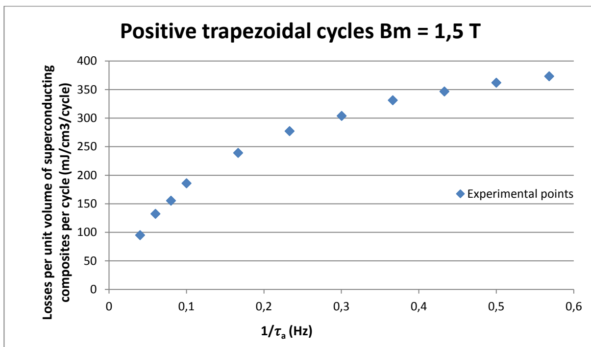
Figure 72 : AC losses of JT-60SA TF conductor per unit volume of superconducting composites per cycle measured in Josefa facility for positive trapezoidal cycles with B_m = 1.5 \text{ T}
