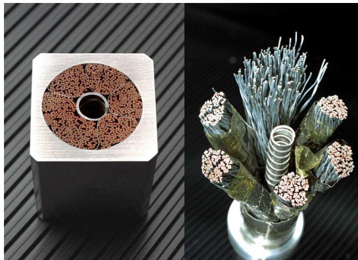
Figure 7 : Two ITER CICC illustrations: (left) view of CS conductor, round cable in square jacket; (right) exploded view of TF Model Coil [4] cable, with wrapped petals and central spiral
