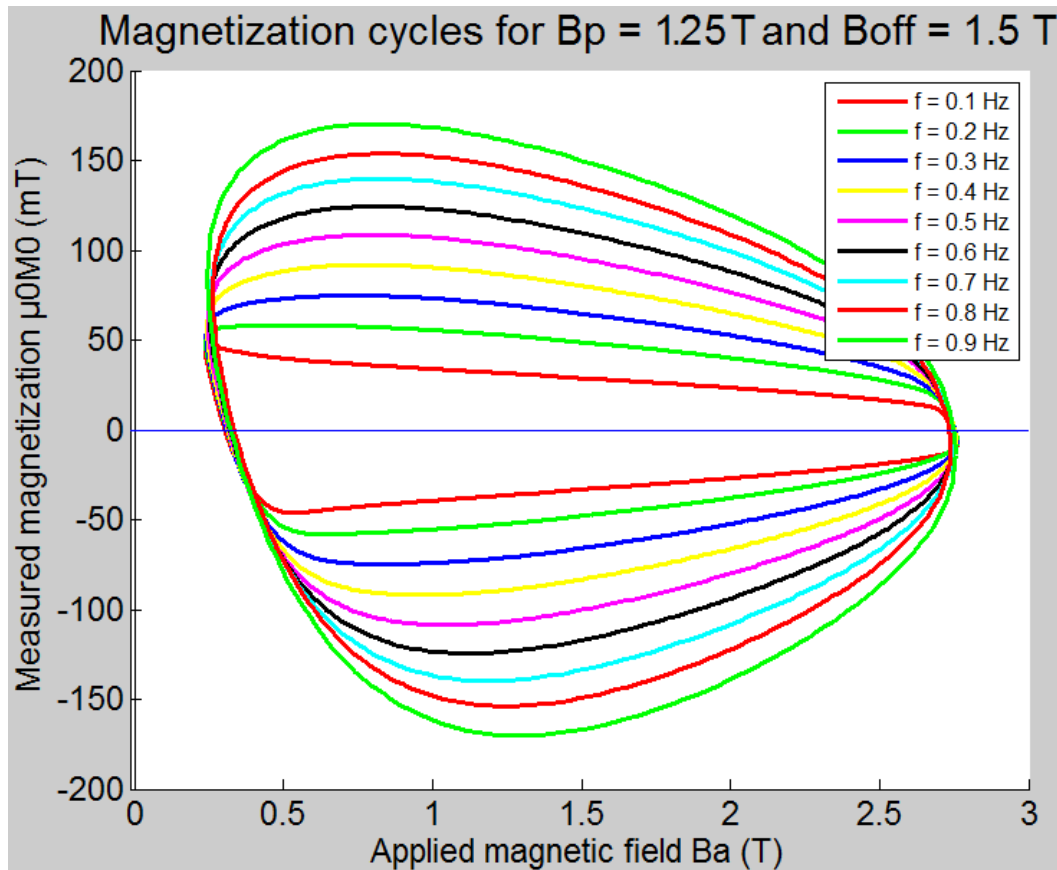
Figure 113 : Magnetization cycles of K006-01C JT-60SA TF strand measured in Speedy facility for sinusoidal cycles with B_p = 1.25\text{T} and B_{off} = 1.5\text{T}
