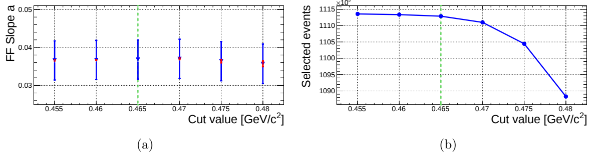
Figure 3.41: (a) Stability of the fit result and (b) number of selected events as a function of the cut value on the minimum reconstructed \pi^+\pi^0 invariant mass.
