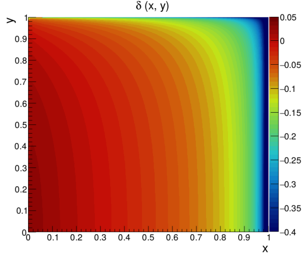
Figure 1.5: Size of the radiative corrections to the \pi_D^0 decay over the x, y plane. The magnitude of the effect goes up to 40 % of the LO decay width and has a stronger variation in the x direction.
