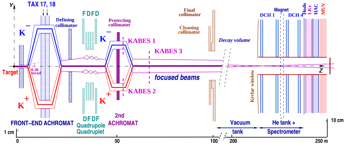
Figure 2.1: The NA48/2 beam line and detector [50].
