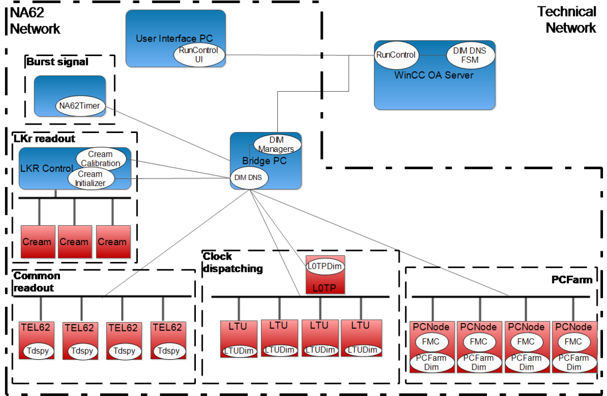
Figure 5.8: Schematic of the infrastructure of the DAQ and Run Control of the NA62 experiment. Red elements are for manipulating data. Blue elements are part of the control system of the TDAQ.
