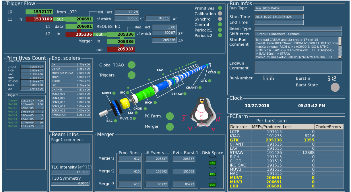
Figure 5.7: “Big Screen” of the Run Control displayed on a screen on the wall of the control room. It is the main tool reporting the status of the run, and allows quick detection of a problem in the data taking process.
