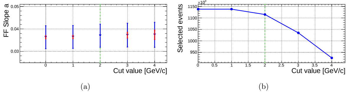
Figure 3.28: (a) Stability of the fit result and (b) number of selected events as a function of the cut value on the minimum e^\pm momentum. This cut is applied simultaneously on all tracks in the selection, but the cut value is modified only for tracks identified as e^\pm for the purpose of this scan.
