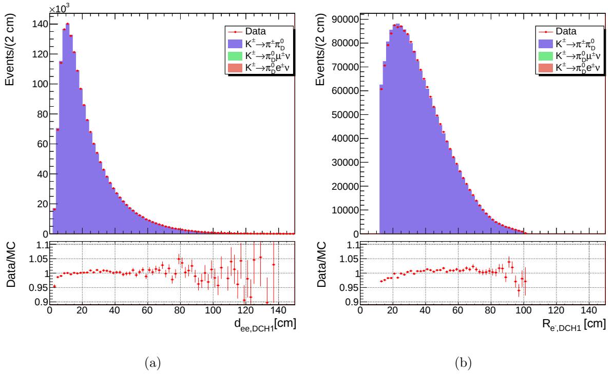
Figure 3.8: Distributions of (a) d_{ee,DCH1} and (b) R_{e-,DCH1} defined in subsection 3.5.6. The x > 0.01 cut is applied, but not the DCH acceptance cut. The deficit of data events in the lowest part of the distributions ( d_{ee,DCH1} < 10 cm and R_{e-,DCH1} < 20 cm) can be seen.
