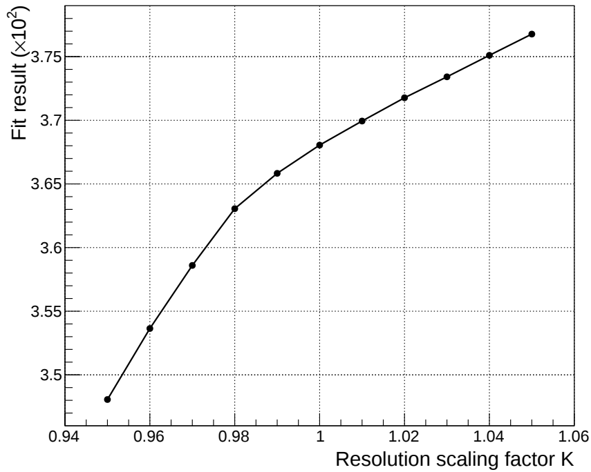
Figure 3.21: Effect of the scaling factor K on the fit result.
