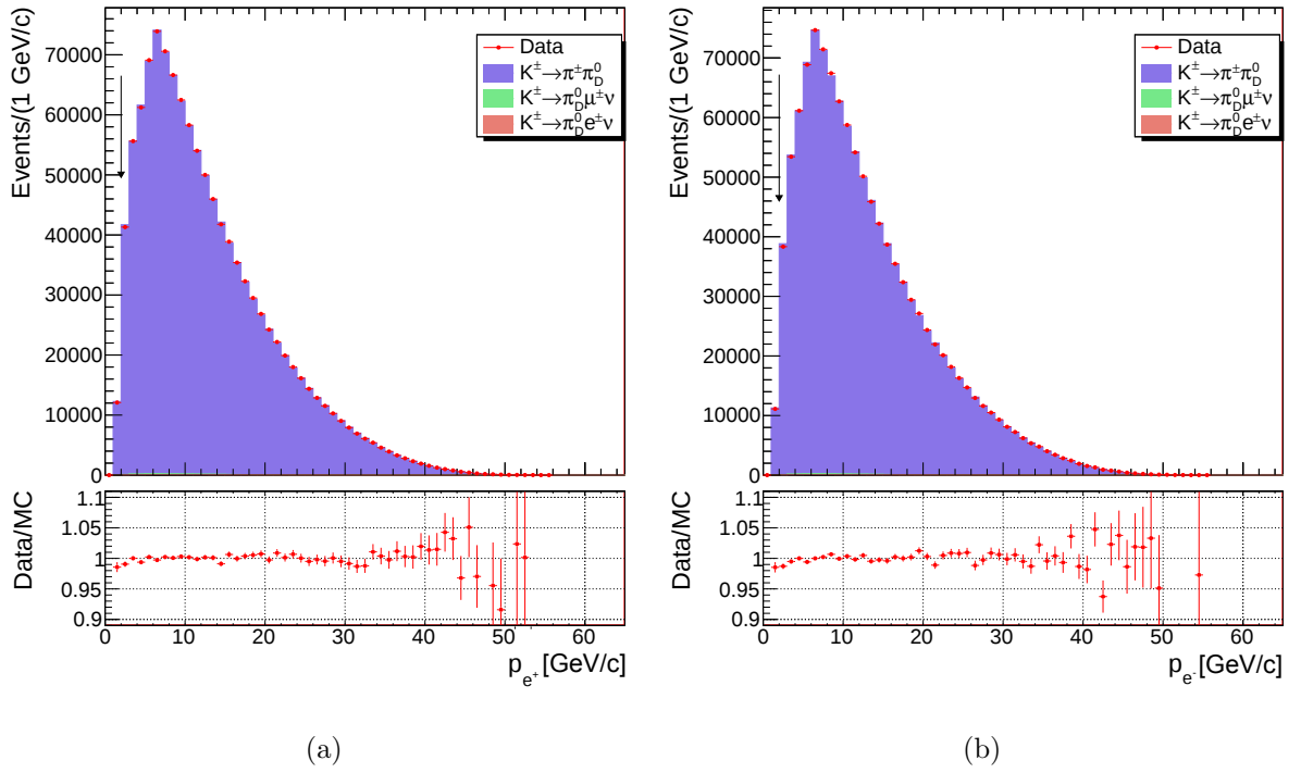
Figure 3.5: Electron (a) and positron (b) track momentum for data, MC and data/MC ratio. A 2% deficit of data is observed below 2 GeV/ c . The arrows indicate the standard value for the cut applied in the K_{2\pi D} selection.
