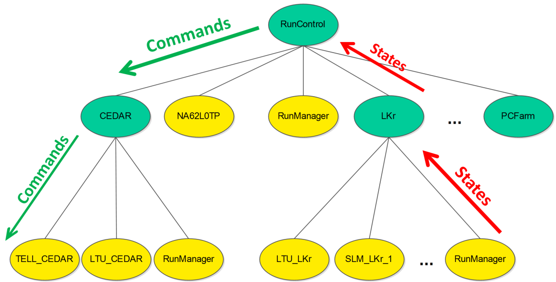
Figure 5.2: Tree-like hierarchy of units. Green units are logical units and yellow are device units. Commands are propagated downwards and states are propagated upwards and summarized in the logical units.
