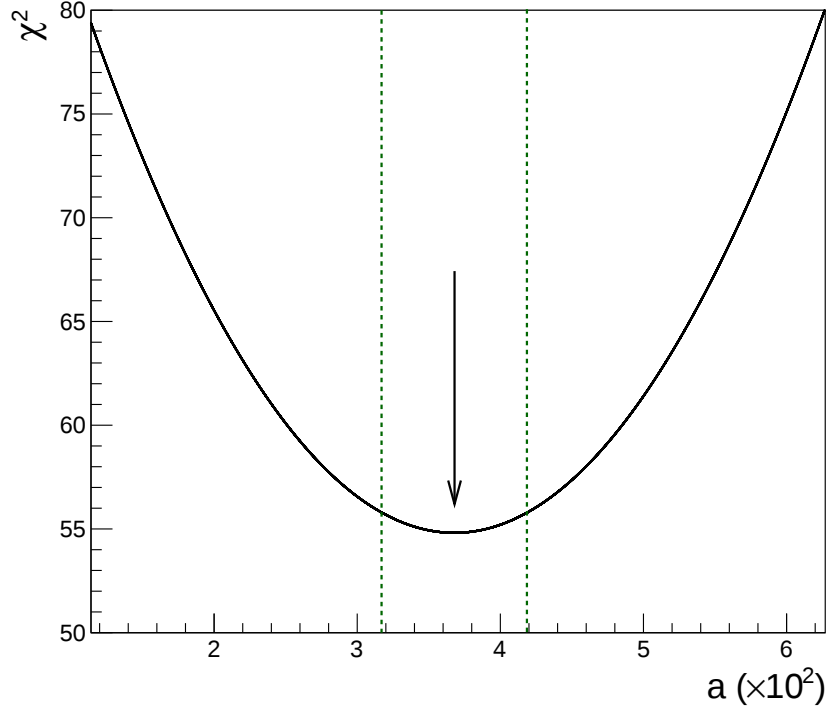
Figure 3.14: \chi^2 as a function of the TFF slope value. The number of degree of freedom (ndf) is 49. The arrow indicates the fit central value (minimum \chi^2 ), and the dashed lines represents the 1\sigma statistical uncertainty band.
